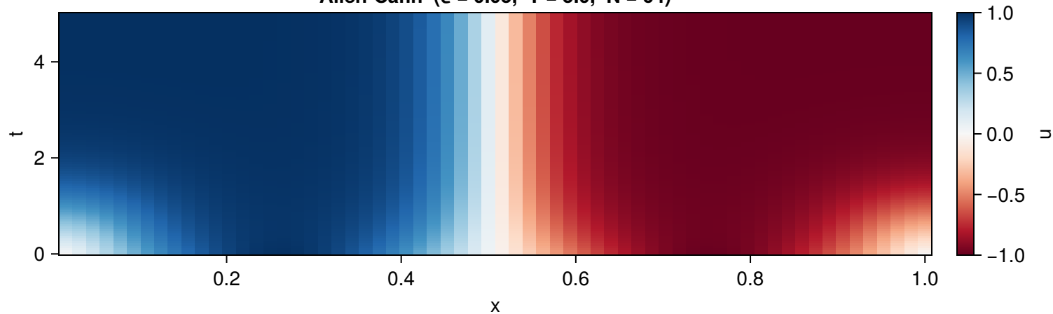
Allen-Cahn ( \epsilon = 0.05 , T = 5.0 , N = 64 )
