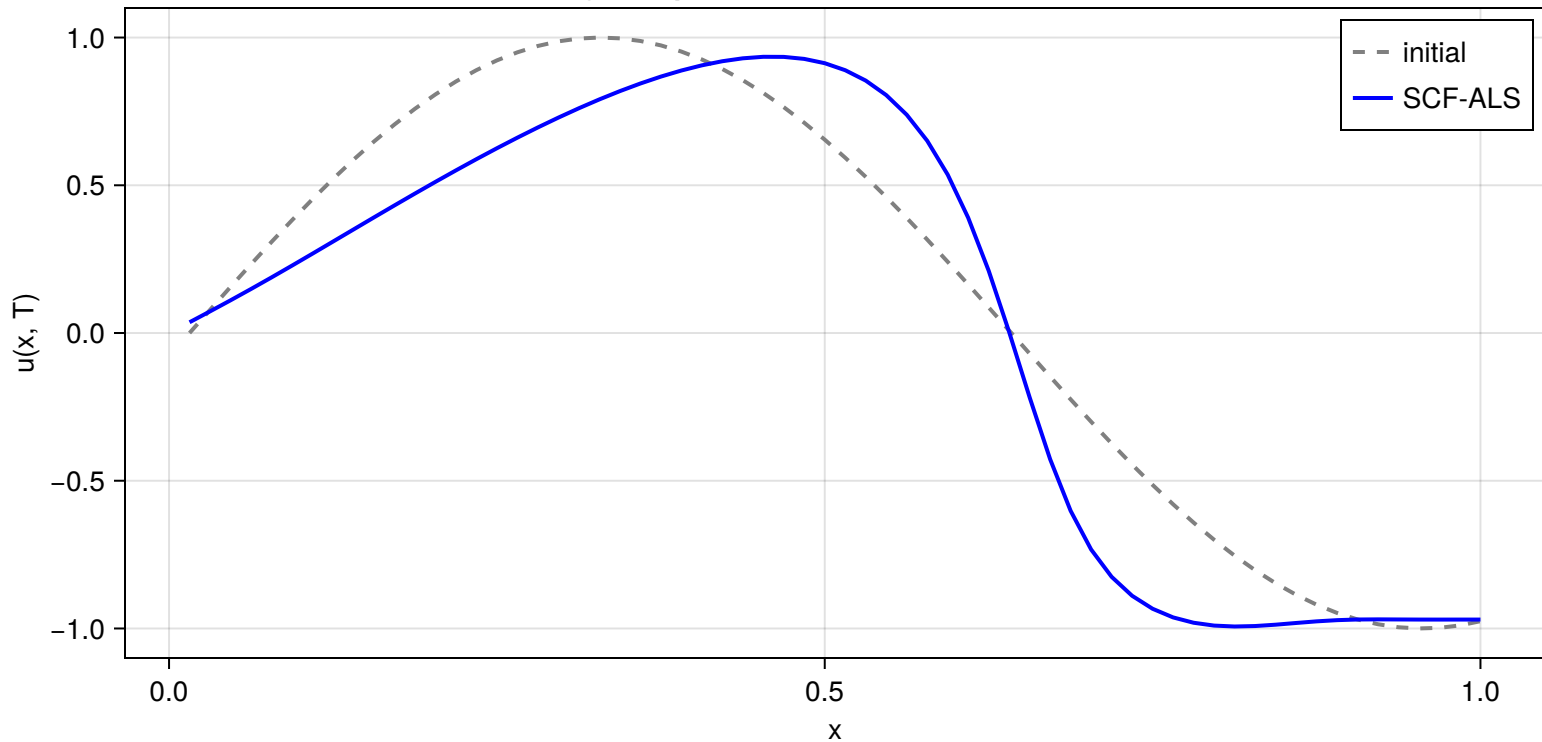
Burgers equation ( \nu = 0.01 , T = 0.15 , N = 64 )
