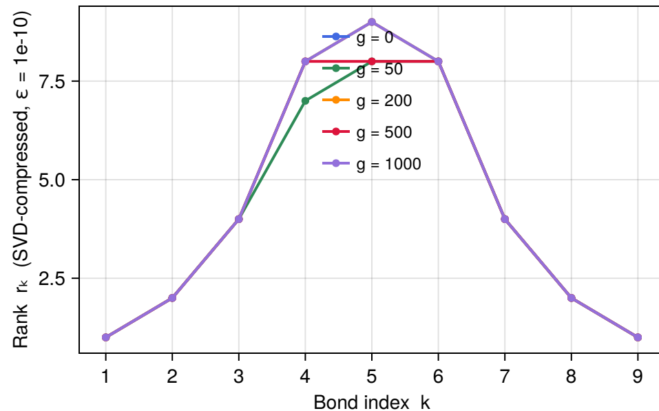
Intrinsic TT rank
