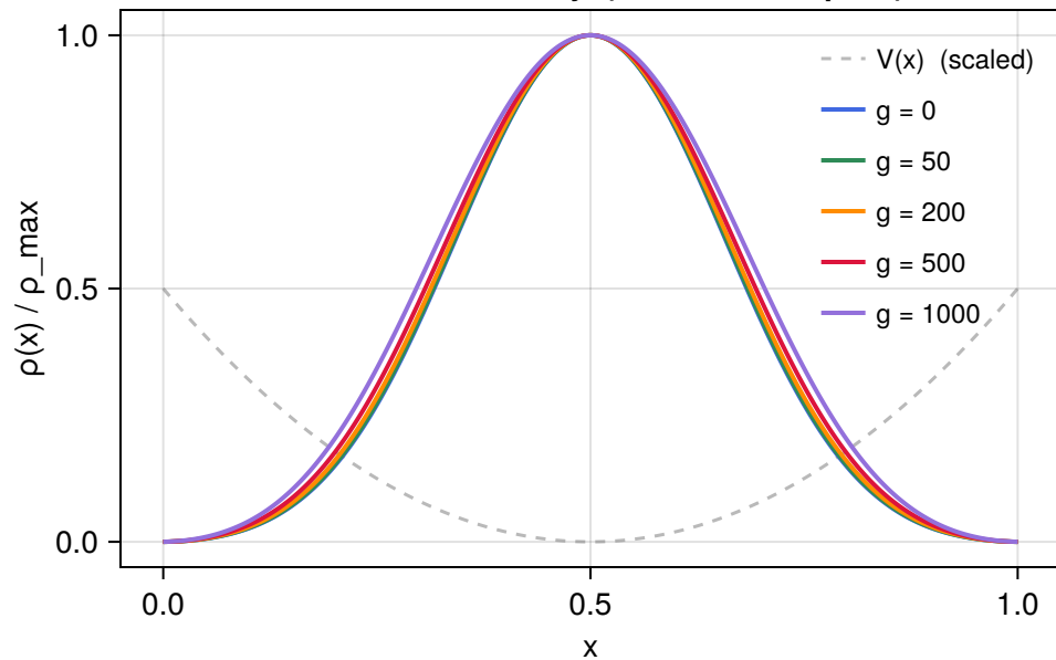
Ground-state density (normalized to peak)
