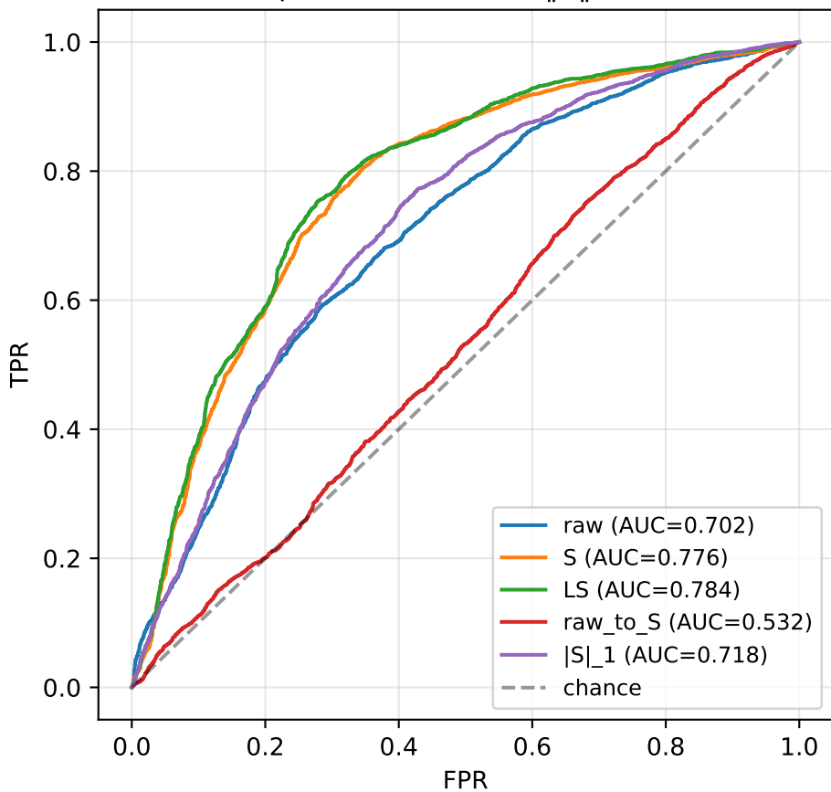
UCSDped1 — ROC with \|S\|_1 baseline
