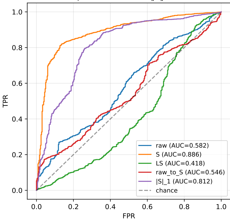
UCSDped2 — ROC with \|S\|_1 baseline
