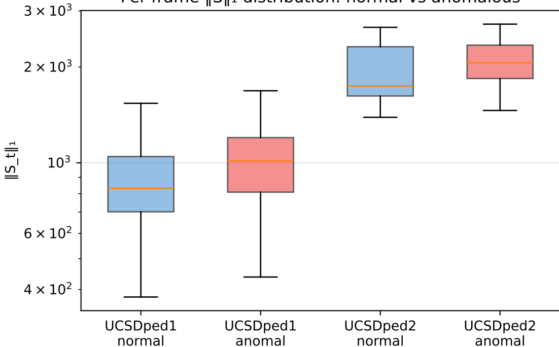
Per-frame \|S\|_1 distribution: normal vs anomalous
