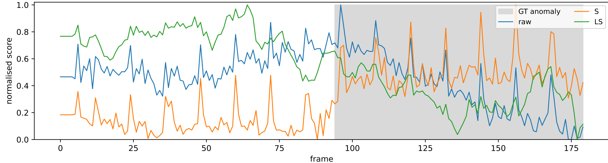
Anomaly score over time — UCSDped2/Test002
