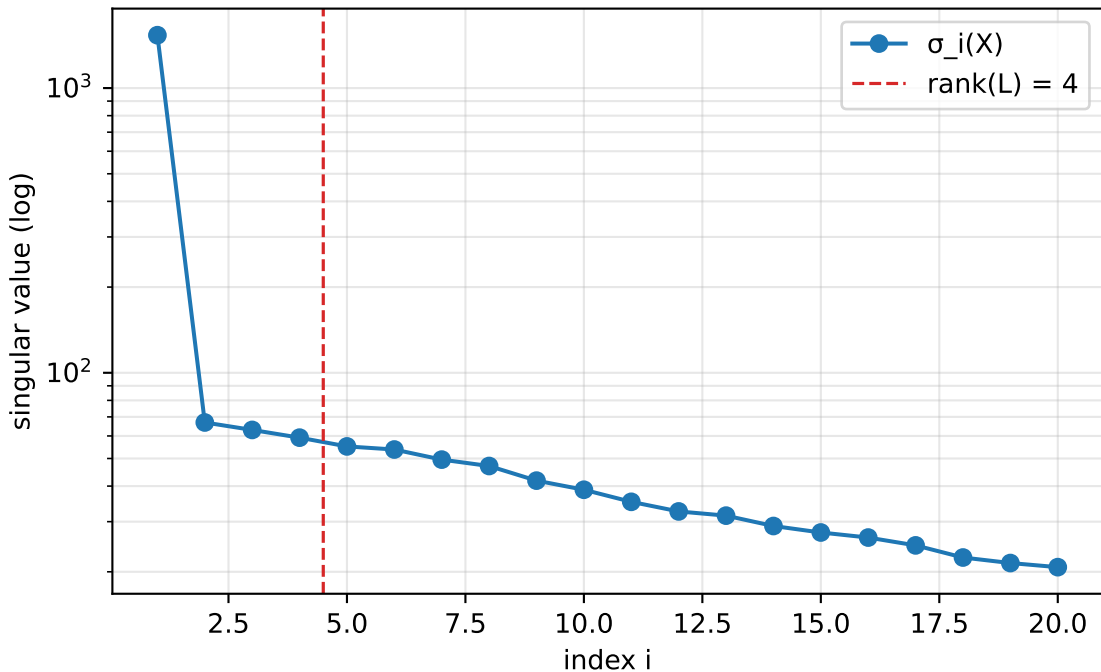
Singular spectrum of X — UCSDped2/Train/Train001
