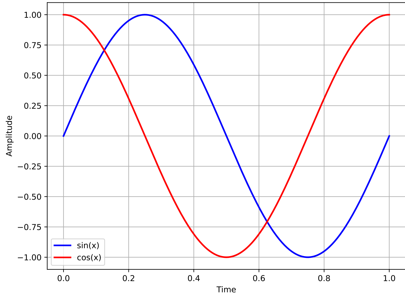
Graph of the Sine Function
