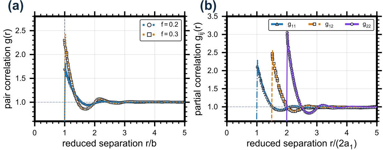
Figure 3: PackLab PY pair correlations (coloured lines) and digitised reference curves from Tsang et al. [9] (open markers). (a) Monodisperse correlations at volume fractions f = 0.2 and f = 0.3 , plotted against r/b . (b) Binary-mixture partial correlations for a_2 = 2a_1 and partial volume fractions f_1 = 0.2 , f_2 = 0.1 , plotted against r/(2a_1) .
