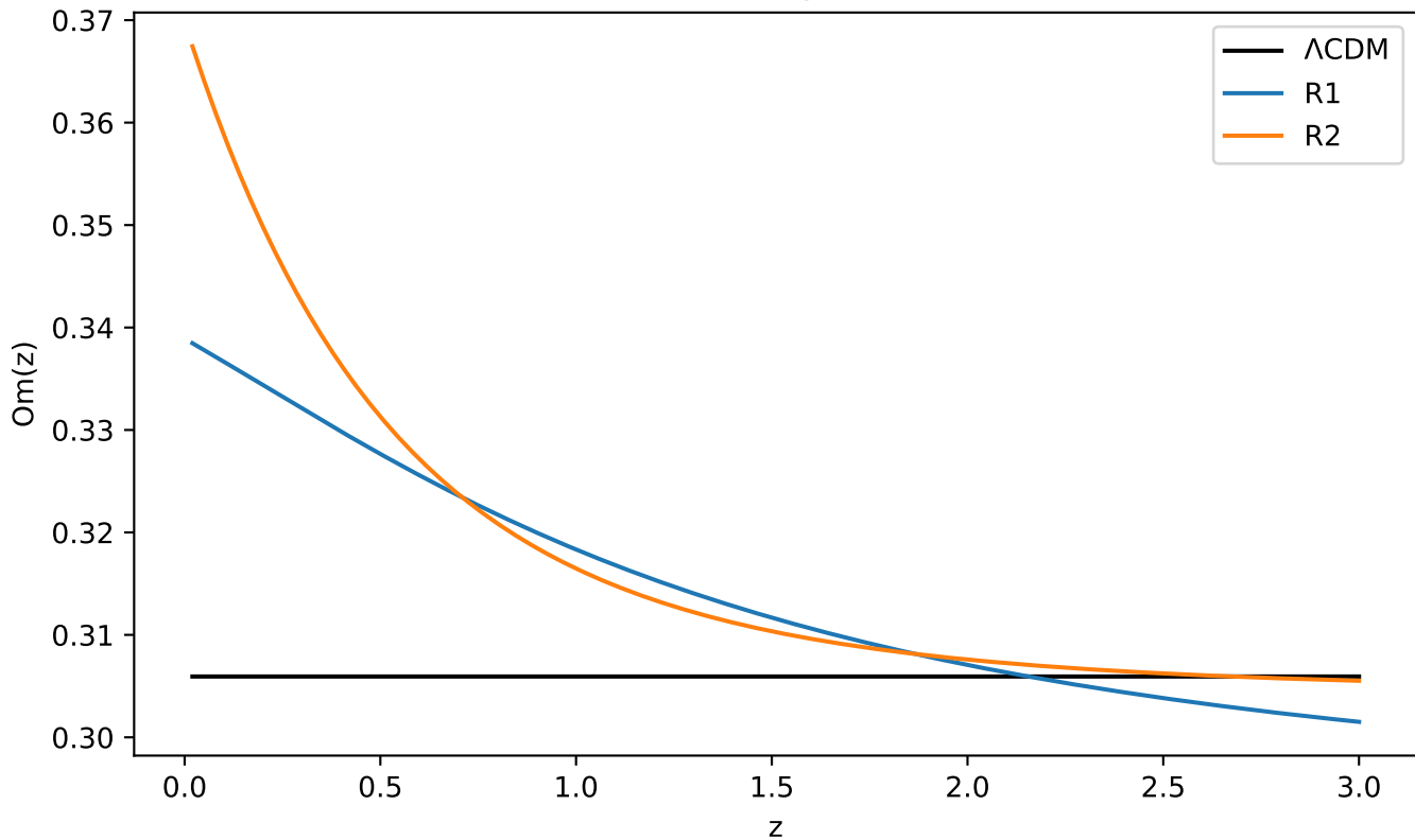
Om(z) diagnostic
