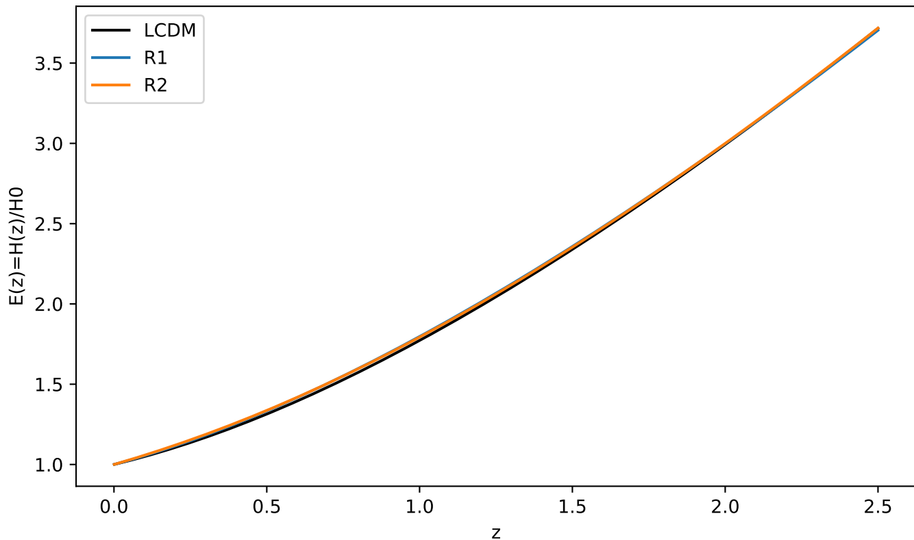
Expanzni historie pro Pantheon+ full + DESI DR2 + CC
