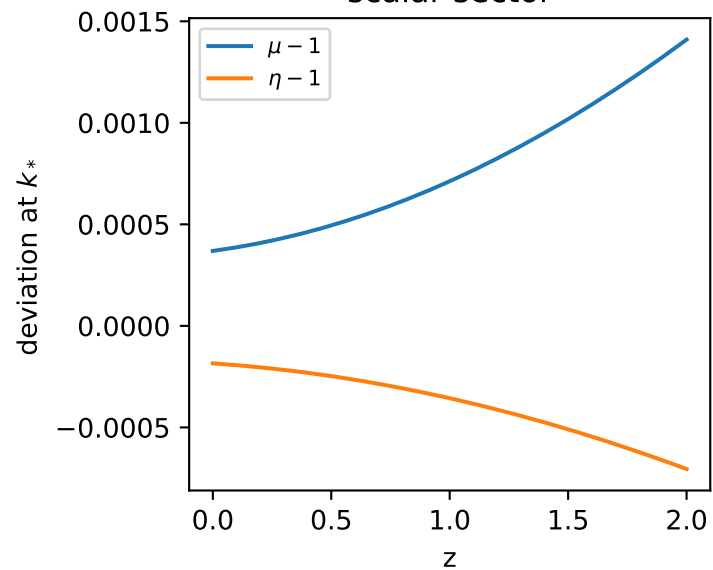
scalar sector
