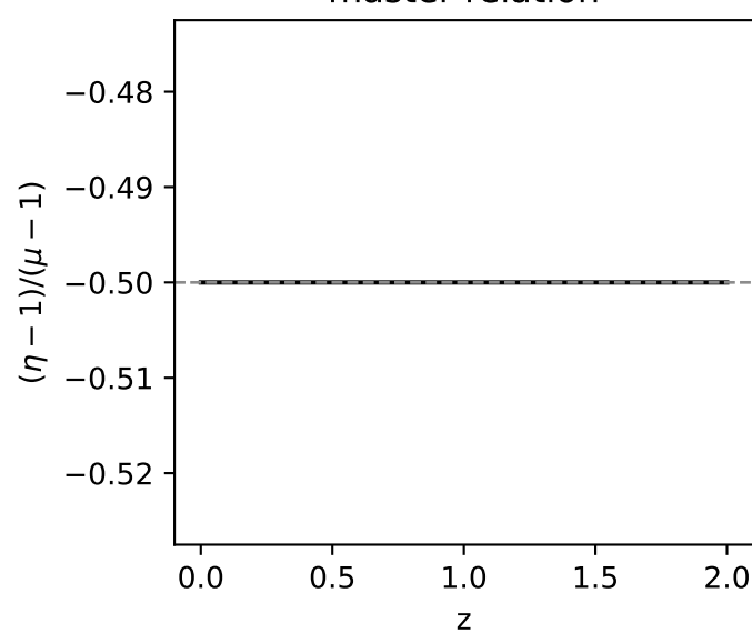
master relation
