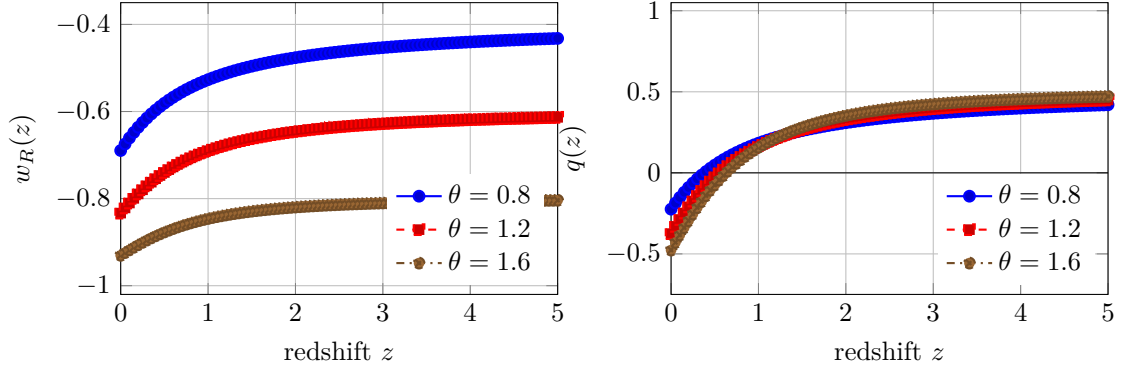
Figure 1: Cosmological dynamics evaluated from the homogeneous RFG equations and rendered from numerical coordinates embedded in this L A T E X source. The left panel shows w_R(z) , and the right panel shows q(z) , for three representative values of \theta . The acceleration transition q = 0 coincides with \Omega_R(z_{\text{acc}}) = 1/(1 + \theta) . Parameters: \Omega_{m0} = 0.3 , \Omega_{r0} = 9 \times 10^{-5} , and \Omega_{R0} = 1 - \Omega_{m0} - \Omega_{r0} .
