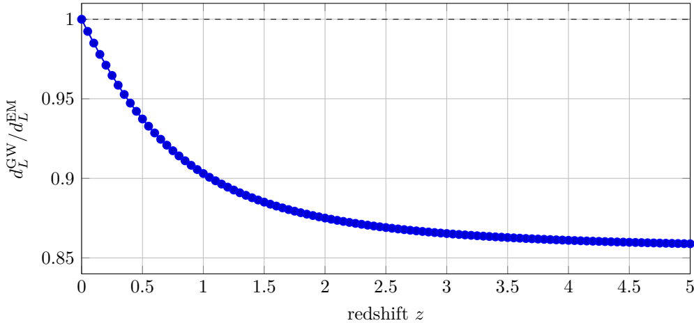
Figure 2: Standard-siren prediction evaluated from Eq. (25) on the homogeneous RFG background and rendered from numerical coordinates embedded in this \text{\LaTeX} source, for \Omega_{R0} = 0.70 and \theta = 1.6 . The ratio equals unity at z = 0 , is approximately 0.903 at z = 1 , and approaches \sqrt{Q_T(0)} \approx 0.855 at high redshift. No illustrative observational point is added, because a statistically meaningful comparison requires an explicit likelihood analysis.
