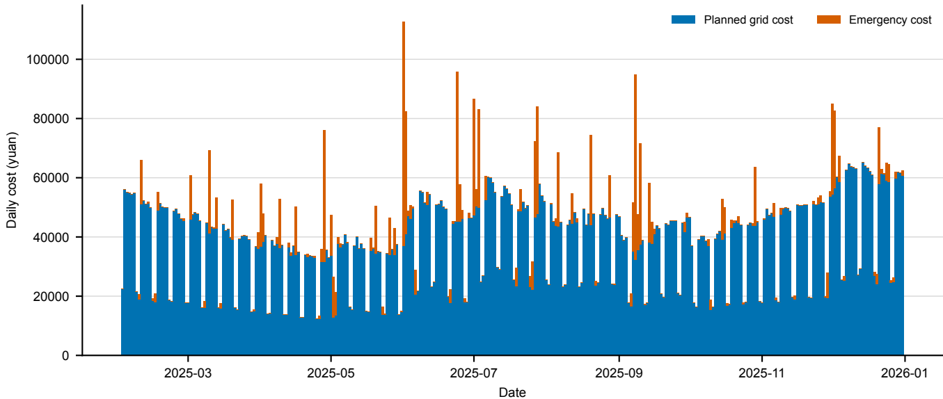
Daily cost components under dynamic dispatch
