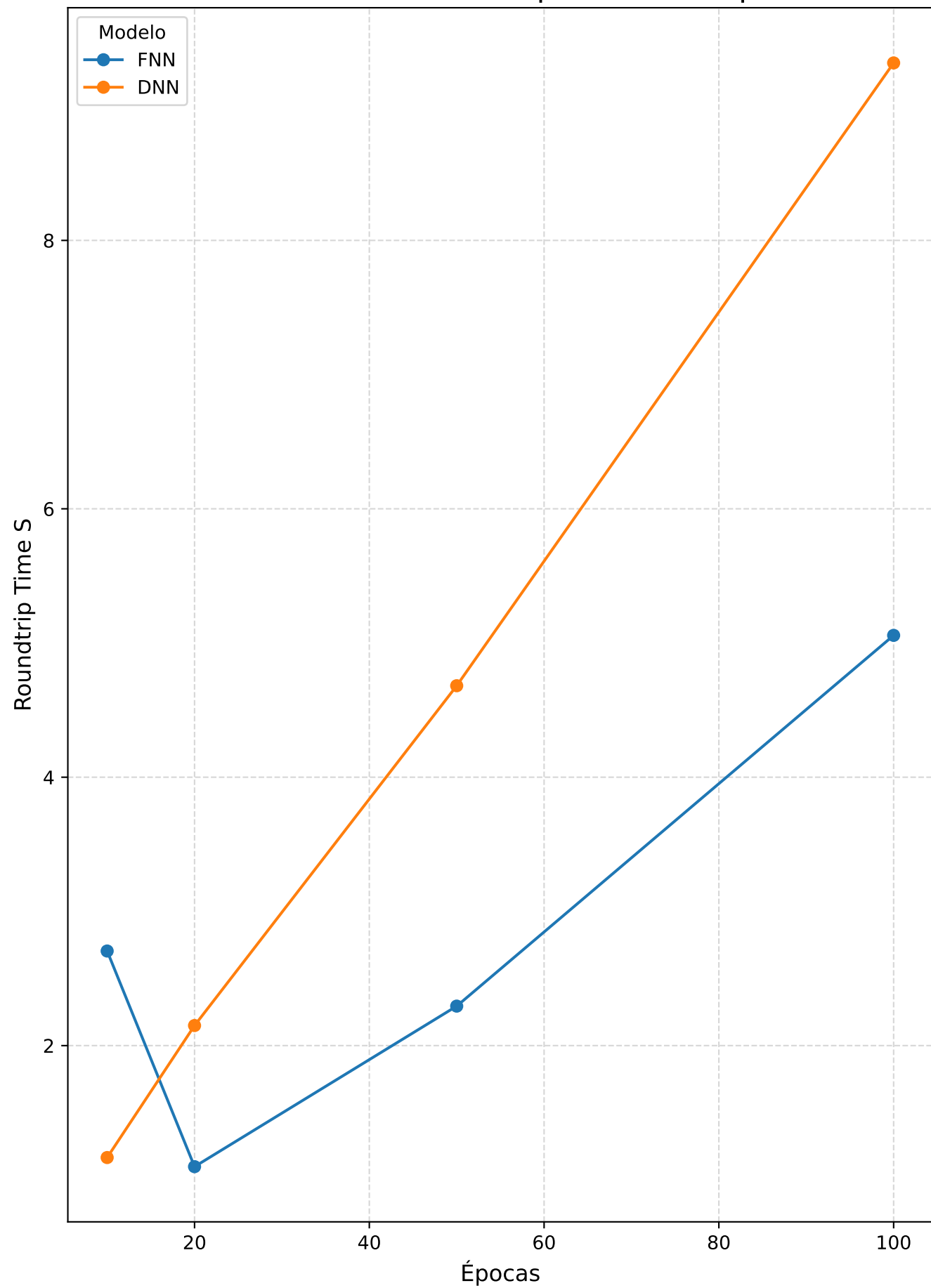
Classification • Roundtrip Time S vs Épocas
