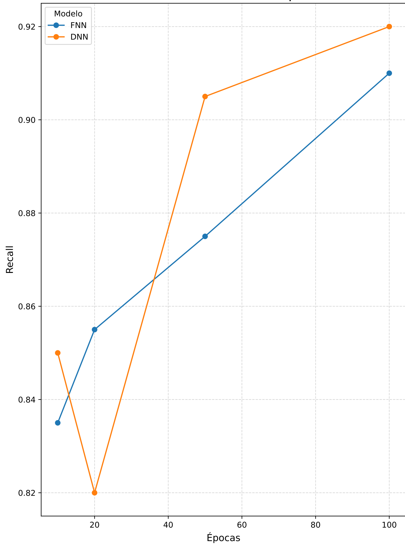
Classification • Recall vs Épocas
