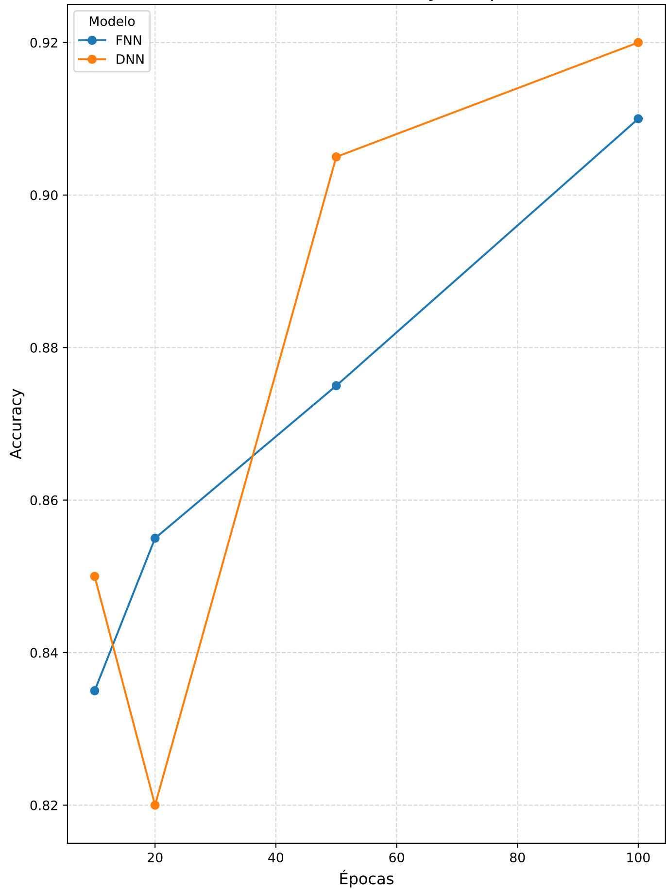
Classification • Accuracy vs Épocas
