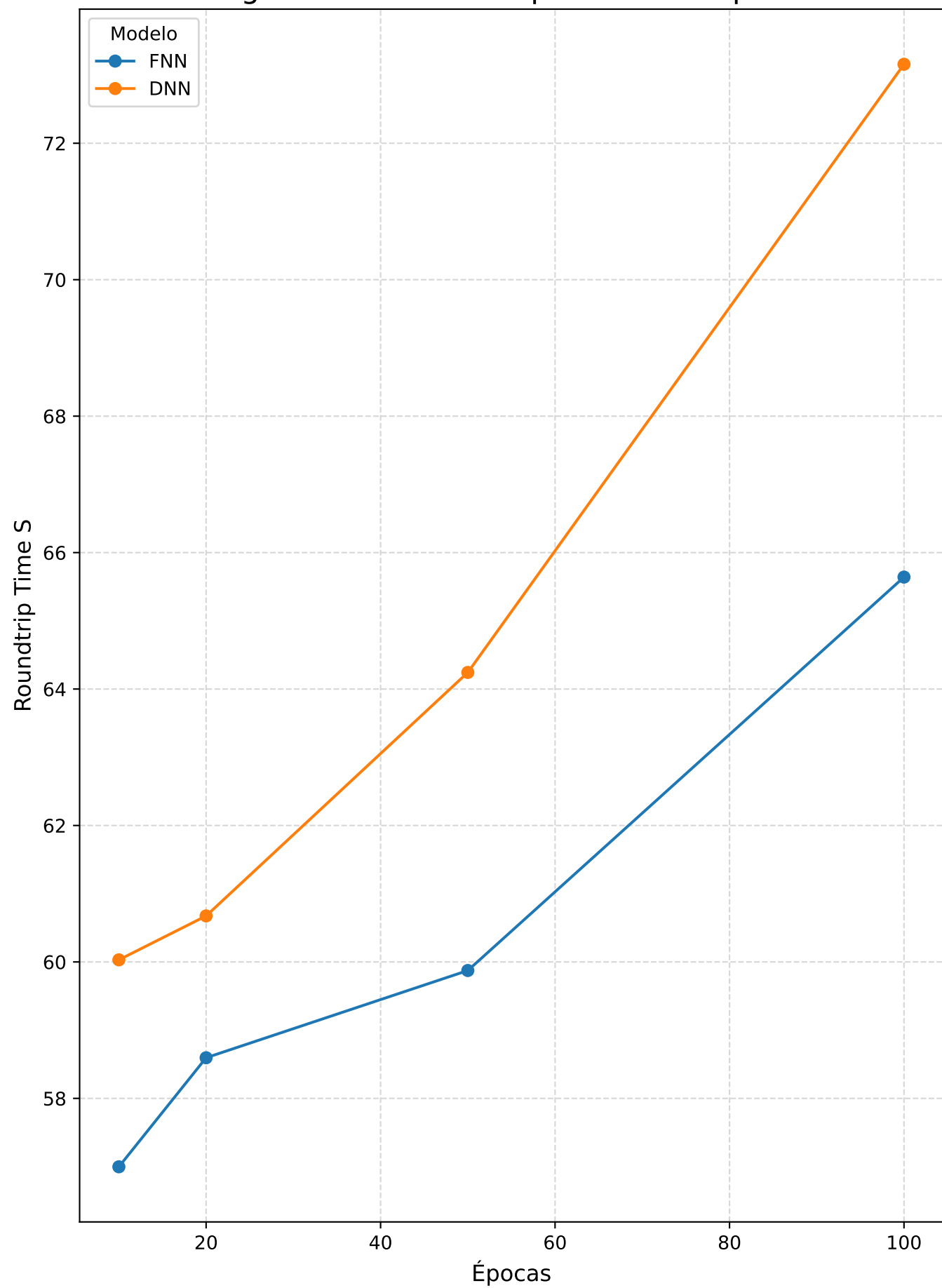
Regression • Roundtrip Time S vs Épocas
