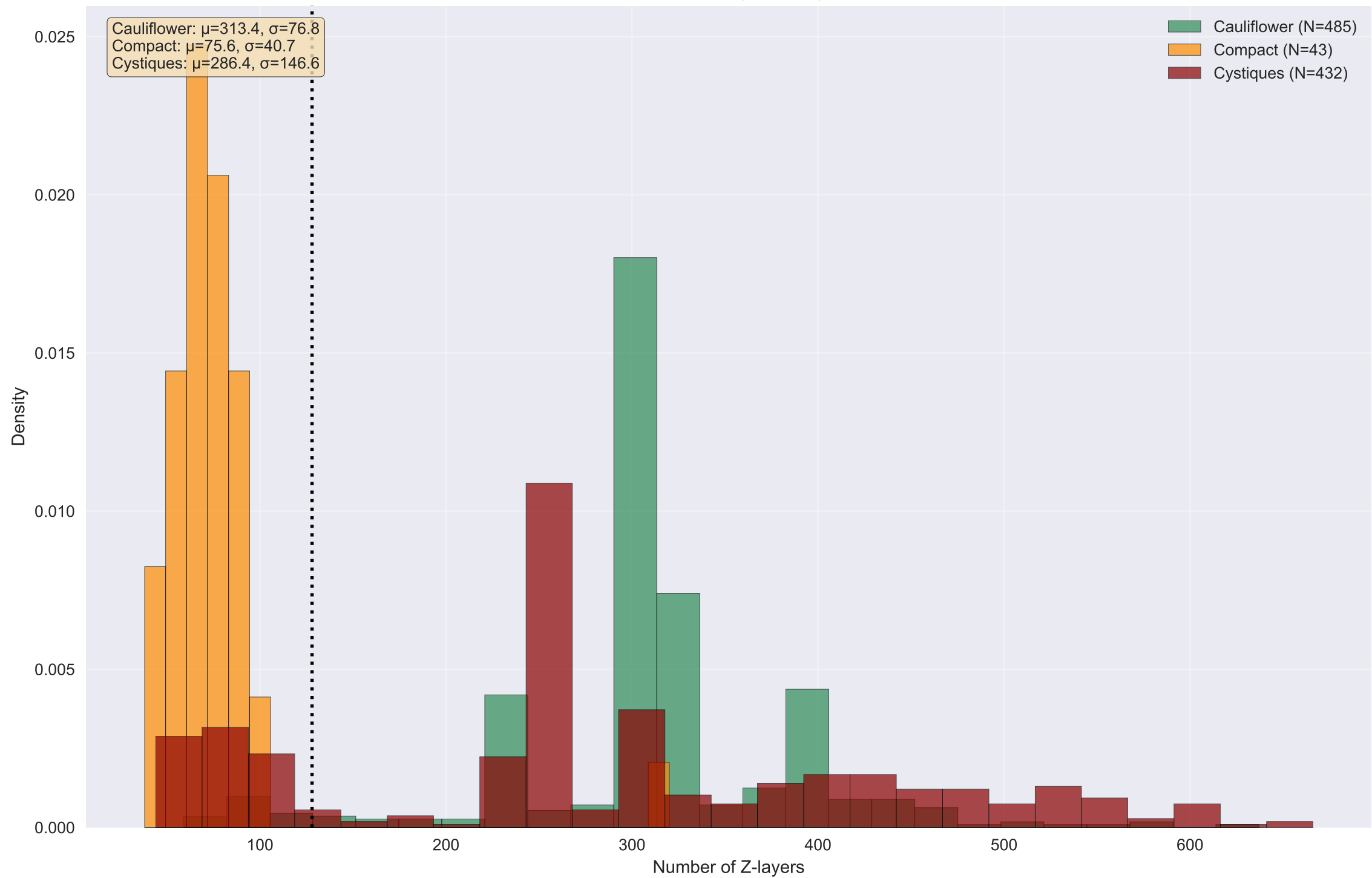
Z-Depth Distribution by Phenotypic Class
