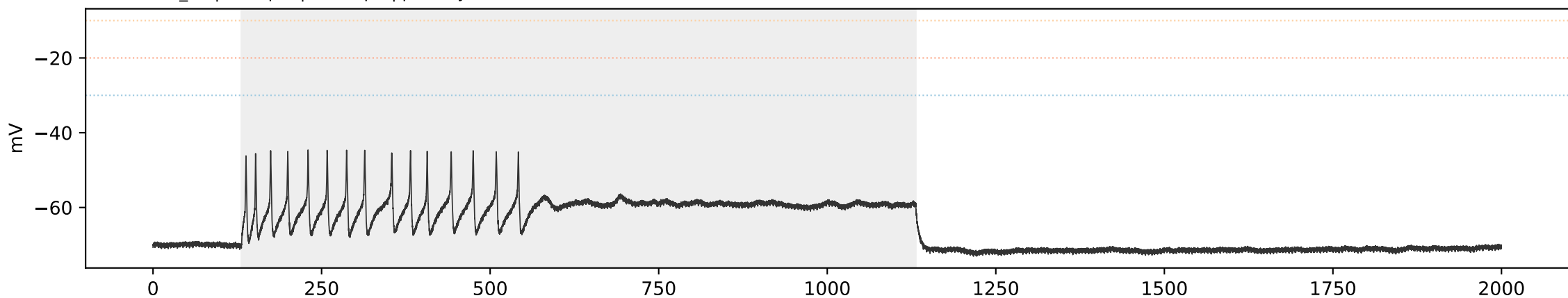
SCA3 SCA3_02 | sweep 6 | 300.0 pA | primary=0, strict=0
