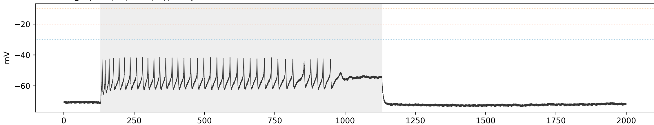
SCA3 SCA3_02 | sweep 9 | 450.0 pA | primary=0, strict=0
