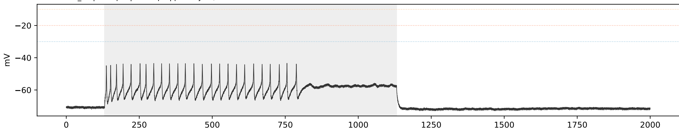
SCA3 SCA3_02 | sweep 7 | 350.0 pA | primary=0, strict=0
