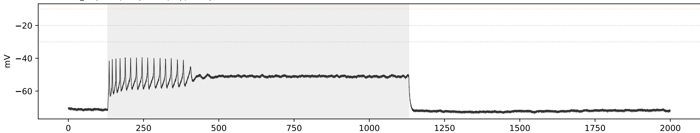
SCA3 SCA3_02 | sweep 11 | 550.0 pA | primary=0, strict=0
