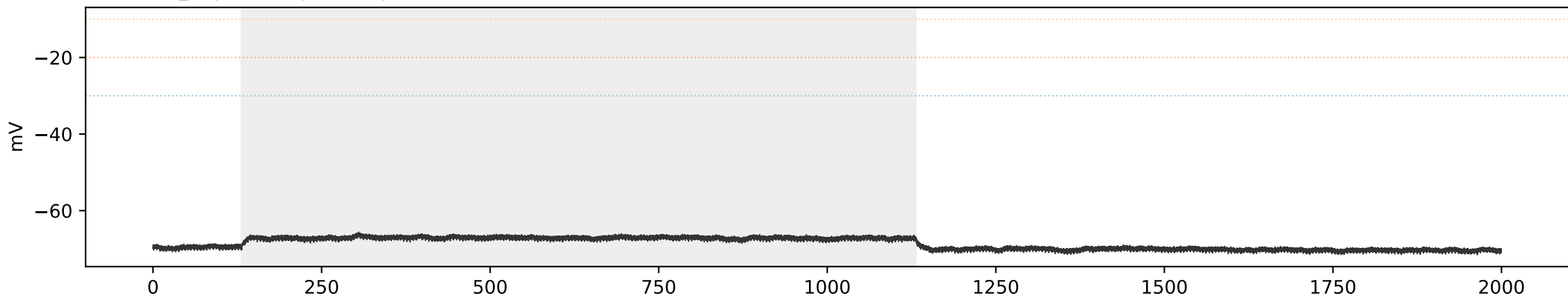
SCA3 SCA3_02 | sweep 2 | 100.0 pA | primary=0, strict=0
