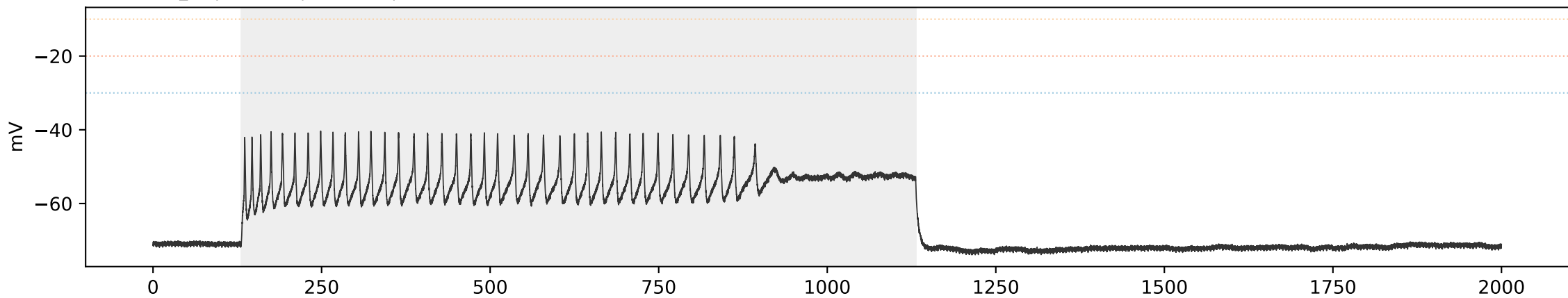
SCA3 SCA3_02 | sweep 10 | 500.0 pA | primary=0, strict=0
