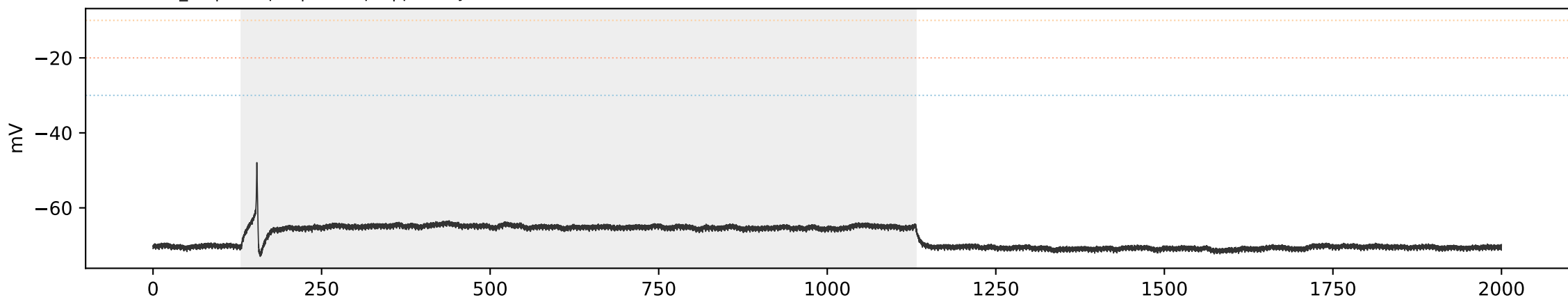
SCA3 SCA3_02 | sweep 3 | 150.0 pA | primary=0, strict=0
