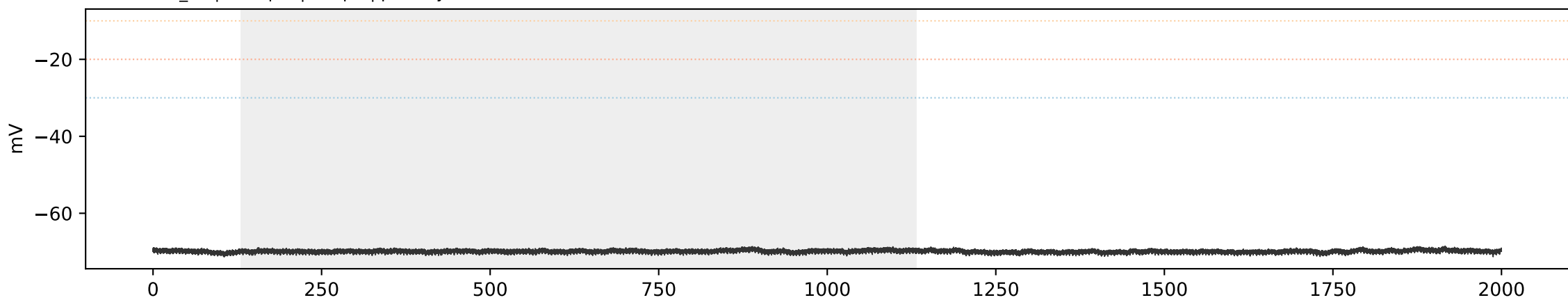
SCA3 SCA3_02 | sweep 1 | 50.0 pA | primary=0, strict=0
