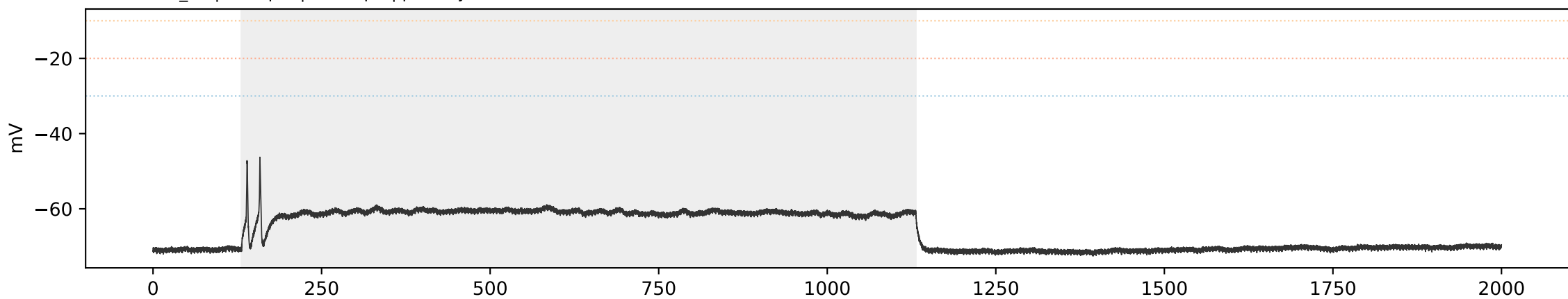
SCA3 SCA3_02 | sweep 5 | 250.0 pA | primary=0, strict=0
