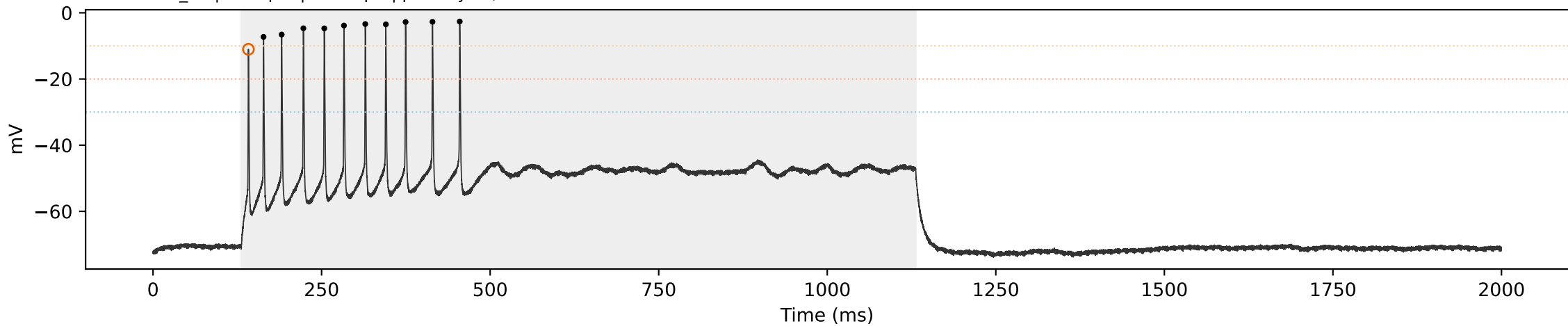
SCA3 SCA3_05 | sweep 7 | 350.0 pA | primary=0, strict=0
