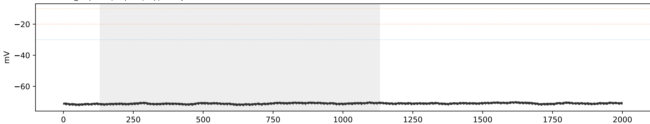
SCA3 SCA3_05 | sweep 1 | 50.0 pA | primary=0, strict=0
