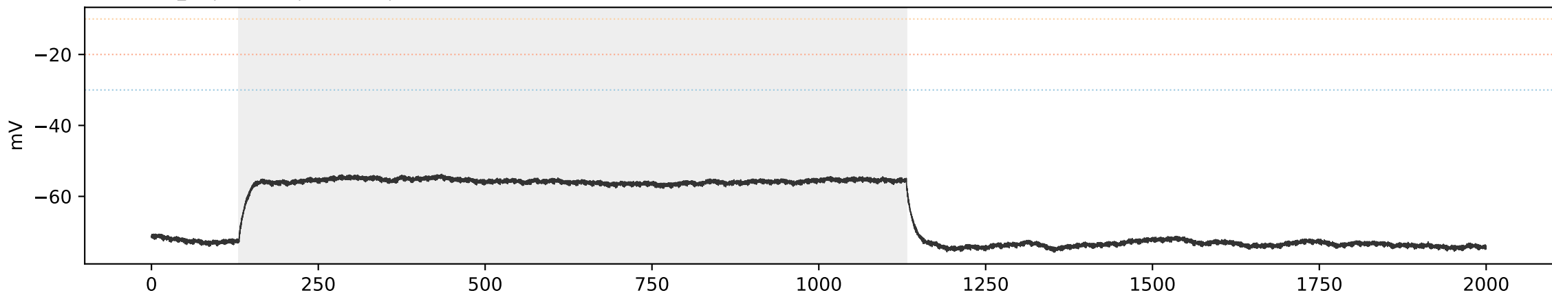
SCA3 SCA3_05 | sweep 6 | 300.0 pA | primary=0, strict=0
