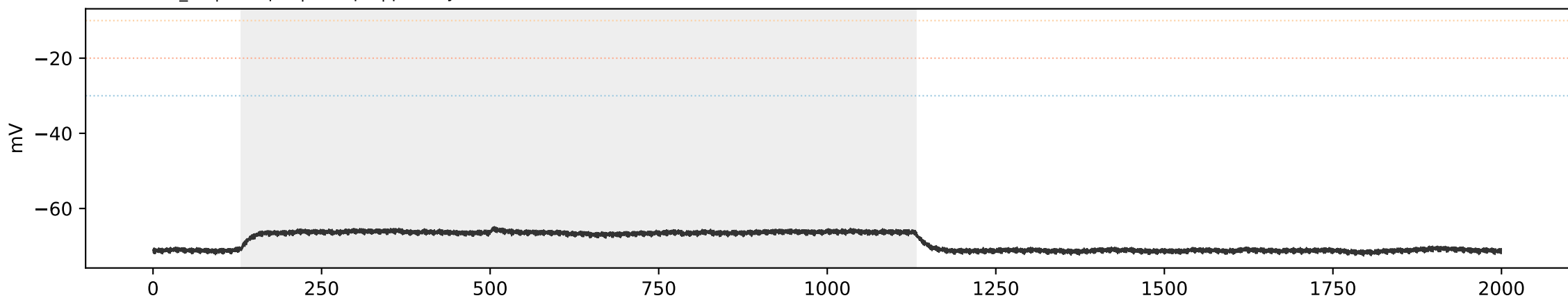
SCA3 SCA3_05 | sweep 2 | 100.0 pA | primary=0, strict=0
