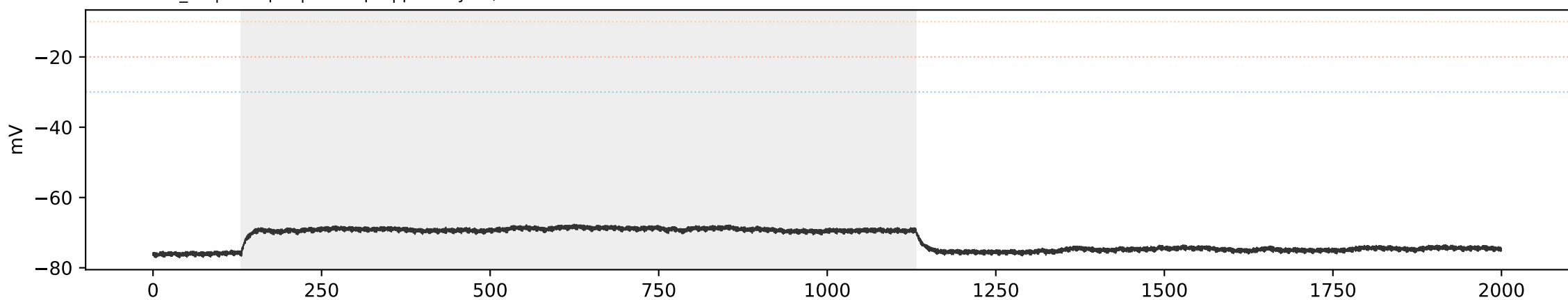
SCA3 SCA3_05 | sweep 3 | 150.0 pA | primary=0, strict=0
