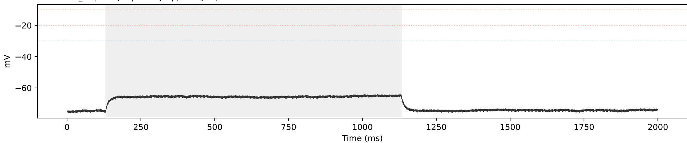
SCA3 SCA3_05 | sweep 3 | 150.0 pA | primary=0, strict=0
