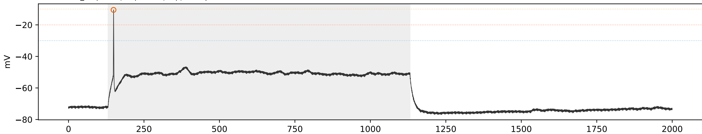
SCA3 SCA3_05 | sweep 7 | 350.0 pA | primary=0, strict=0
