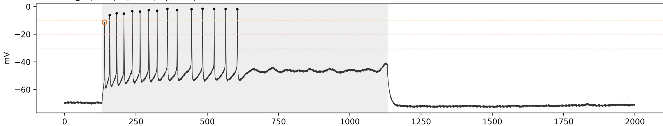
SCA3 SCA3_05 | sweep 9 | 450.0 pA | primary=2, strict=2
