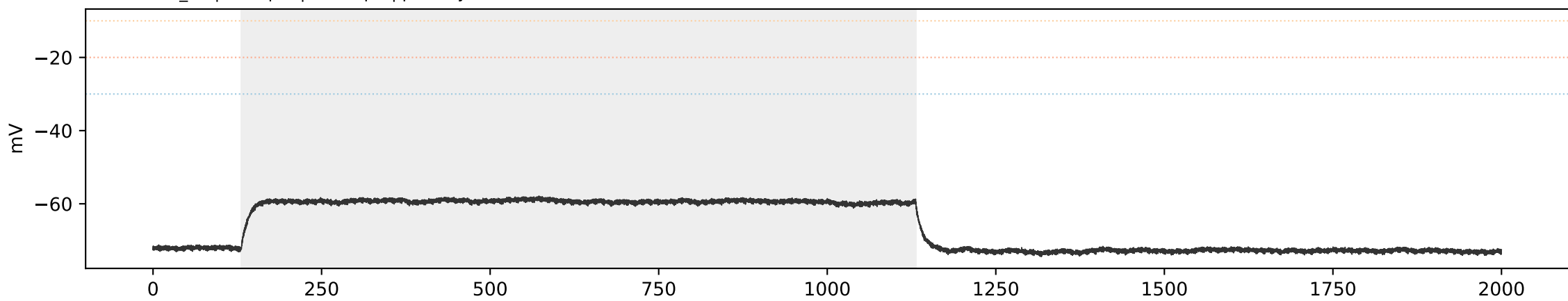
SCA3 SCA3_05 | sweep 5 | 250.0 pA | primary=0, strict=0
