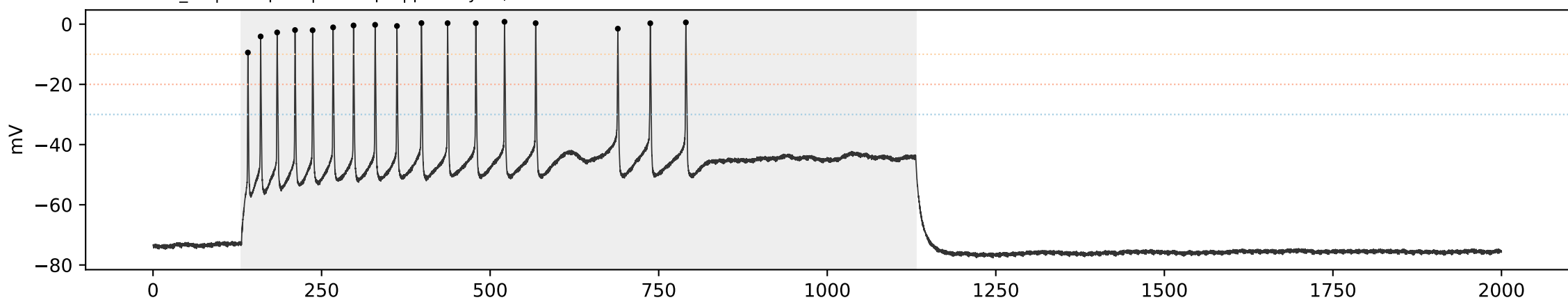
SCA3 SCA3_05 | sweep 11 | 550.0 pA | primary=2, strict=2
