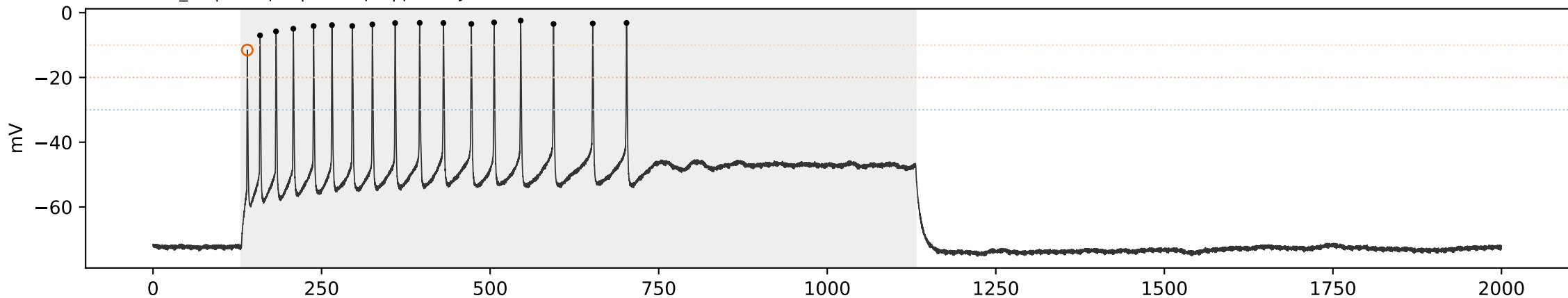
SCA3 SCA3_05 | sweep 10 | 500.0 pA | primary=3, strict=3
