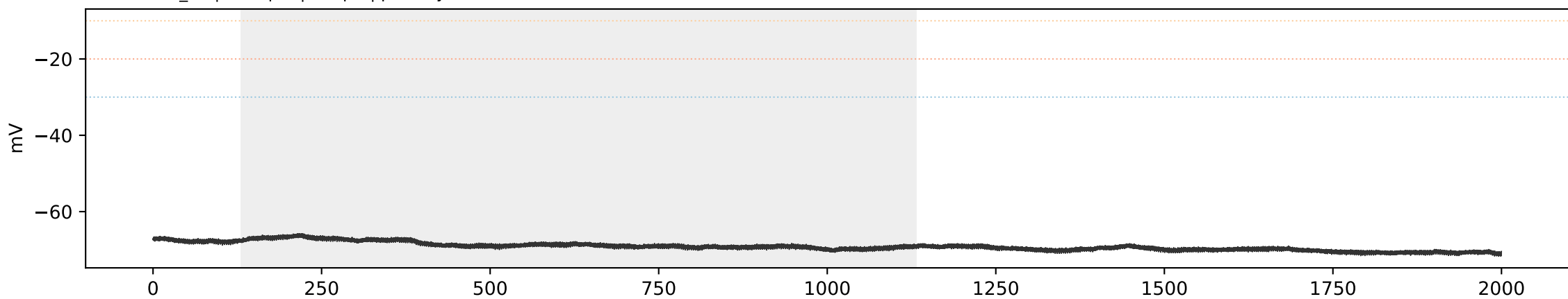
SCA3 SCA3_09 | sweep 1 | 50.0 pA | primary=0, strict=0
