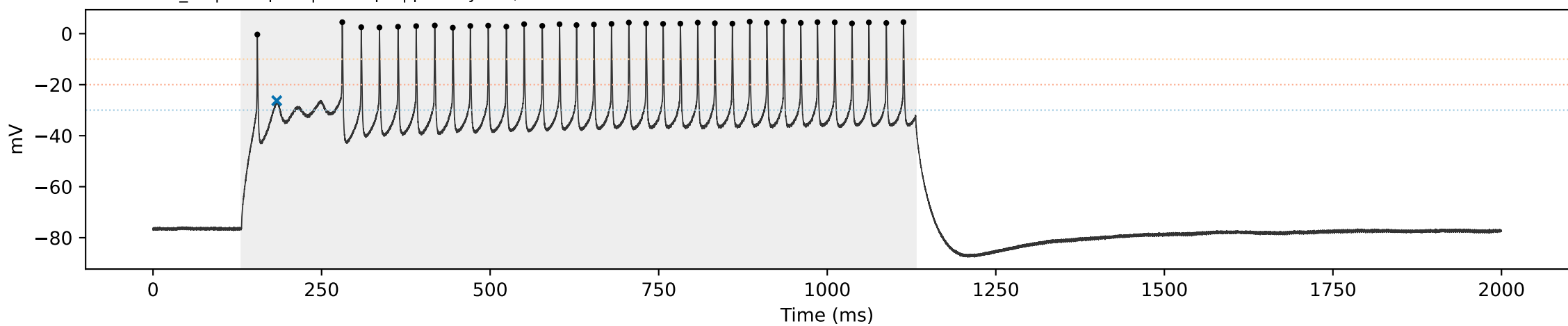
SCA3 SCA3_09 | sweep 11 | 550.0 pA | primary=21, strict=21
