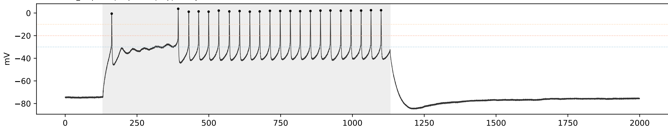
SCA3 SCA3_09 | sweep 10 | 500.0 pA | primary=18, strict=18
