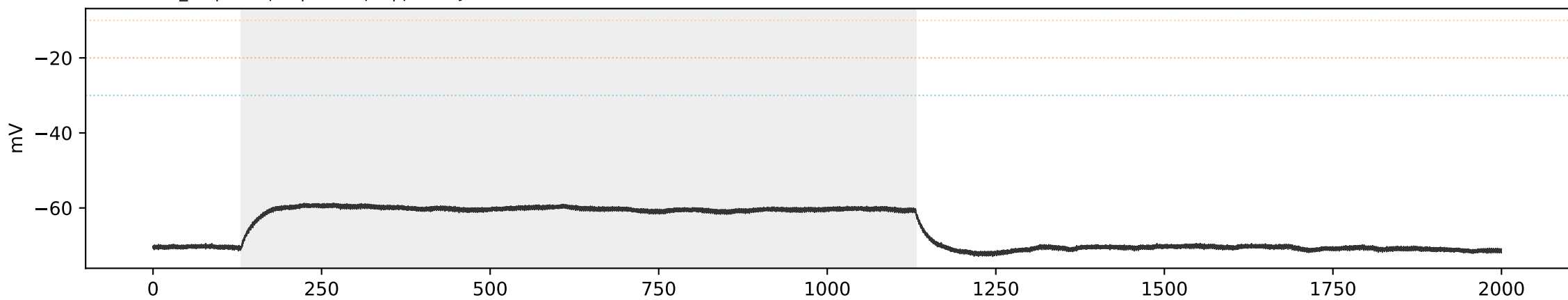
SCA3 SCA3_09 | sweep 3 | 150.0 pA | primary=0, strict=0
