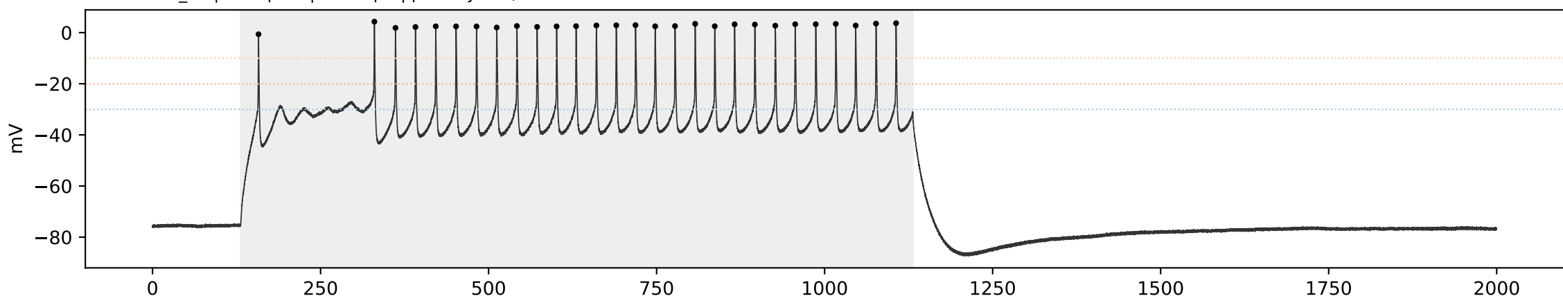
SCA3 SCA3_09 | sweep 11 | 550.0 pA | primary=21, strict=21
