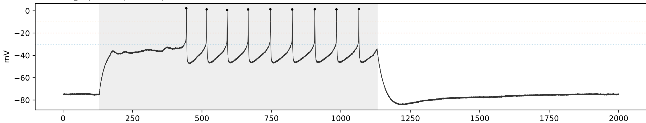
SCA3 SCA3_09 | sweep 7 | 350.0 pA | primary=6, strict=6
