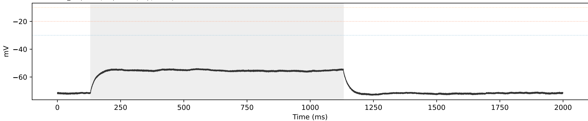
SCA3 SCA3_09 | sweep 3 | 150.0 pA | primary=0, strict=0
