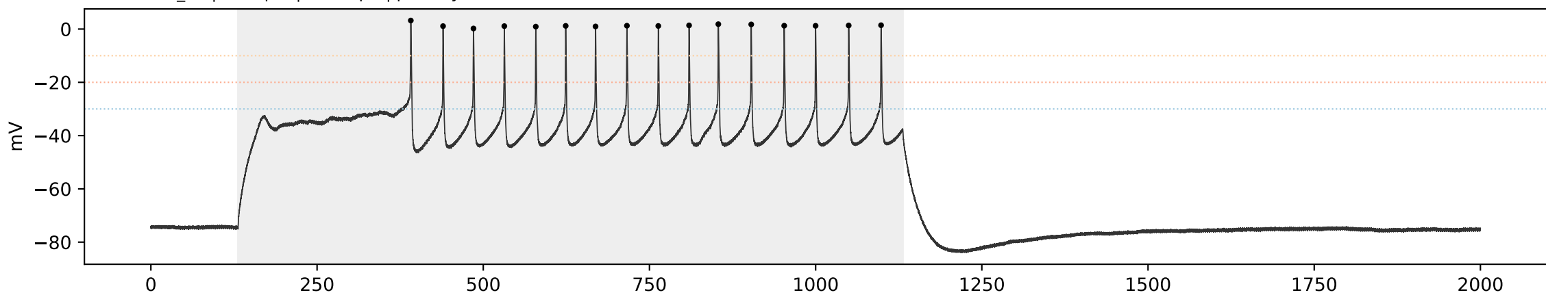
SCA3 SCA3_09 | sweep 9 | 450.0 pA | primary=15, strict=15
