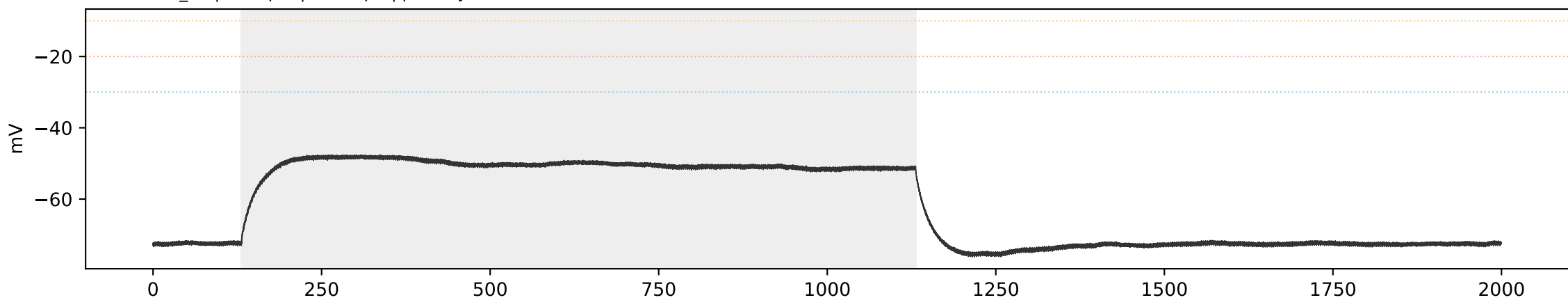
SCA3 SCA3_09 | sweep 5 | 250.0 pA | primary=0, strict=0
