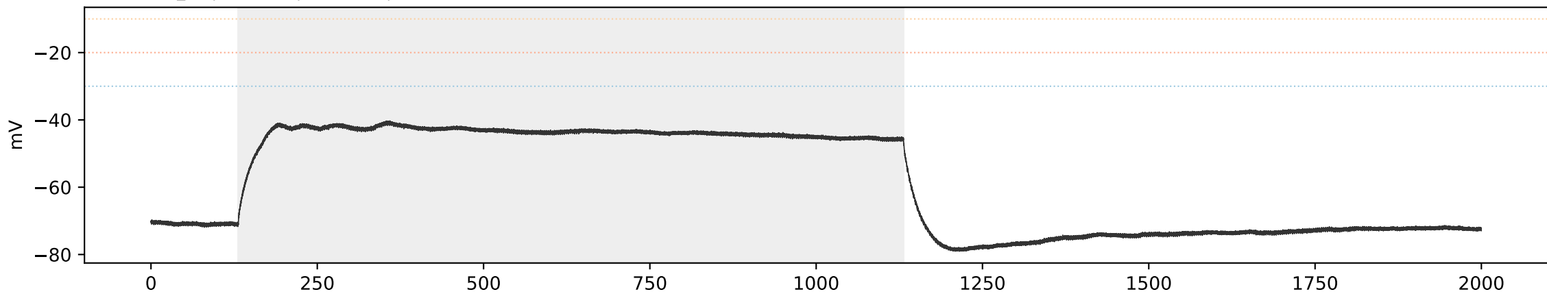
SCA3 SCA3_09 | sweep 6 | 300.0 pA | primary=4, strict=4
