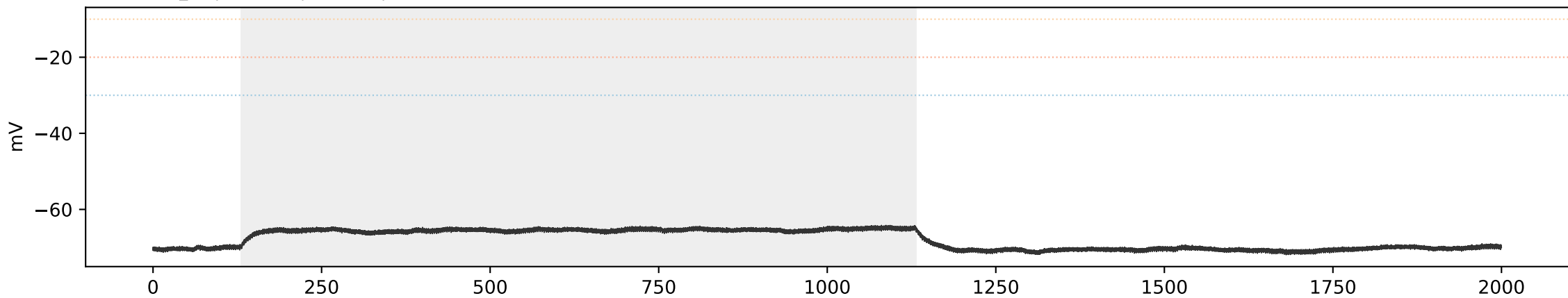
SCA3 SCA3_09 | sweep 2 | 100.0 pA | primary=0, strict=0
