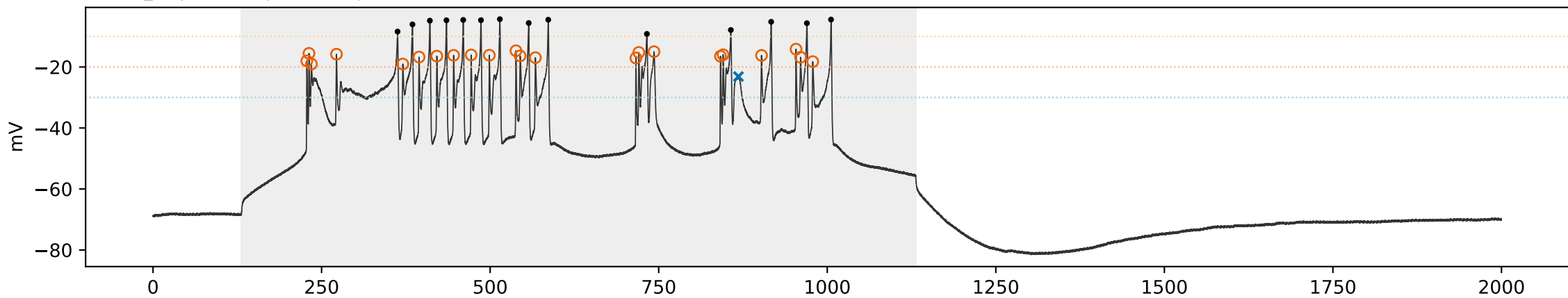
WT WT_02 | sweep 6 | 300.0 pA | primary=4, strict=2
