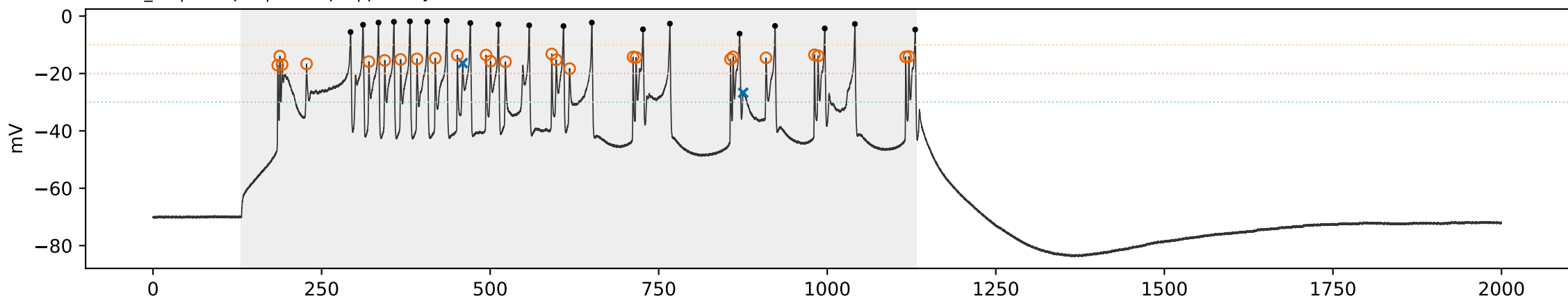
WT WT_02 | sweep 9 | 450.0 pA | primary=18, strict=9
