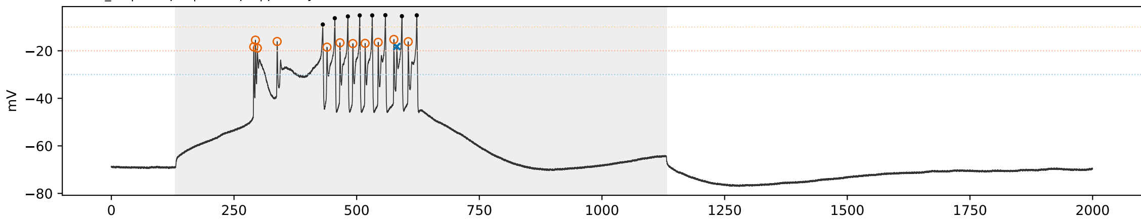
WT WT_02 | sweep 5 | 250.0 pA | primary=14, strict=5
