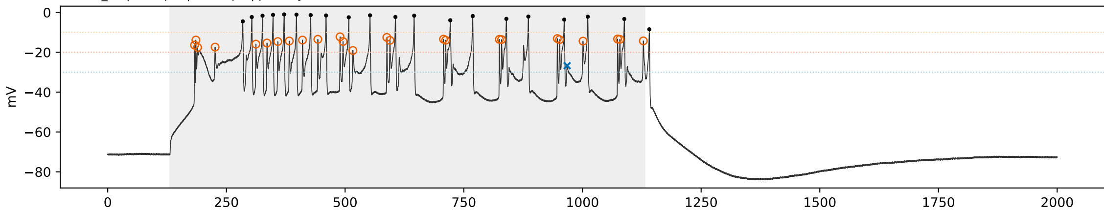
WT WT_02 | sweep 10 | 500.0 pA | primary=22, strict=9
