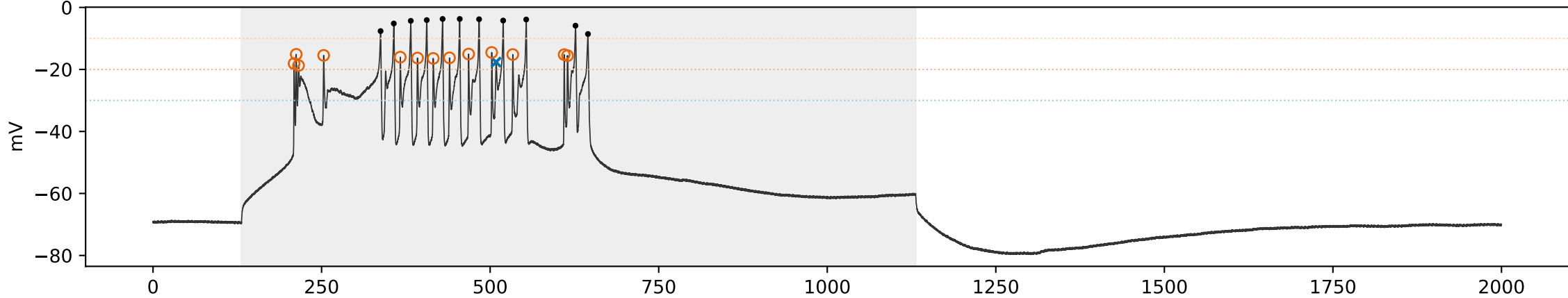
WT WT_02 | sweep 7 | 350.0 pA | primary=16, strict=7
