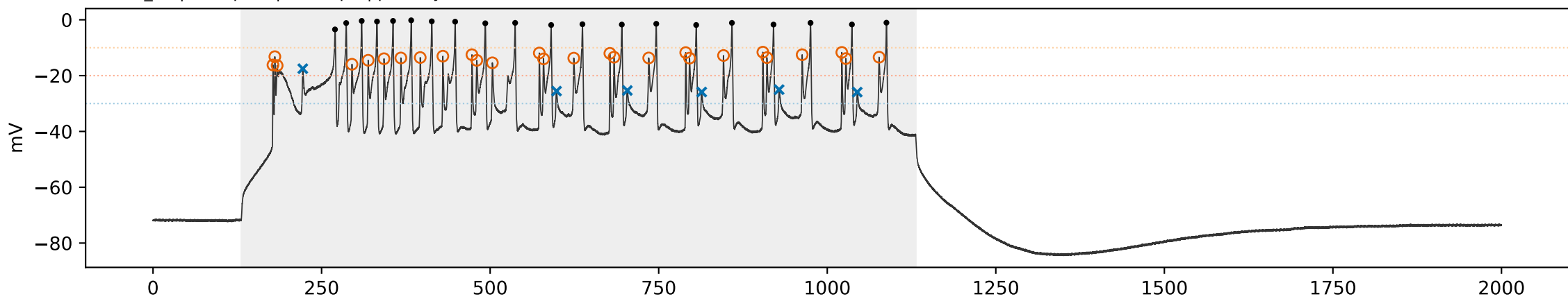
WT WT_02 | sweep 11 | 550.0 pA | primary=19, strict=10
