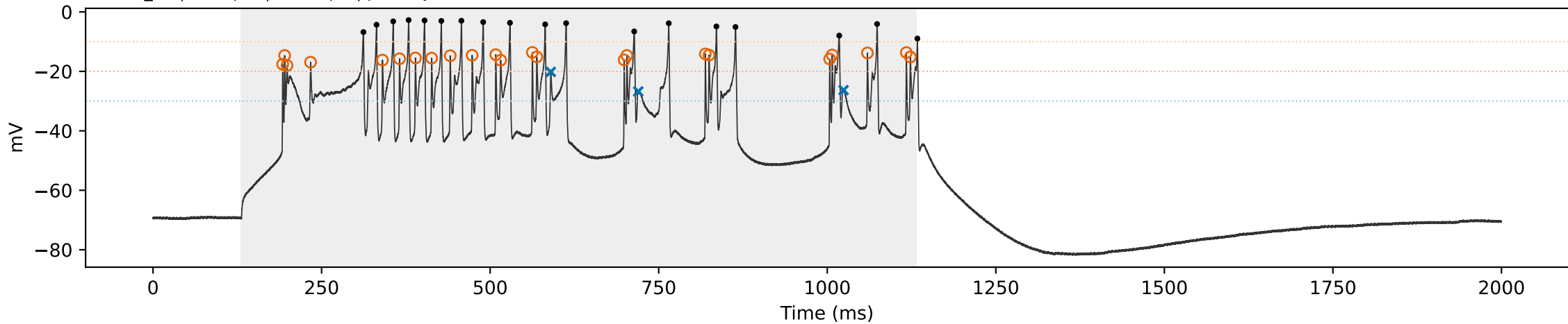
WT WT_02 | sweep 7 | 350.0 pA | primary=16, strict=7
