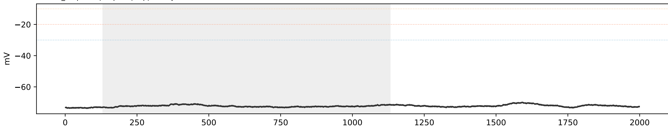
WT WT_06 | sweep 1 | 50.0 pA | primary=0, strict=0
