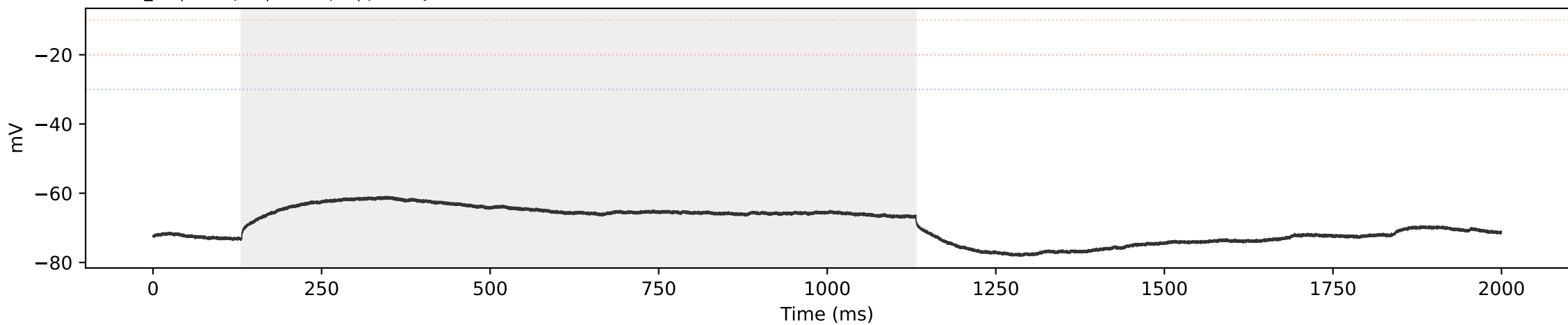
WT WT_06 | sweep 3 | 150.0 pA | primary=0, strict=0
