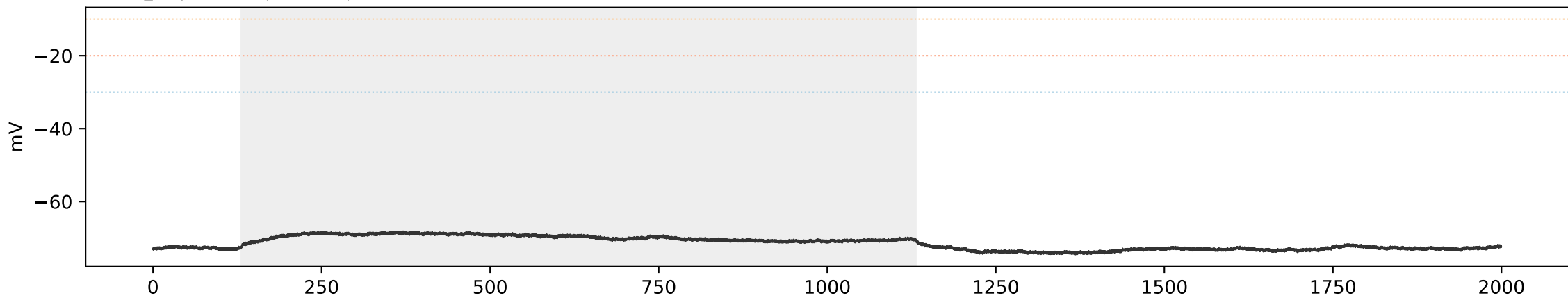
WT WT_06 | sweep 2 | 100.0 pA | primary=0, strict=0
