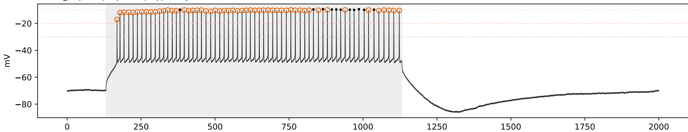
WT WT_06 | sweep 9 | 450.0 pA | primary=35, strict=32
