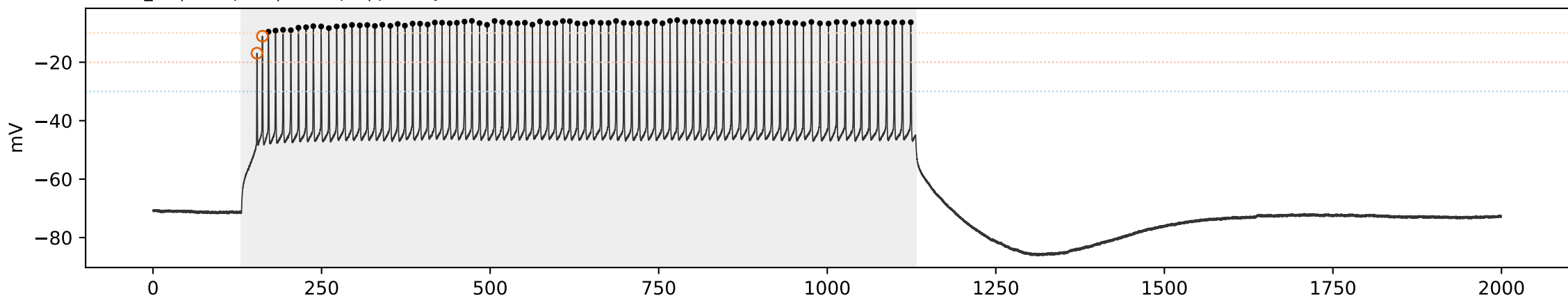
WT WT_06 | sweep 11 | 550.0 pA | primary=45, strict=45
