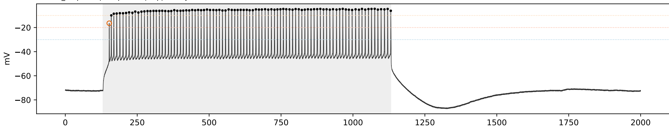
WT WT_06 | sweep 13 | 650.0 pA | primary=54, strict=54
