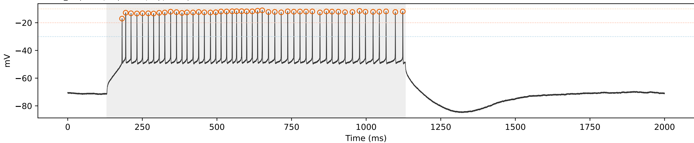
WT WT_06 | sweep 7 | 350.0 pA | primary=24, strict=0
