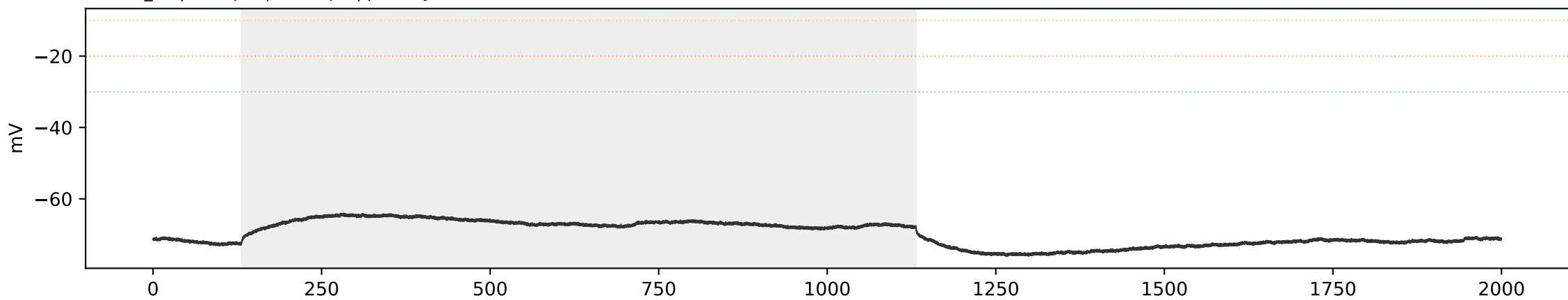
WT WT_06 | sweep 3 | 150.0 pA | primary=0, strict=0
