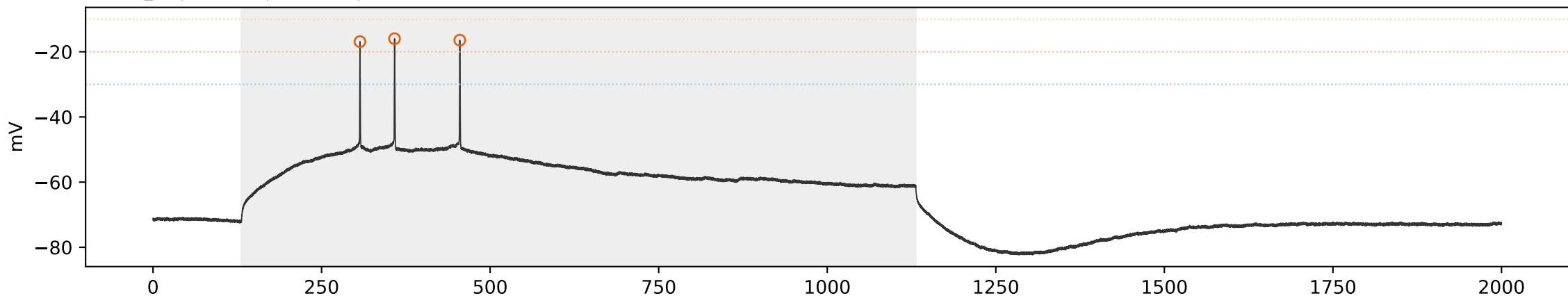
WT WT_06 | sweep 6 | 300.0 pA | primary=7, strict=0
