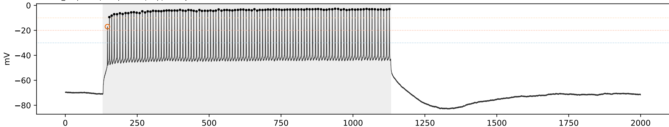
WT WT_06 | sweep 14 | 700.0 pA | primary=56, strict=56
