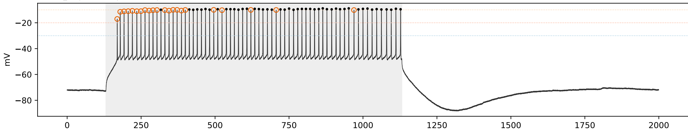
WT WT_06 | sweep 10 | 500.0 pA | primary=41, strict=41
