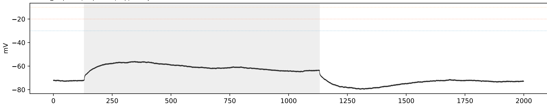
WT WT_06 | sweep 5 | 250.0 pA | primary=0, strict=0
