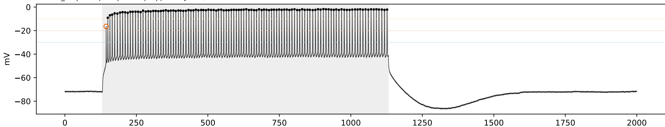
WT WT_06 | sweep 15 | 750.0 pA | primary=57, strict=57
