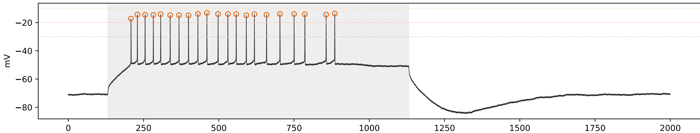
WT WT_06 | sweep 7 | 350.0 pA | primary=24, strict=0
