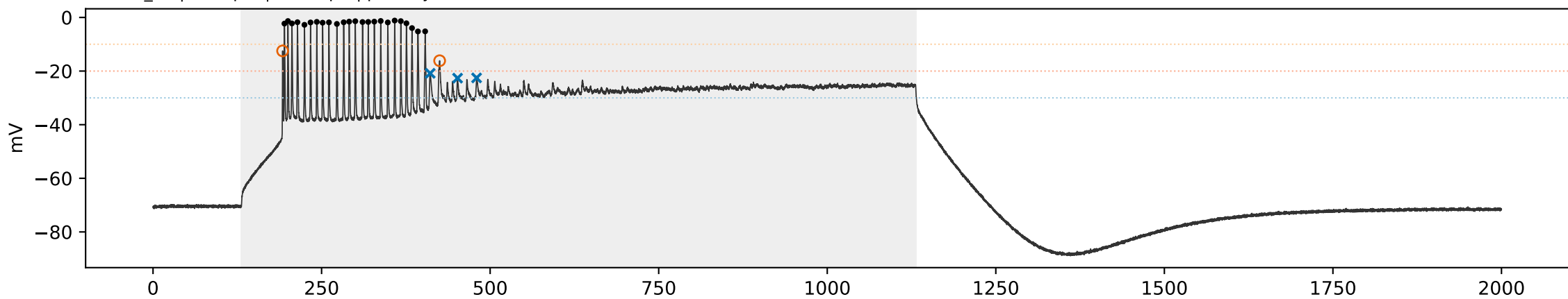
WT WT_08 | sweep 10 | 500.0 pA | primary=0, strict=0
