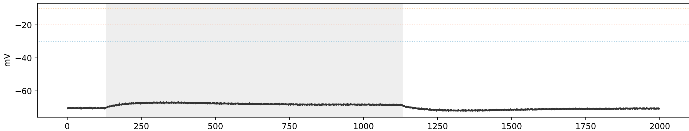
WT WT_08 | sweep 2 | 100.0 pA | primary=0, strict=0
