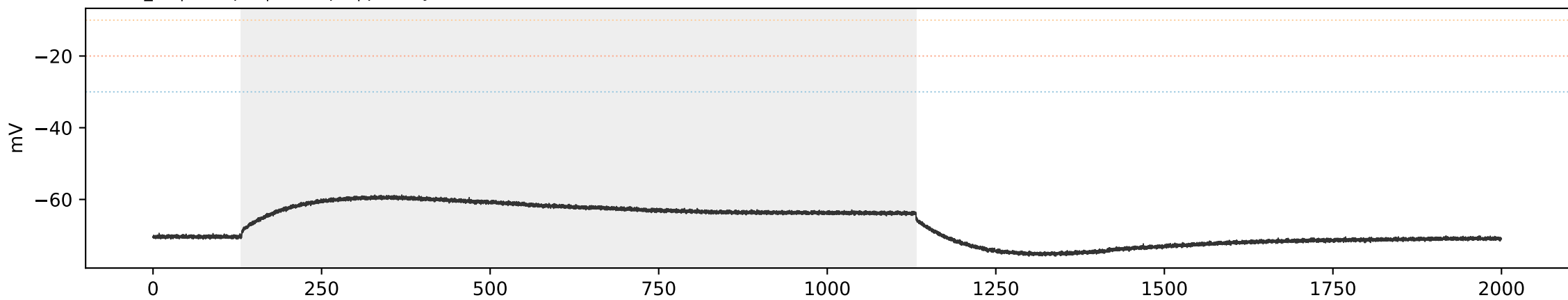
WT WT_08 | sweep 3 | 150.0 pA | primary=0, strict=0
