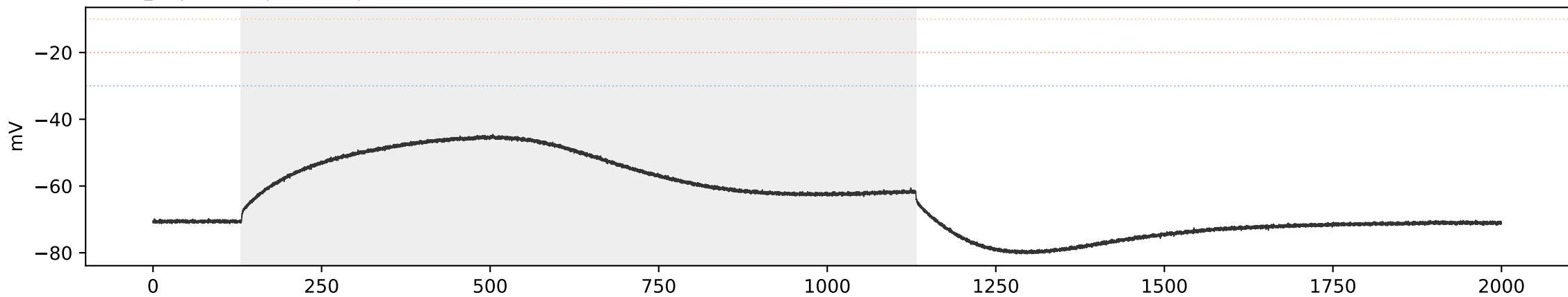
WT WT_08 | sweep 6 | 300.0 pA | primary=16, strict=16
