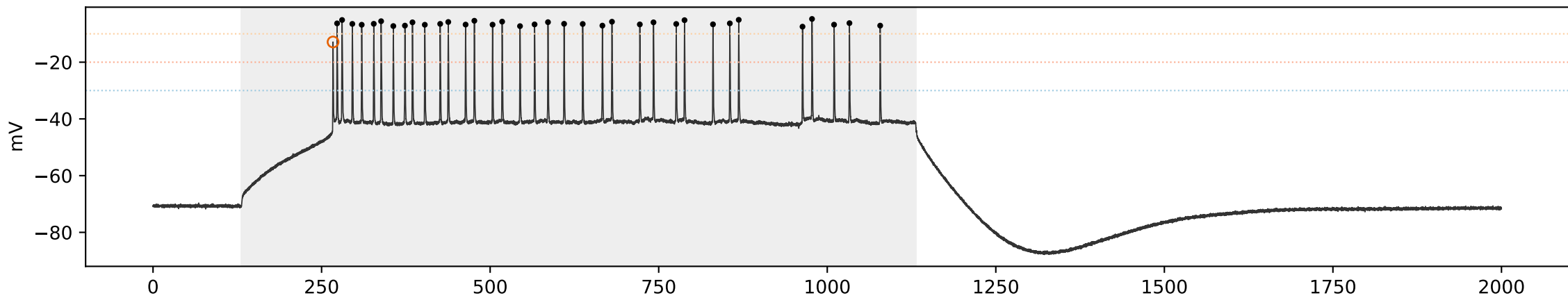
WT WT_08 | sweep 7 | 350.0 pA | primary=39, strict=39
