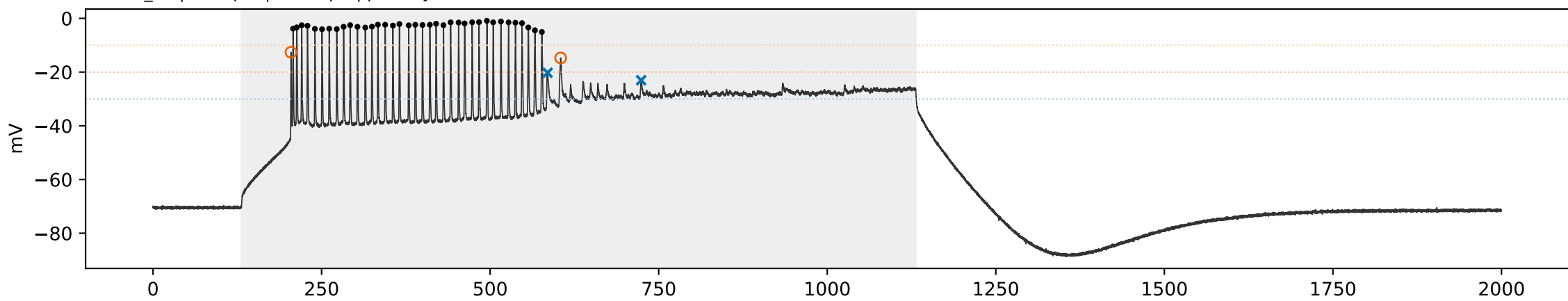
WT WT_08 | sweep 9 | 450.0 pA | primary=0, strict=0
