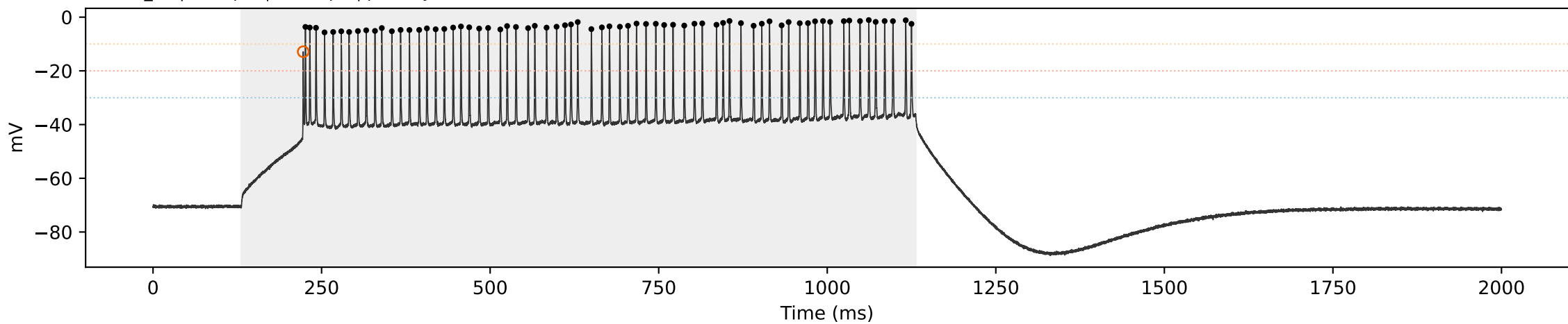
WT WT_08 | sweep 7 | 350.0 pA | primary=39, strict=39
