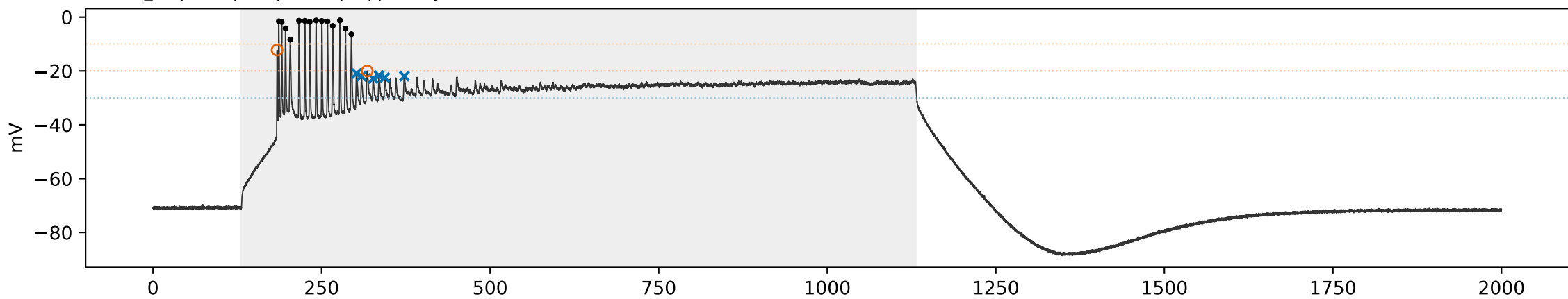
WT WT_08 | sweep 11 | 550.0 pA | primary=0, strict=0
