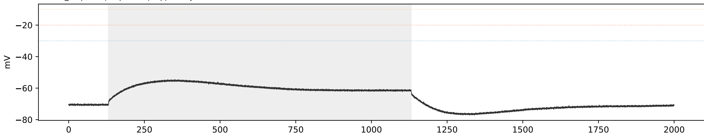
WT WT_08 | sweep 5 | 250.0 pA | primary=0, strict=0
