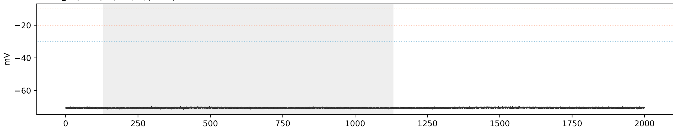
WT WT_08 | sweep 1 | 50.0 pA | primary=0, strict=0
