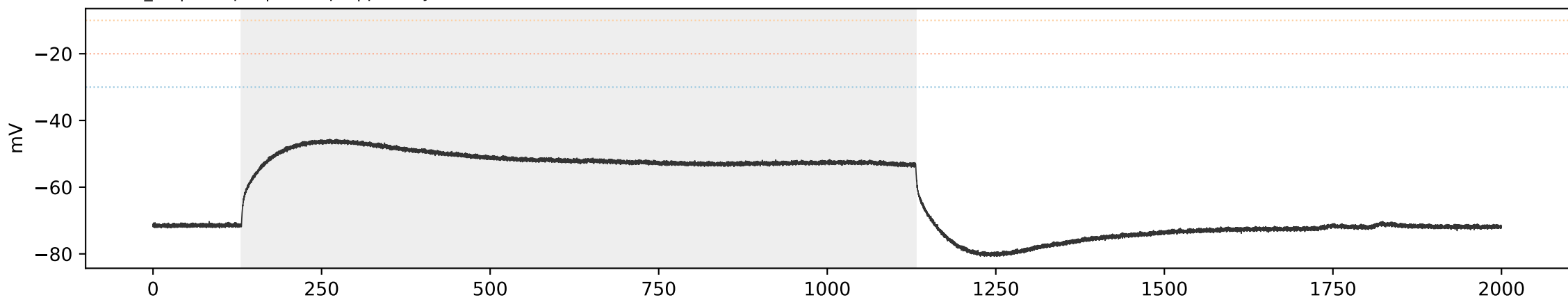
WT WT_11 | sweep 7 | 350.0 pA | primary=0, strict=0
