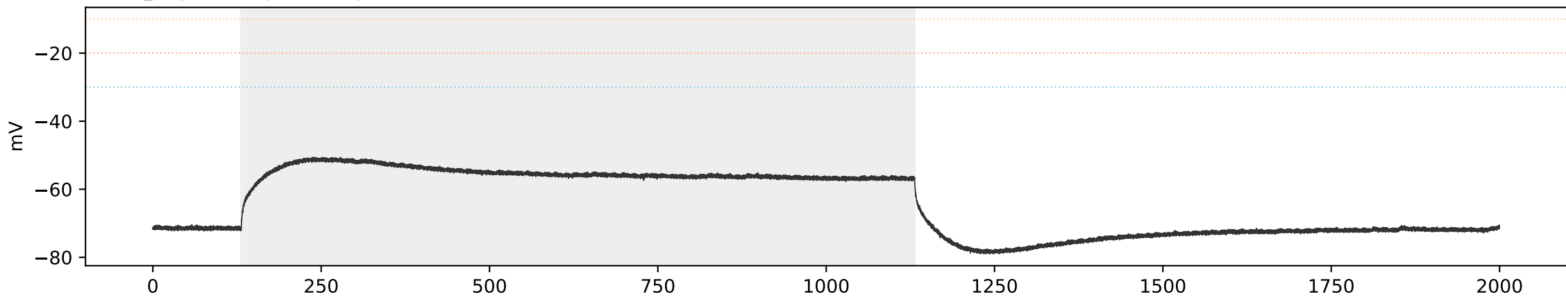
WT WT_11 | sweep 6 | 300.0 pA | primary=0, strict=0
