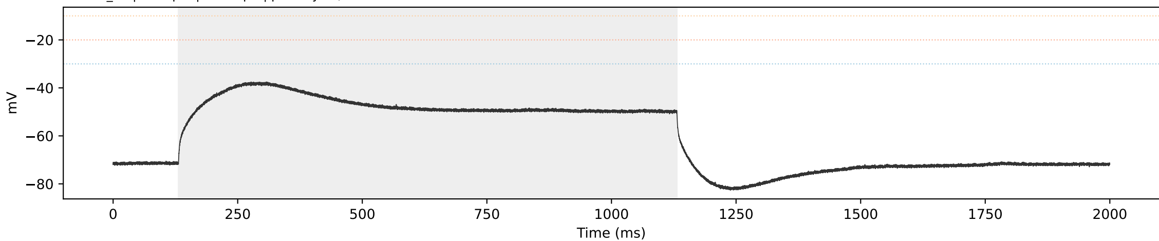
WT WT_11 | sweep 7 | 350.0 pA | primary=0, strict=0
