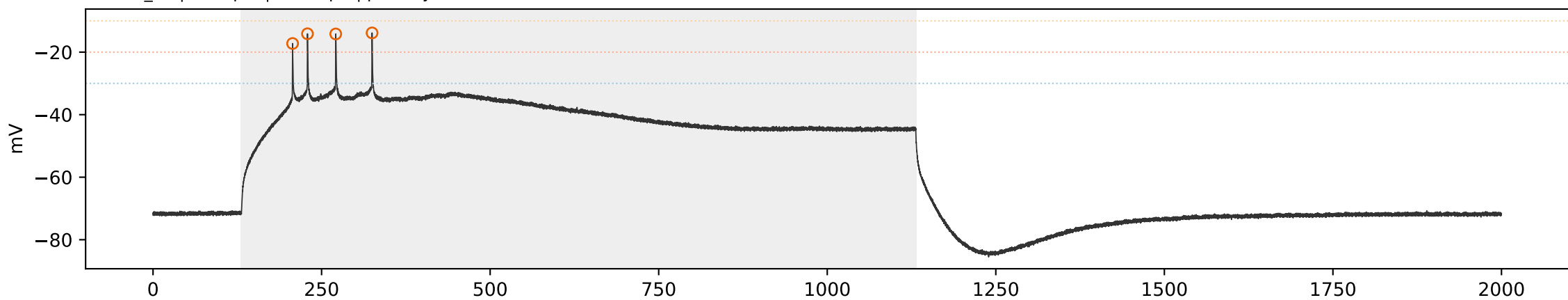
WT WT_11 | sweep 9 | 450.0 pA | primary=12, strict=0
