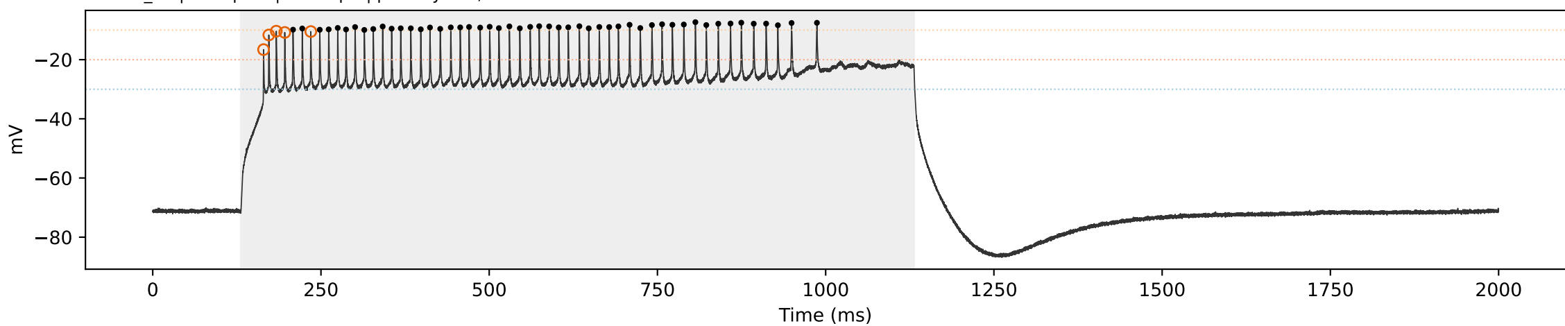
WT WT_11 | sweep 11 | 550.0 pA | primary=23, strict=23
