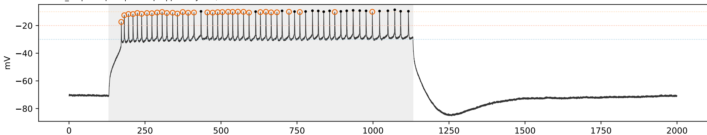
WT WT_11 | sweep 11 | 550.0 pA | primary=23, strict=23
