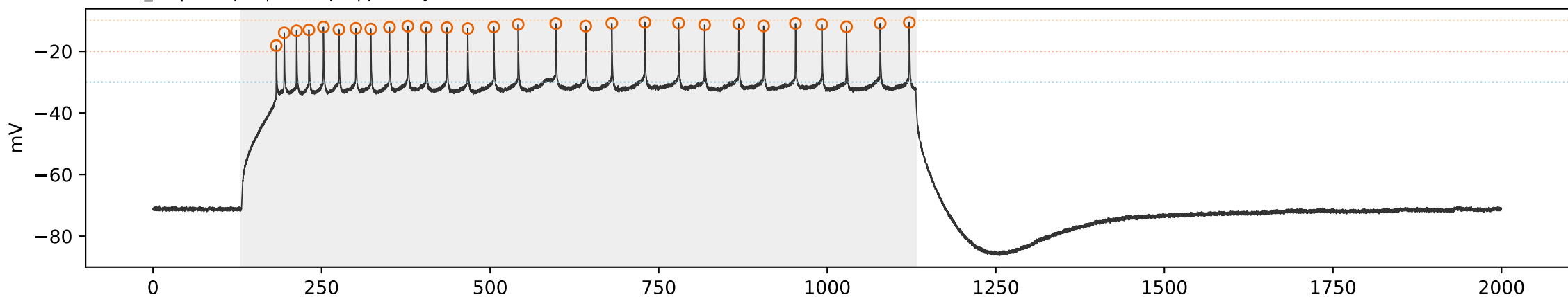
WT WT_11 | sweep 10 | 500.0 pA | primary=26, strict=18
