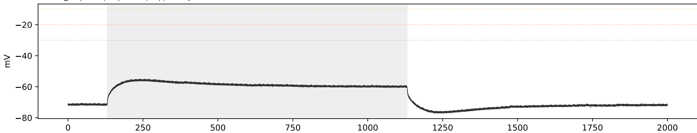
WT WT_11 | sweep 5 | 250.0 pA | primary=0, strict=0
