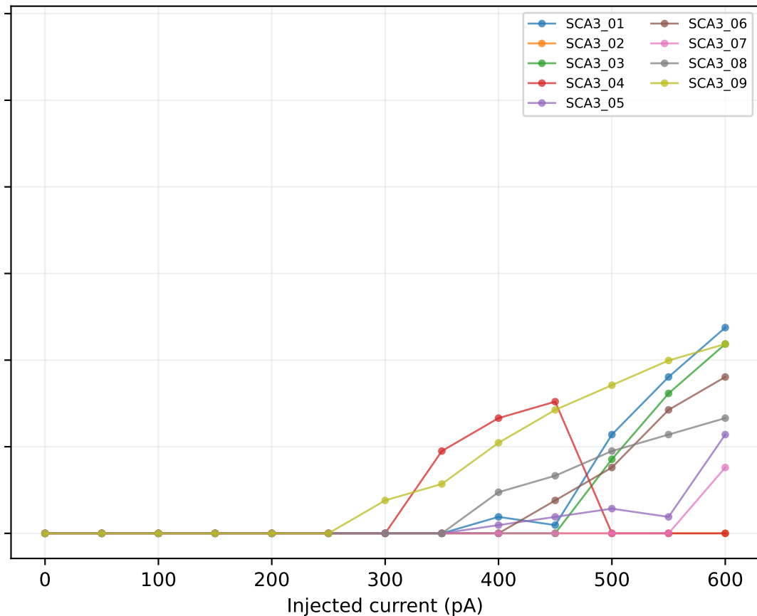
SCA3: every cell, primary detector
