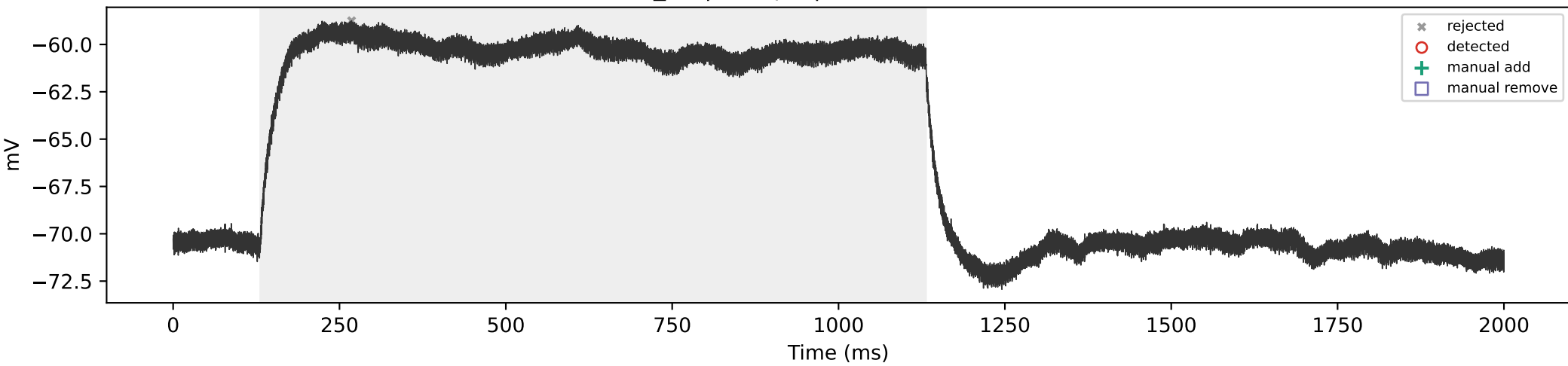
SCA3_09 | 100 pA | total=0, sustained=0
