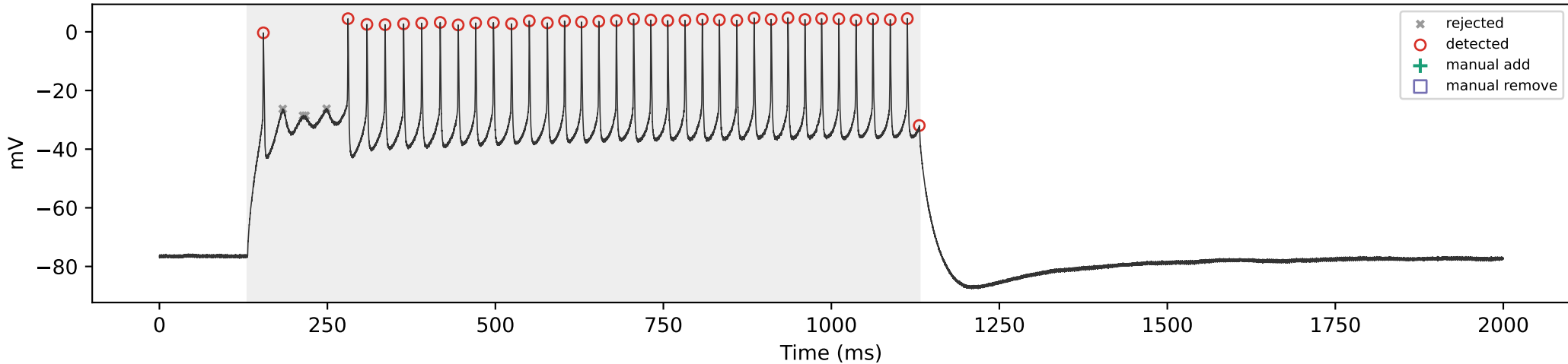
SCA3_09 | 550 pA | total=34, sustained=34
