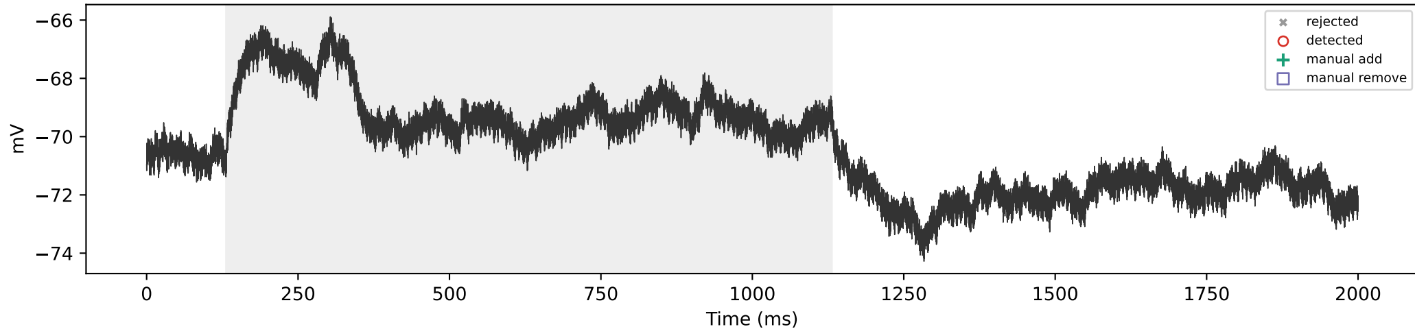
WT_03 | 50 pA | total=0, sustained=0
