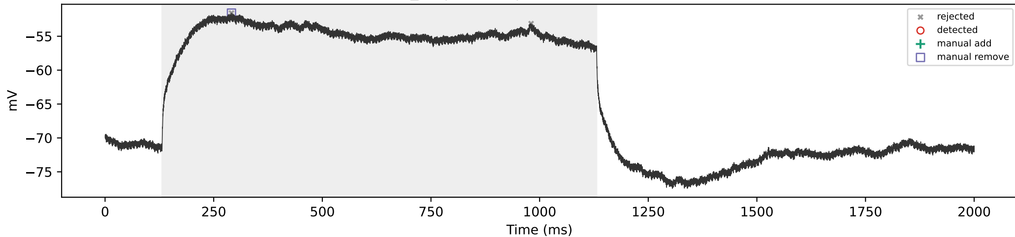
WT_03 | 250 pA | total=0, sustained=0
