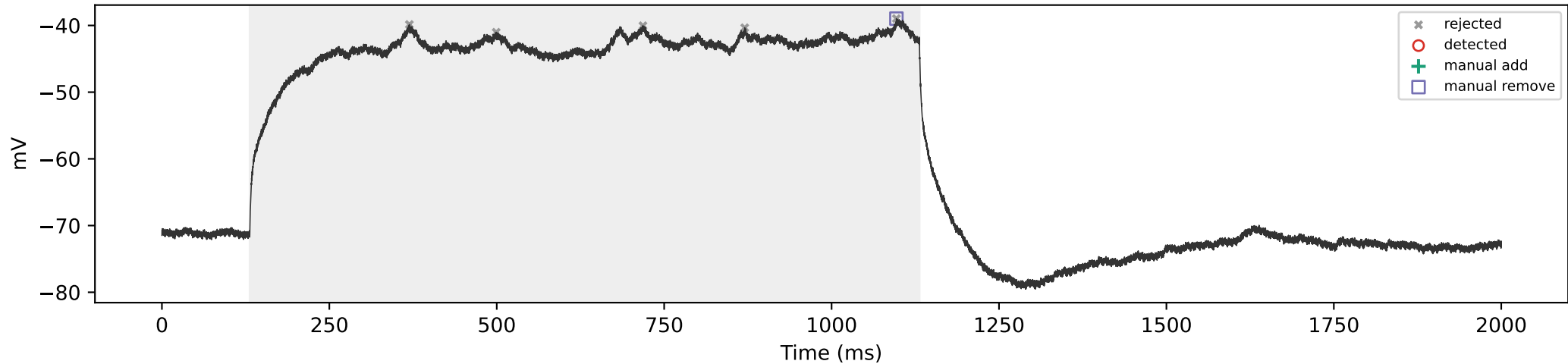
WT_03 | 350 pA | total=0, sustained=0
