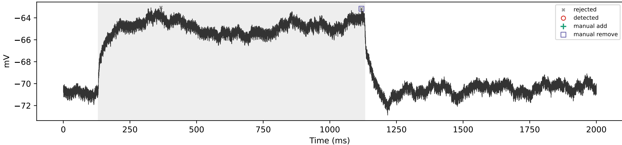
WT_03 | 100 pA | total=0, sustained=0
