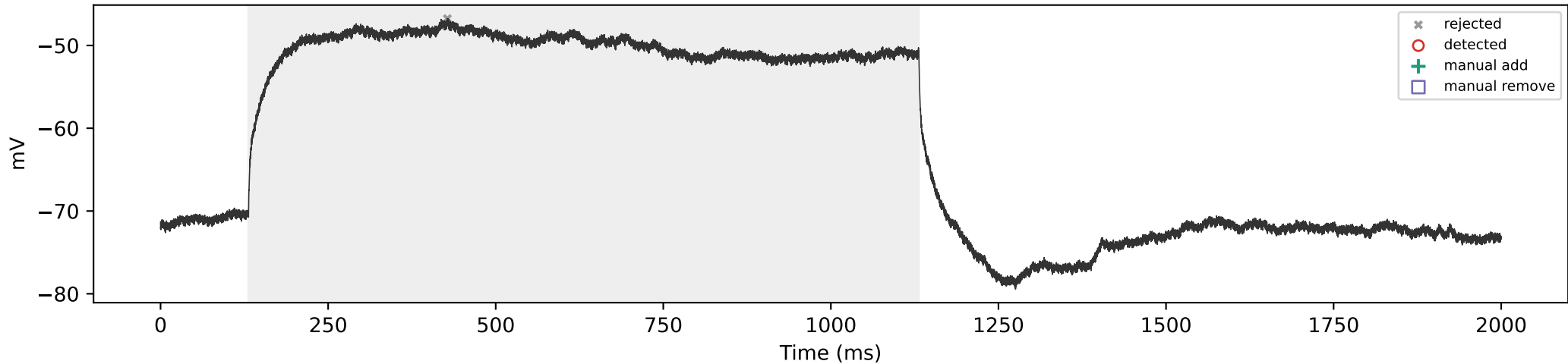
WT_03 | 300 pA | total=0, sustained=0
