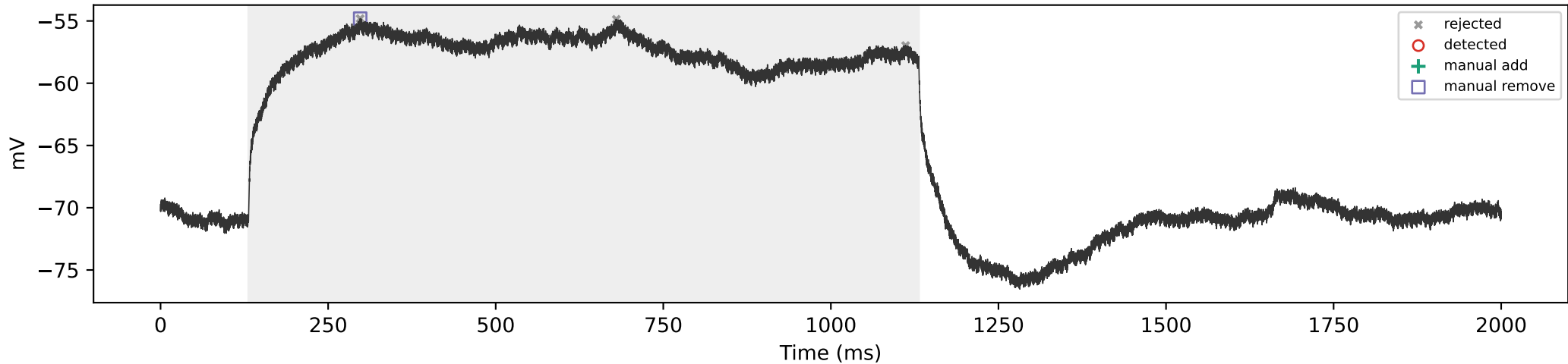
WT_03 | 200 pA | total=0, sustained=0
