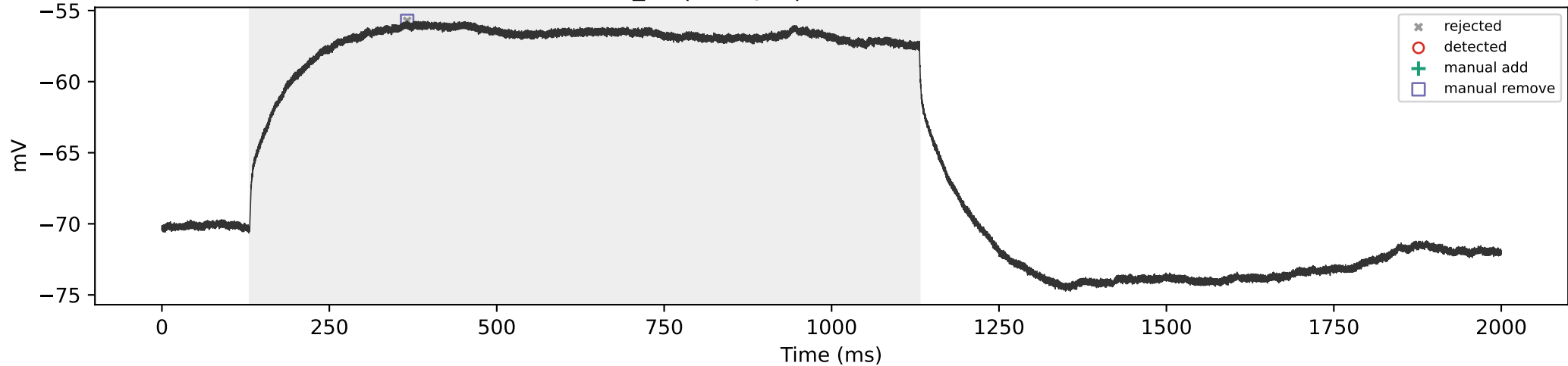
WT_07 | 150 pA | total=0, sustained=0
