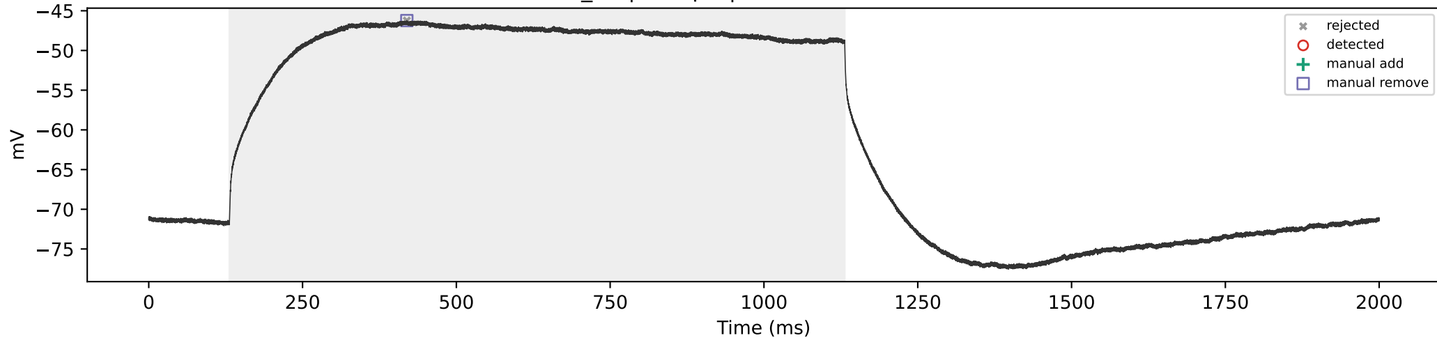
WT_07 | 250 pA | total=0, sustained=0
