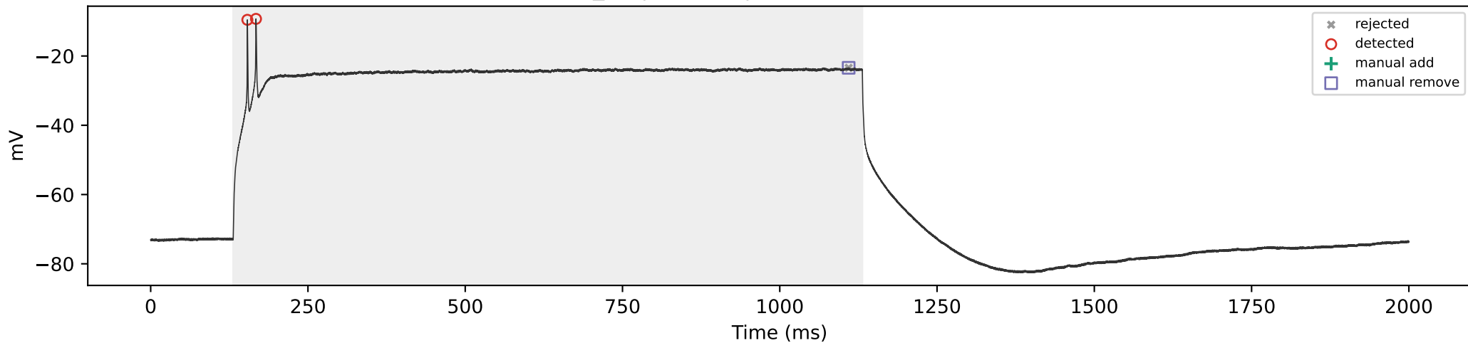
WT_07 | 800 pA | total=2, sustained=2
