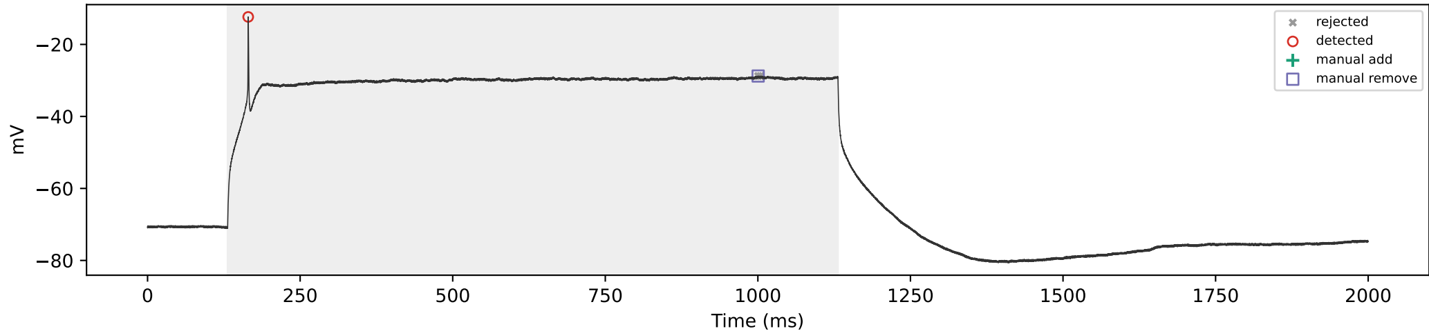
WT_07 | 600 pA | total=1, sustained=0
