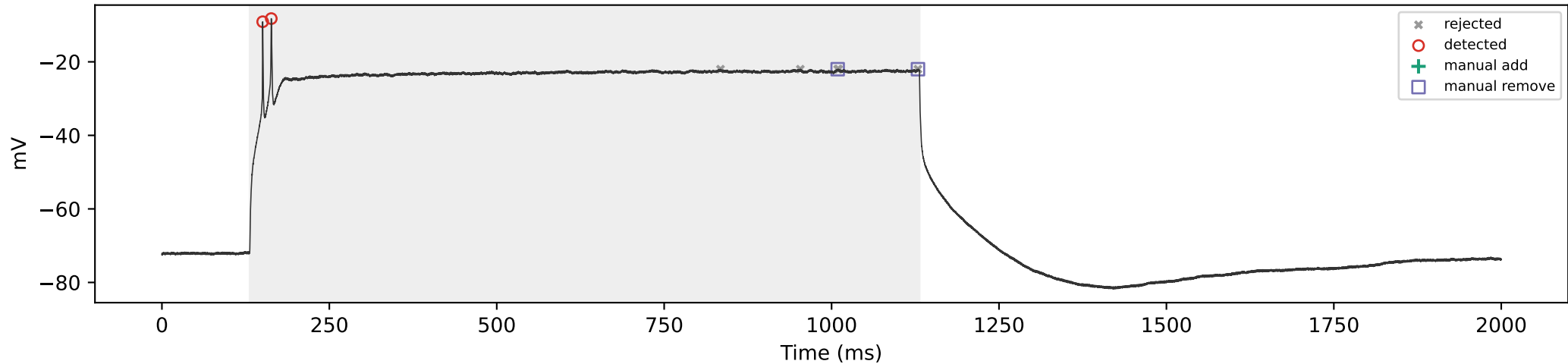
WT_07 | 850 pA | total=2, sustained=2
