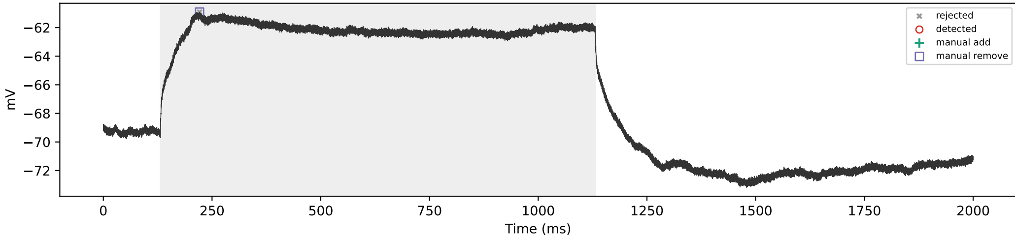
WT_07 | 100 pA | total=0, sustained=0
