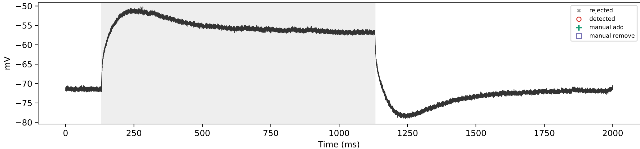
WT_11 | 250 pA | total=0, sustained=0
