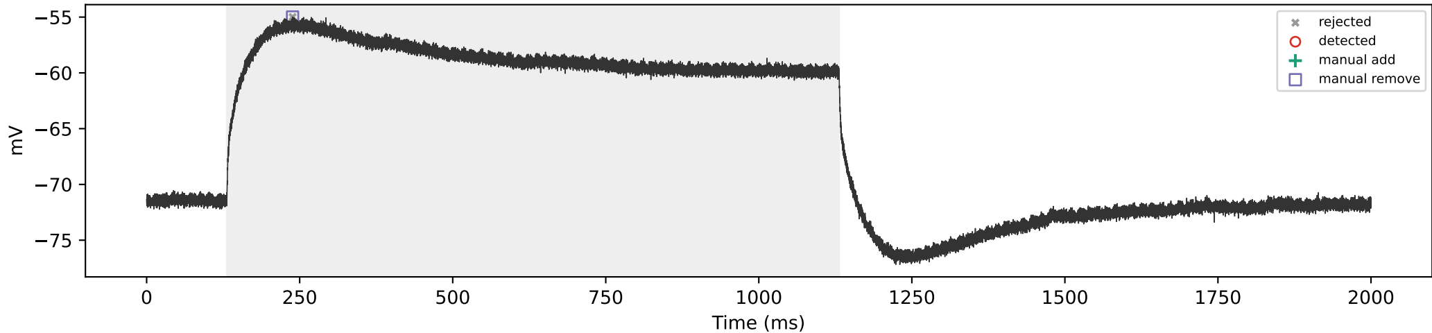
WT_11 | 200 pA | total=0, sustained=0
