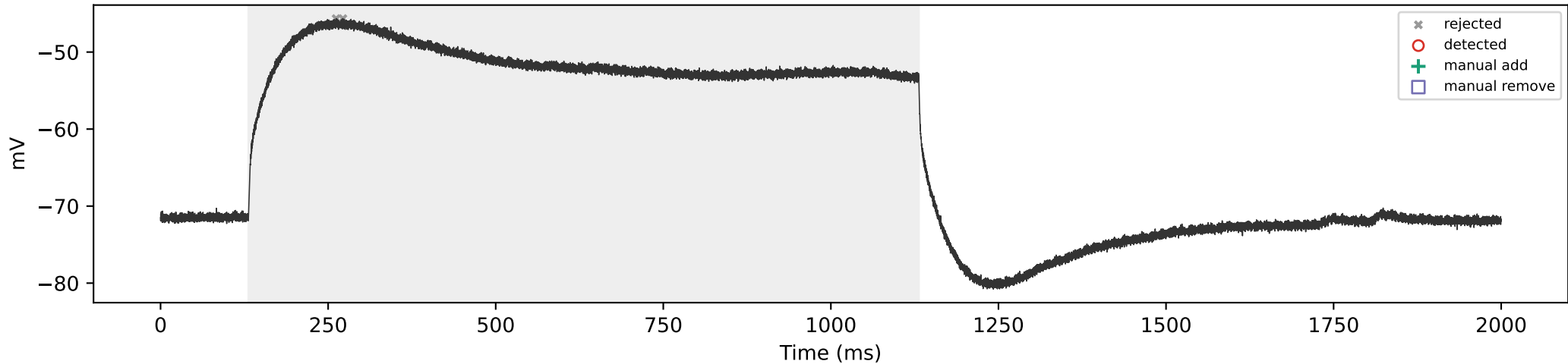
WT_11 | 300 pA | total=0, sustained=0
