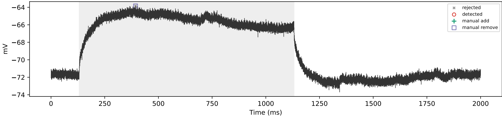
WT_13 | 100 pA | total=0, sustained=0
