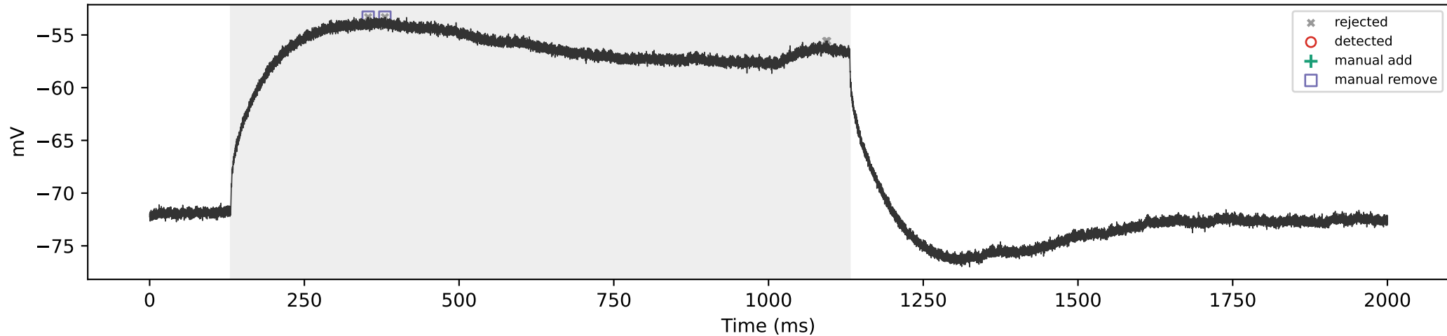
WT_13 | 250 pA | total=0, sustained=0
