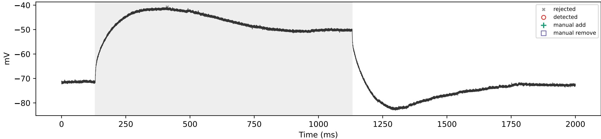
WT_13 | 400 pA | total=0, sustained=0
