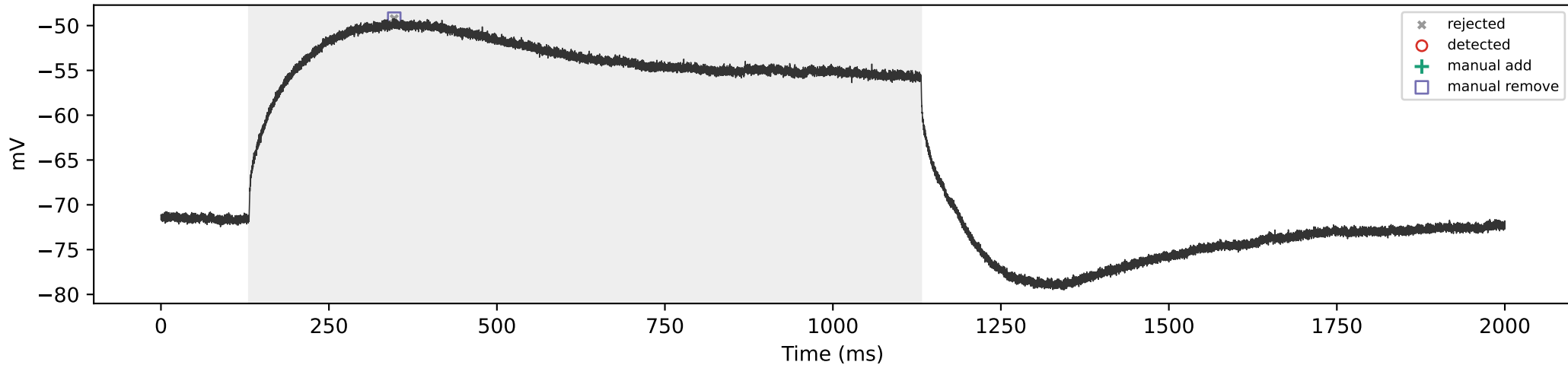
WT_13 | 300 pA | total=0, sustained=0
