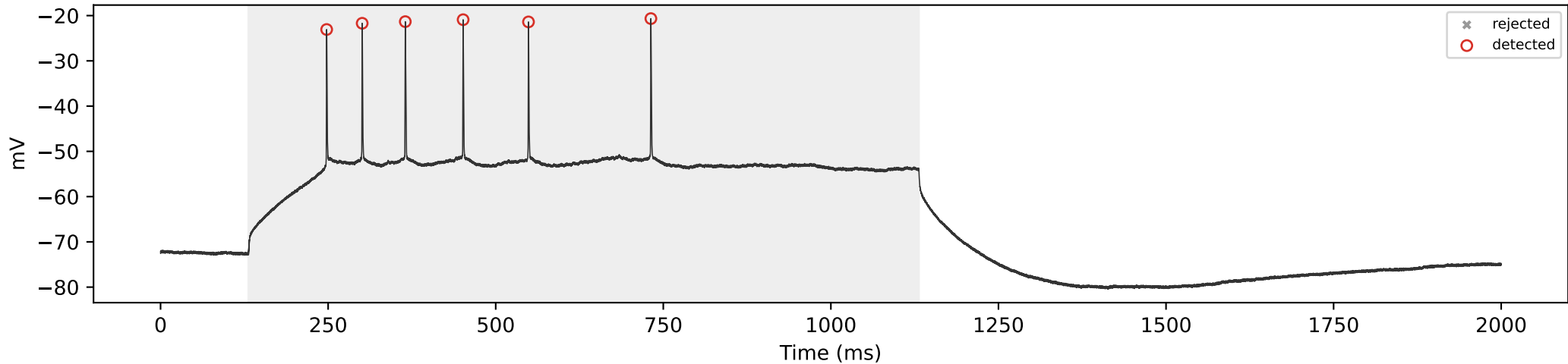
WT_04 | 250 pA | total=6, sustained=6
