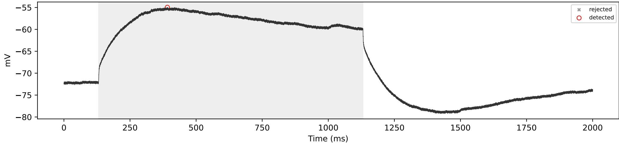
WT_04 | 200 pA | total=1, sustained=0
