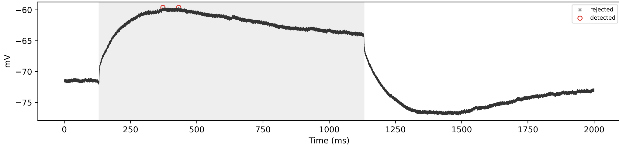
WT_04 | 150 pA | total=2, sustained=2
