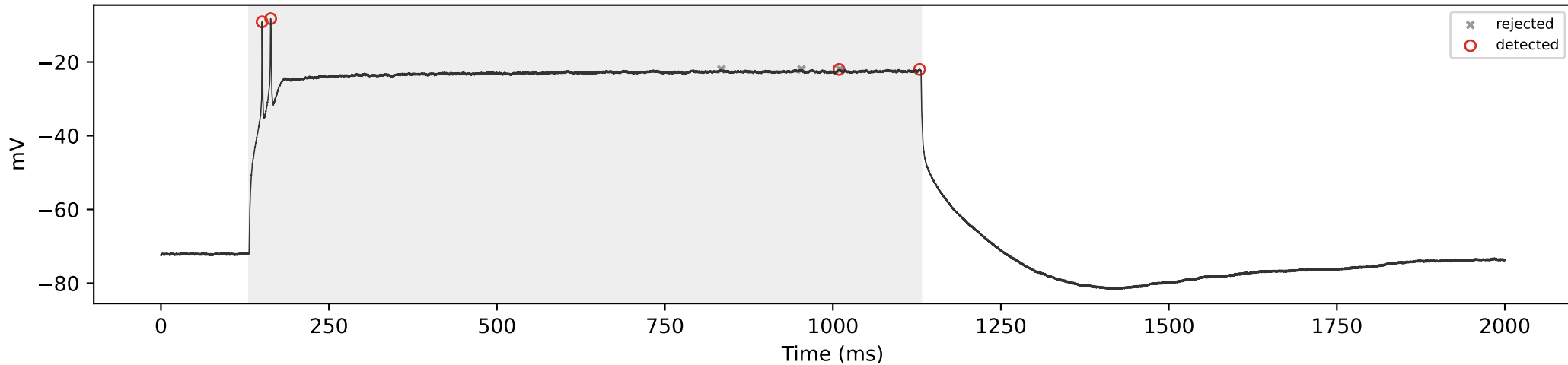
WT_07 | 850 pA | total=3, sustained=2
