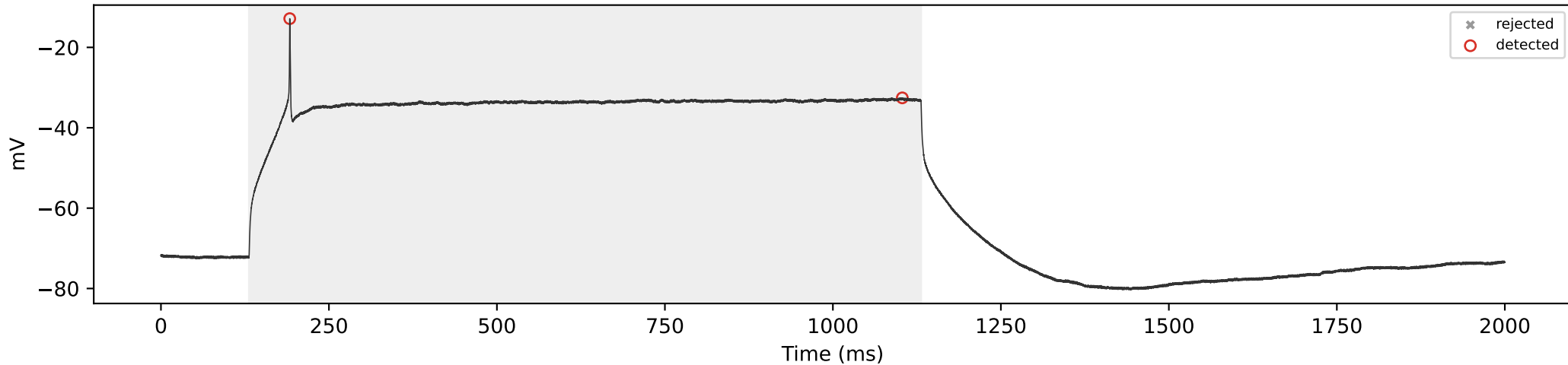
WT_07 | 500 pA | total=2, sustained=0
