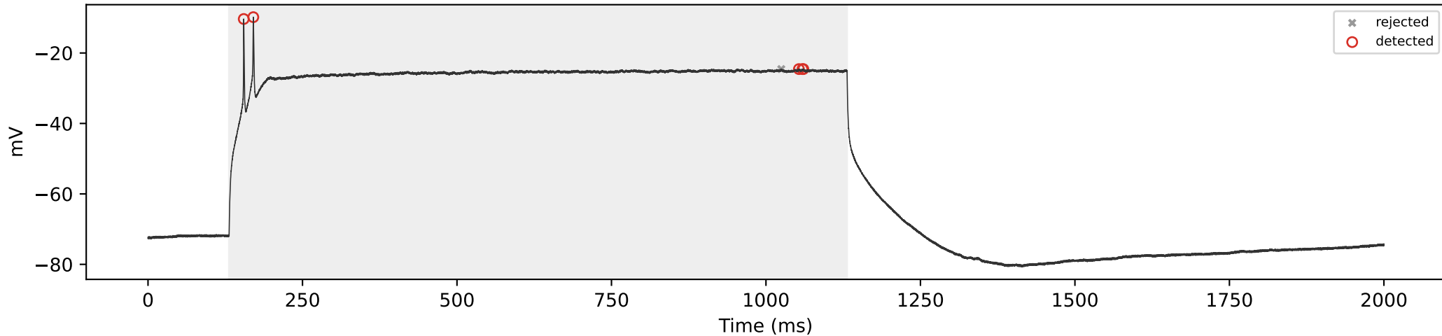
WT_07 | 750 pA | total=5, sustained=5
