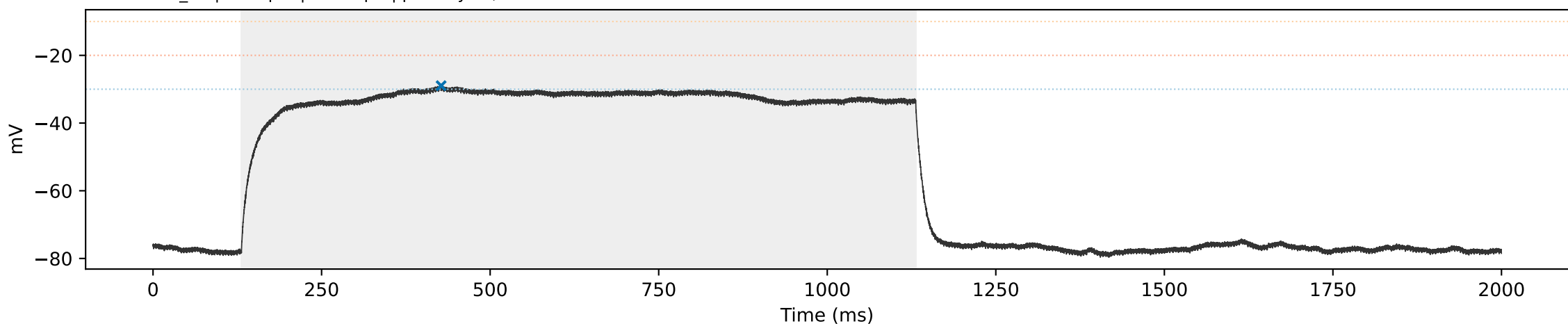
SCA3 SCA3_01 | sweep 7 | 350.0 pA | primary=0, strict=0
