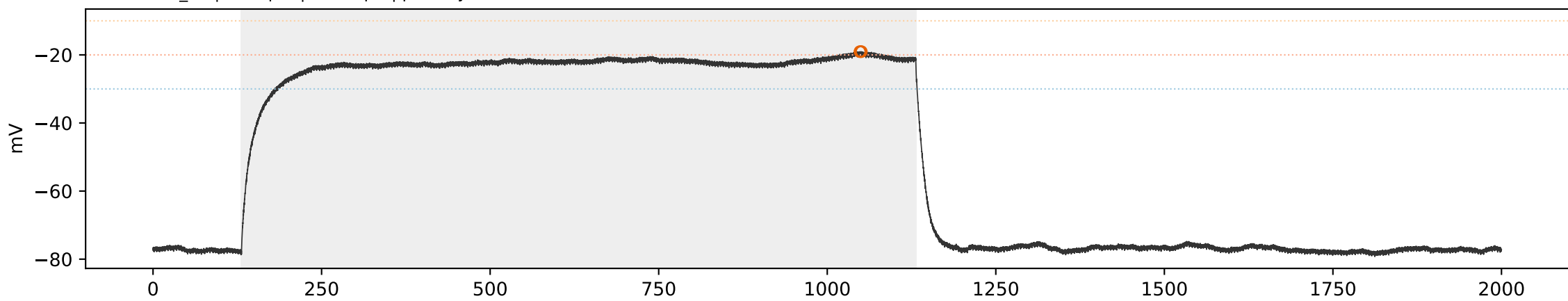
SCA3 SCA3_01 | sweep 9 | 450.0 pA | primary=1, strict=0
