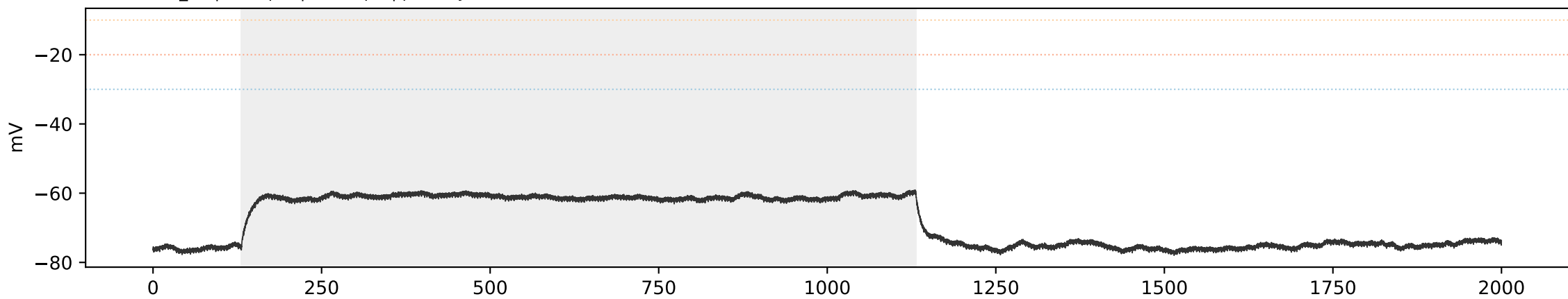
SCA3 SCA3_01 | sweep 3 | 150.0 pA | primary=0, strict=0
