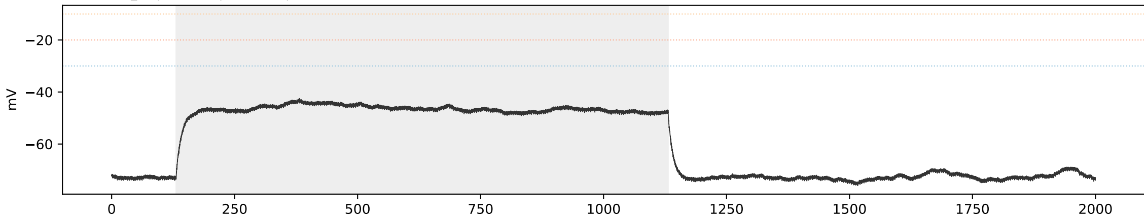
SCA3 SCA3_01 | sweep 6 | 300.0 pA | primary=0, strict=0
