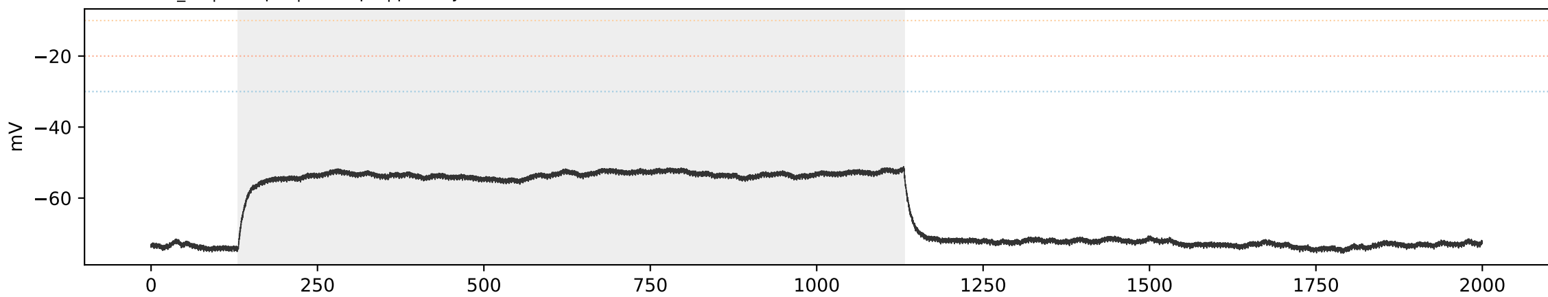
SCA3 SCA3_01 | sweep 5 | 250.0 pA | primary=0, strict=0
