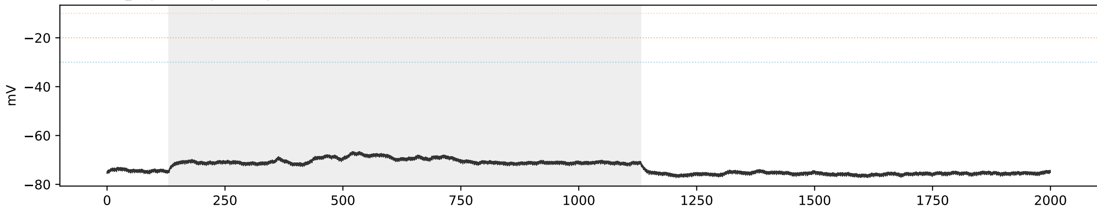
SCA3 SCA3_01 | sweep 2 | 100.0 pA | primary=0, strict=0
