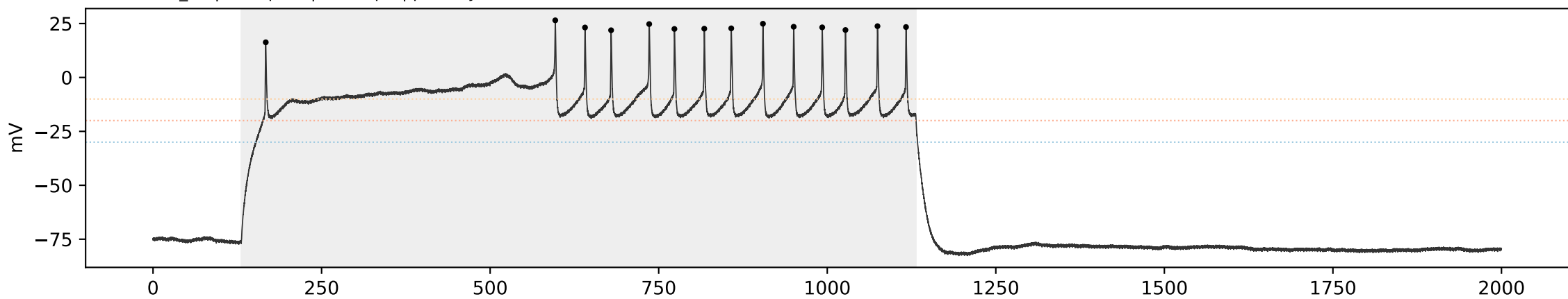
SCA3 SCA3_01 | sweep 11 | 550.0 pA | primary=19, strict=19
