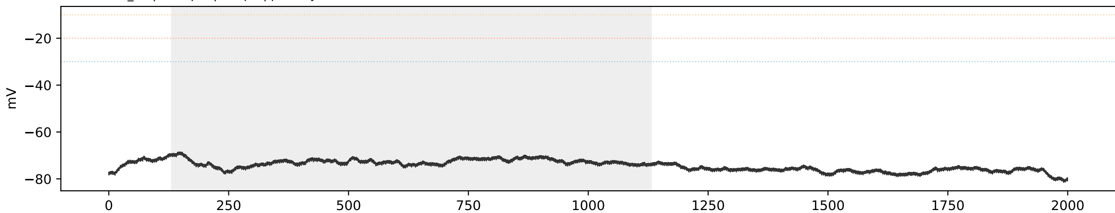
SCA3 SCA3_01 | sweep 1 | 50.0 pA | primary=0, strict=0
