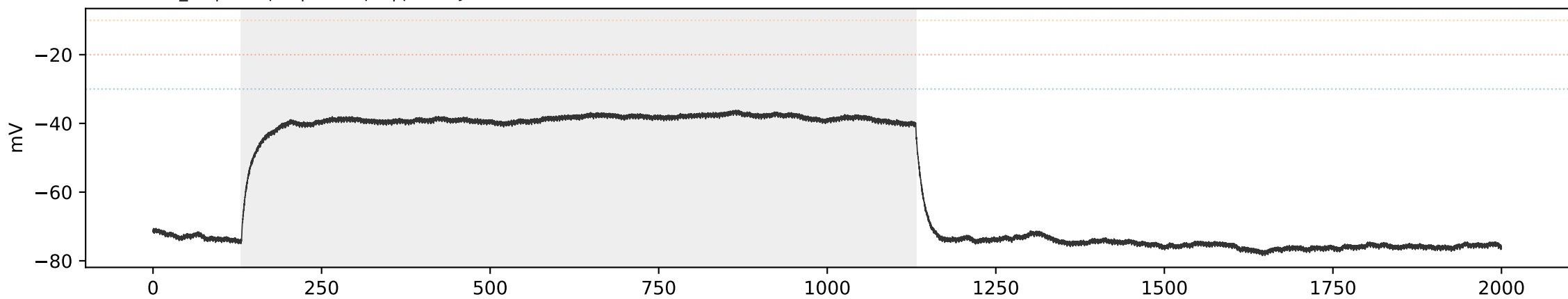
SCA3 SCA3_01 | sweep 7 | 350.0 pA | primary=0, strict=0
