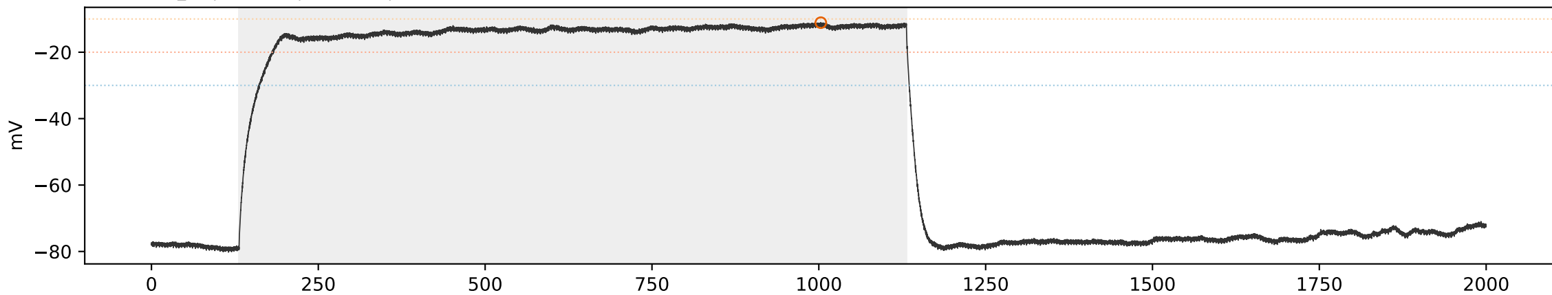
SCA3 SCA3_01 | sweep 10 | 500.0 pA | primary=12, strict=12
