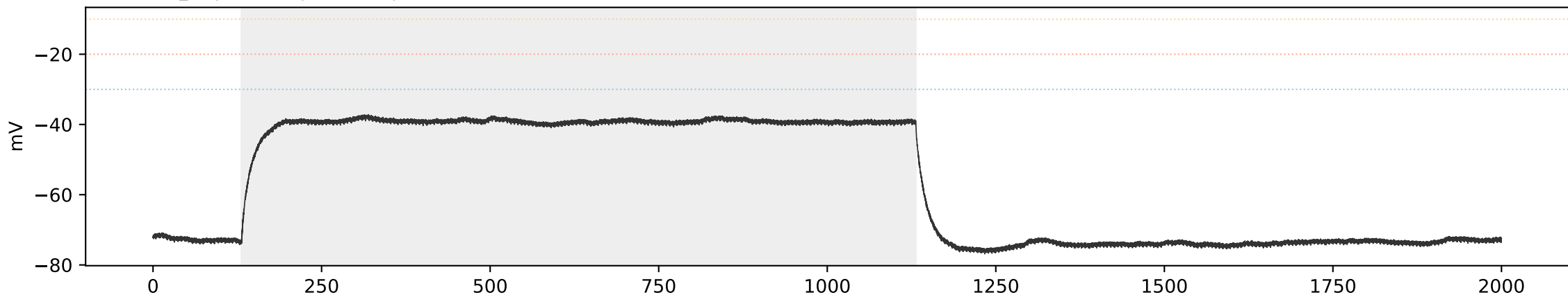
SCA3 SCA3_03 | sweep 6 | 300.0 pA | primary=0, strict=0
