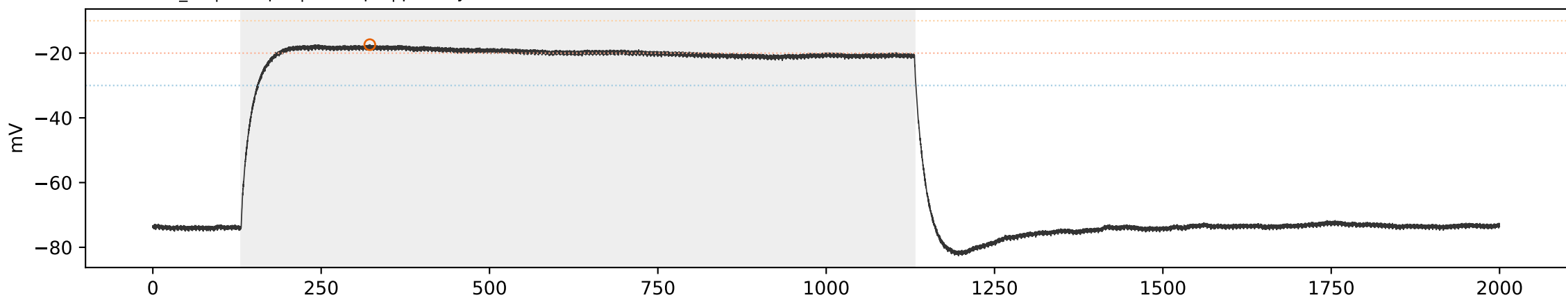
SCA3 SCA3_03 | sweep 9 | 450.0 pA | primary=0, strict=0
