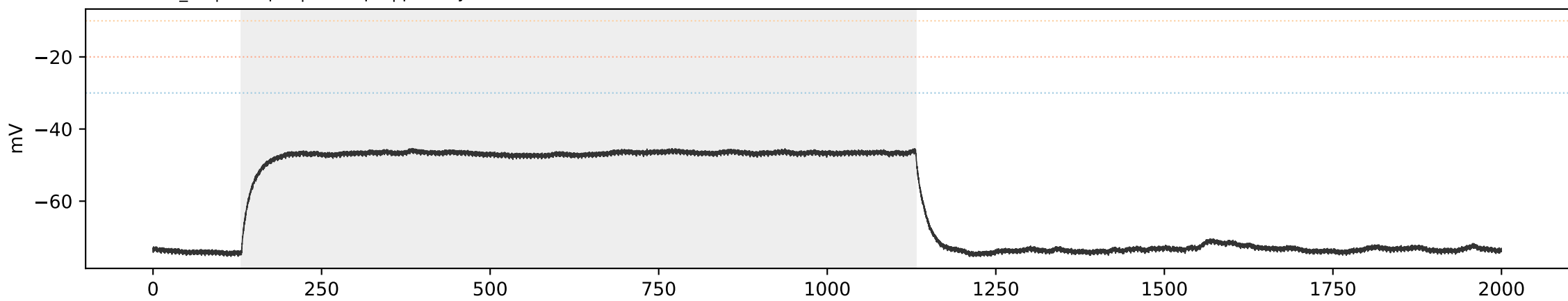
SCA3 SCA3_03 | sweep 5 | 250.0 pA | primary=0, strict=0
