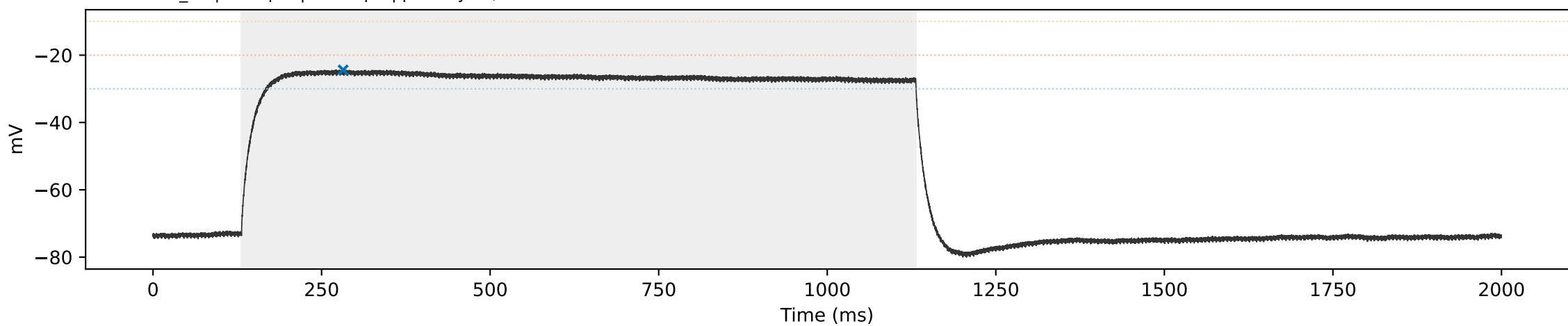
SCA3 SCA3_03 | sweep 7 | 350.0 pA | primary=0, strict=0
