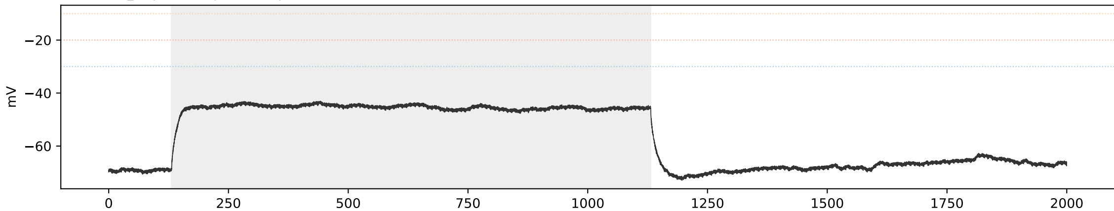
SCA3 SCA3_04 | sweep 6 | 300.0 pA | primary=0, strict=0
