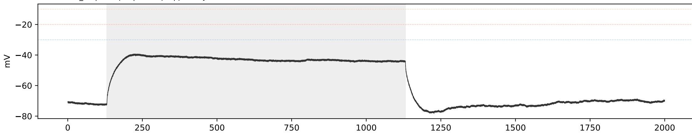
SCA3 SCA3_07 | sweep 9 | 450.0 pA | primary=0, strict=0
