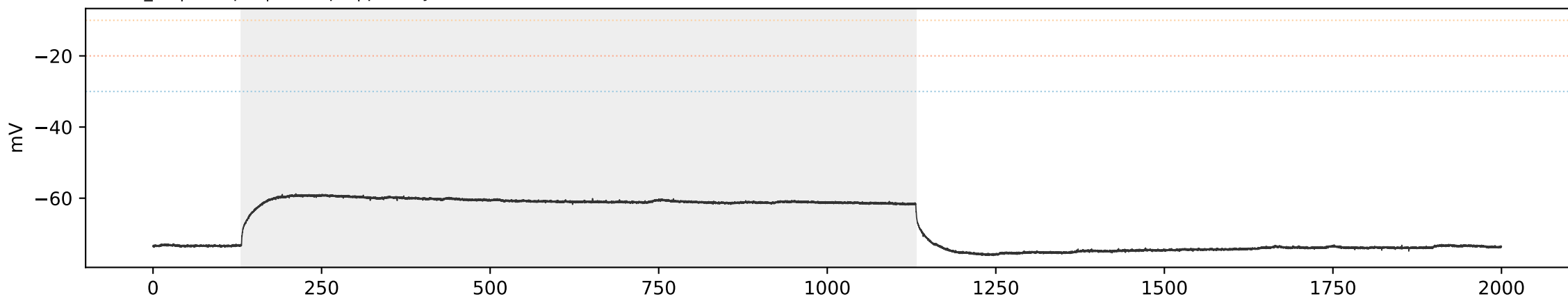
WT WT_12 | sweep 7 | 350.0 pA | primary=0, strict=0
