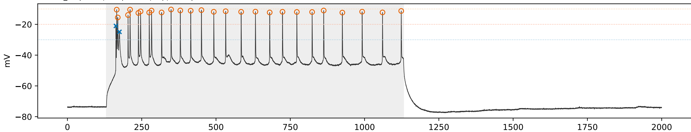
WT WT_12 | sweep 11 | 550.0 pA | primary=13, strict=13
