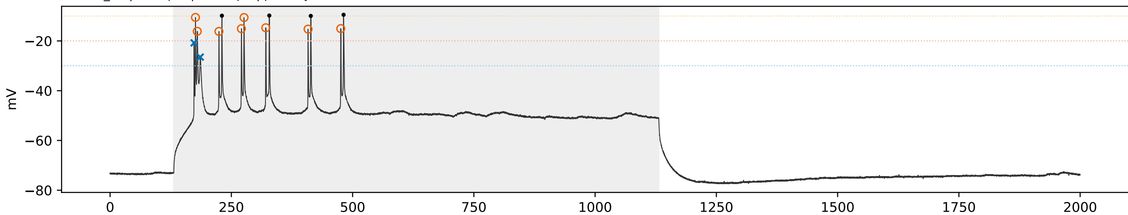
WT WT_12 | sweep 10 | 500.0 pA | primary=10, strict=0
