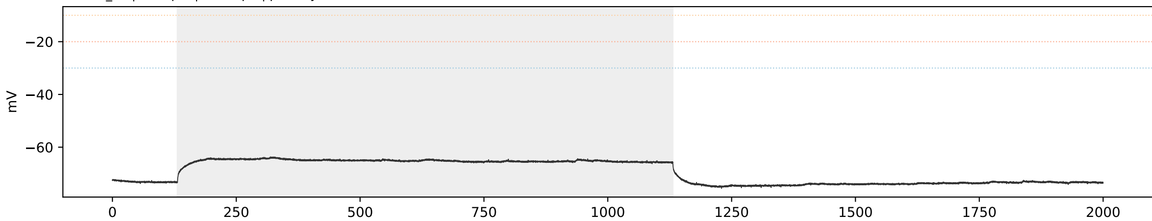
WT WT_12 | sweep 5 | 250.0 pA | primary=0, strict=0
