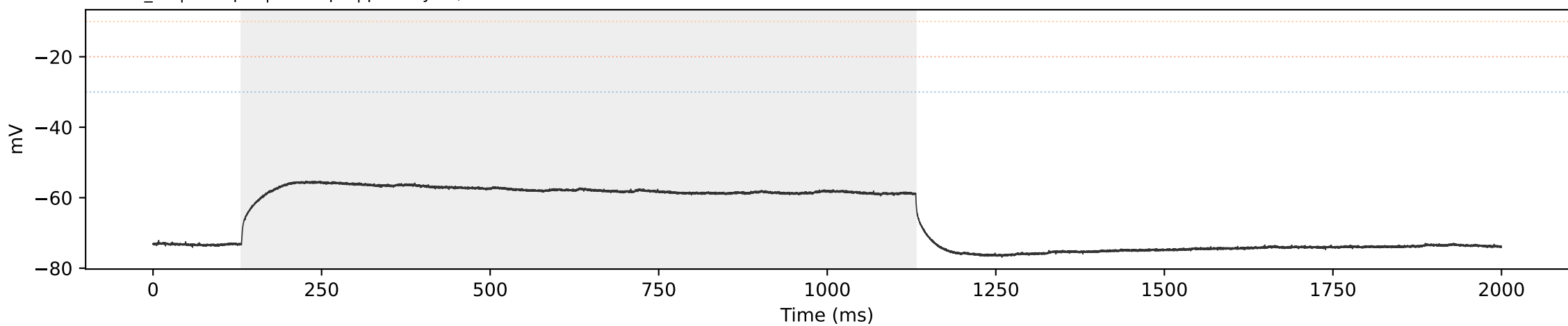
WT WT_12 | sweep 7 | 350.0 pA | primary=0, strict=0
