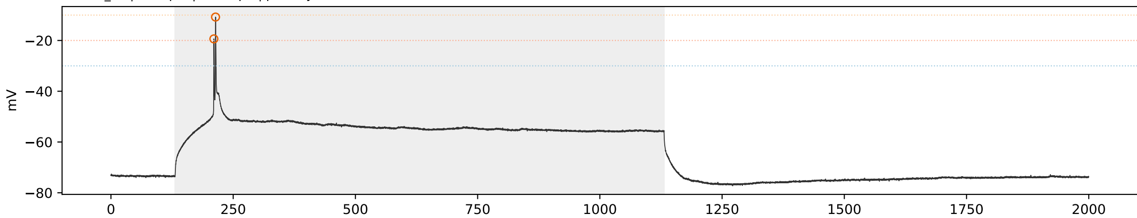
WT WT_12 | sweep 9 | 450.0 pA | primary=0, strict=0
