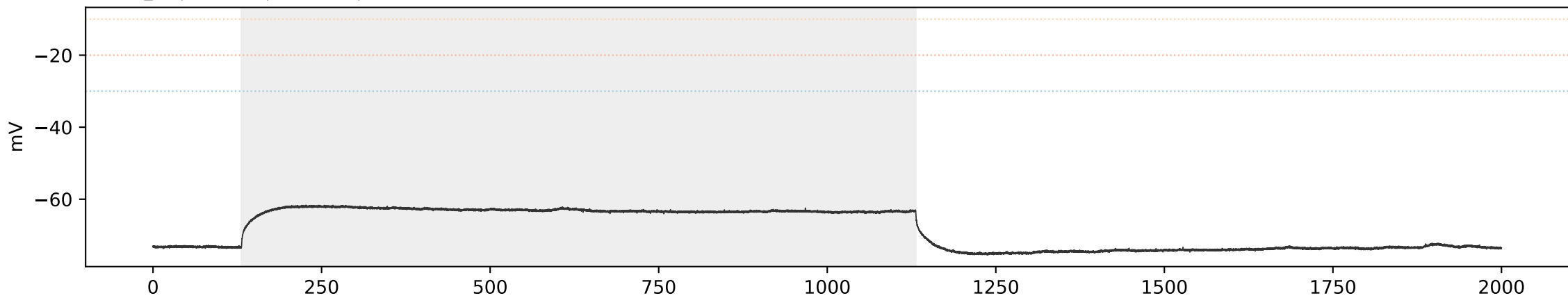
WT WT_12 | sweep 6 | 300.0 pA | primary=0, strict=0
