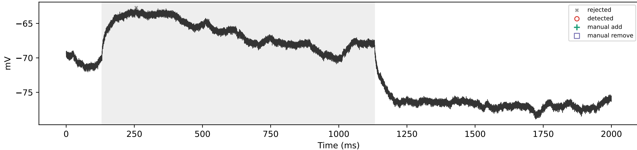
SCA3_07 | 100 pA | total=0, sustained=0
