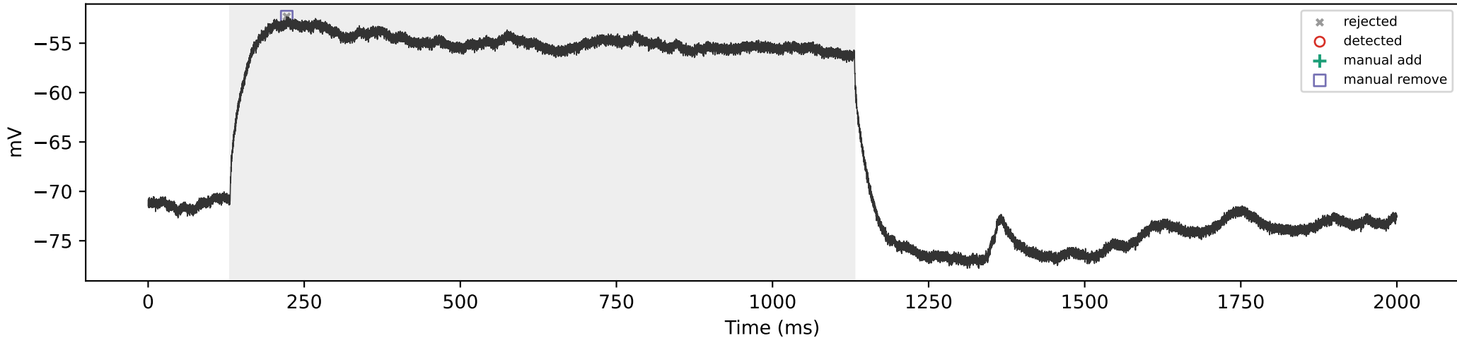
SCA3_07 | 250 pA | total=0, sustained=0
