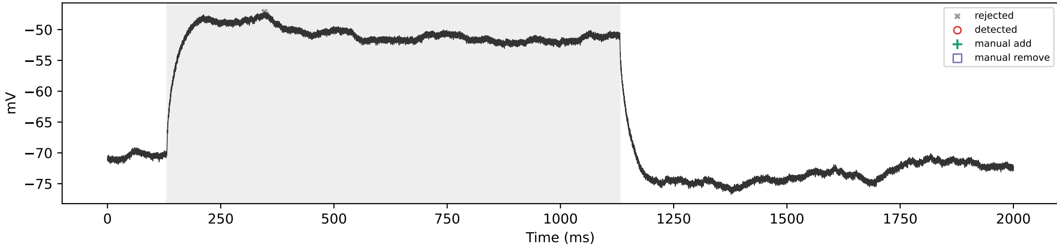
SCA3_07 | 300 pA | total=0, sustained=0
