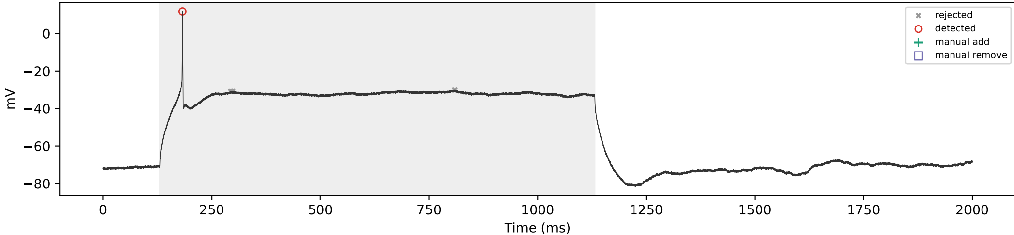
SCA3_07 | 500 pA | total=1, sustained=0
