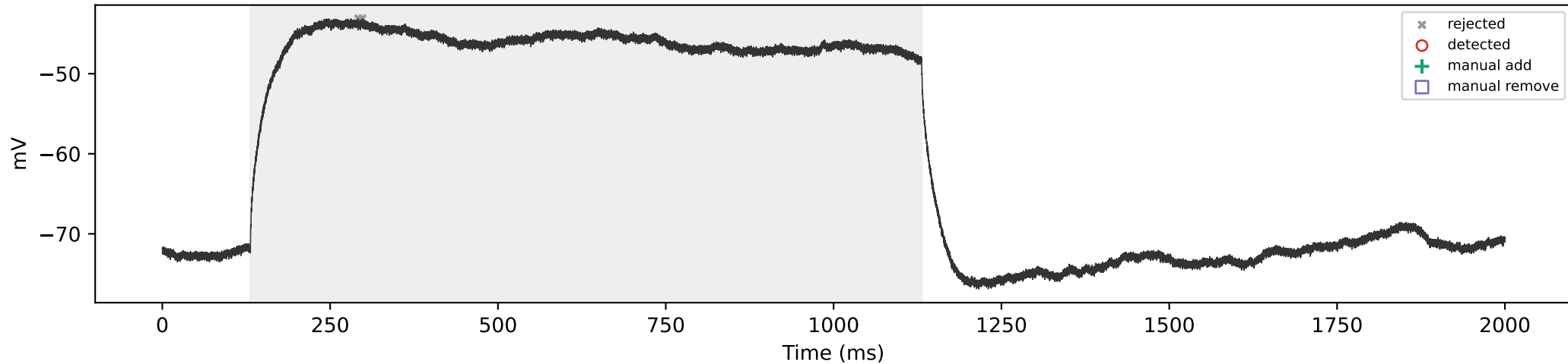
SCA3_07 | 350 pA | total=0, sustained=0
