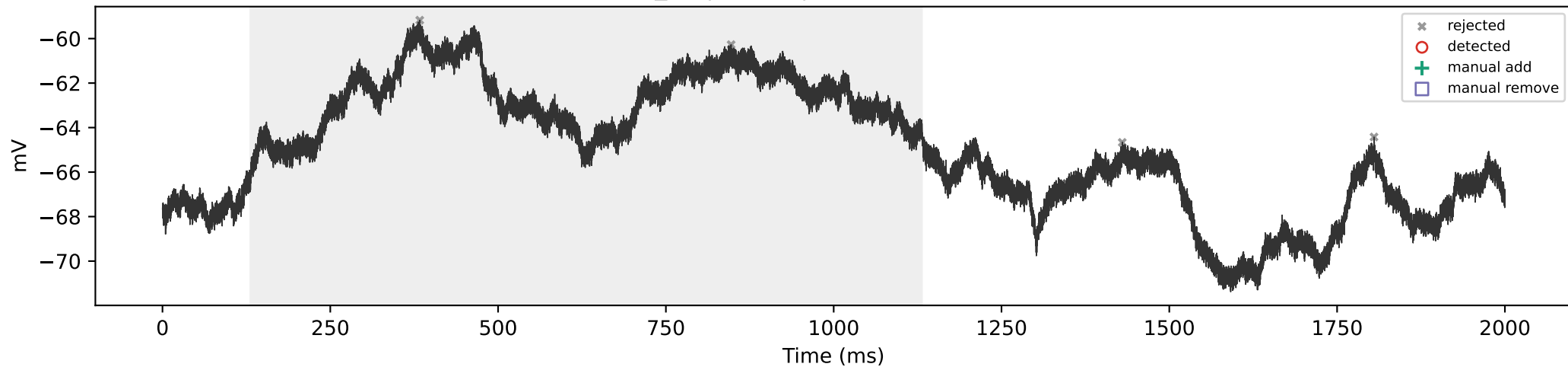
SCA3_07 | 50 pA | total=0, sustained=0
