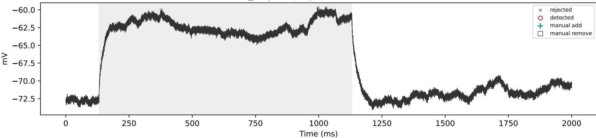
SCA3_07 | 150 pA | total=0, sustained=0
