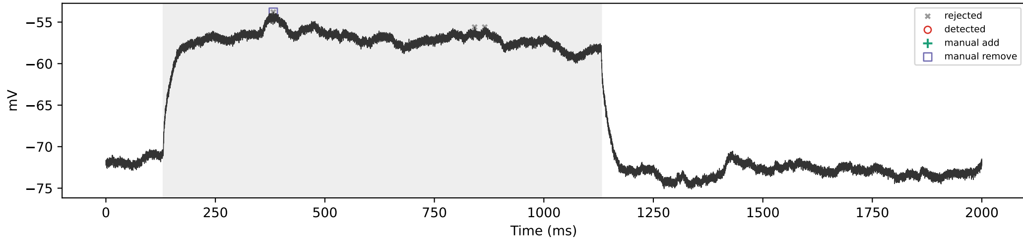
SCA3_07 | 200 pA | total=0, sustained=0
