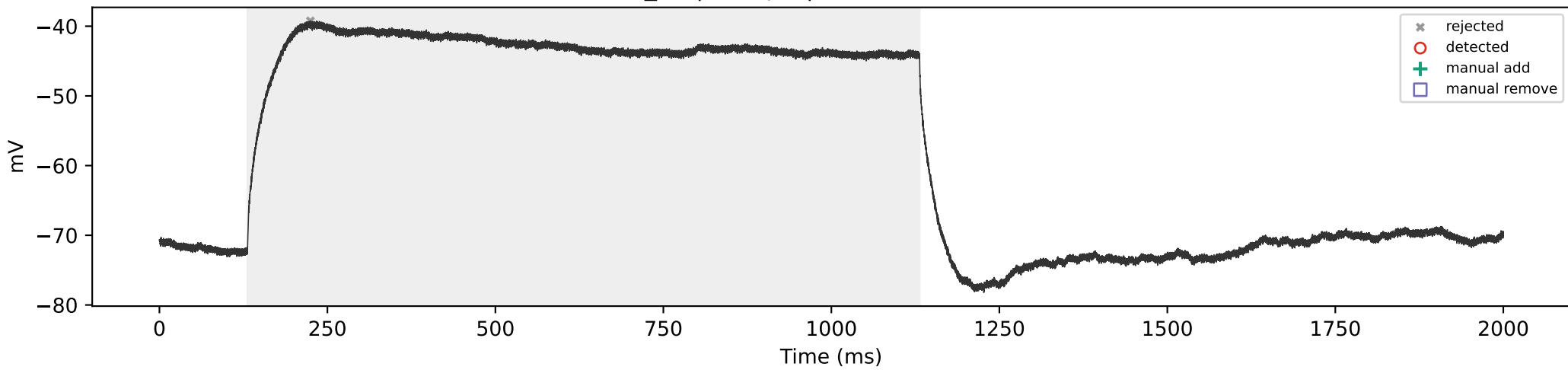
SCA3_07 | 400 pA | total=0, sustained=0
