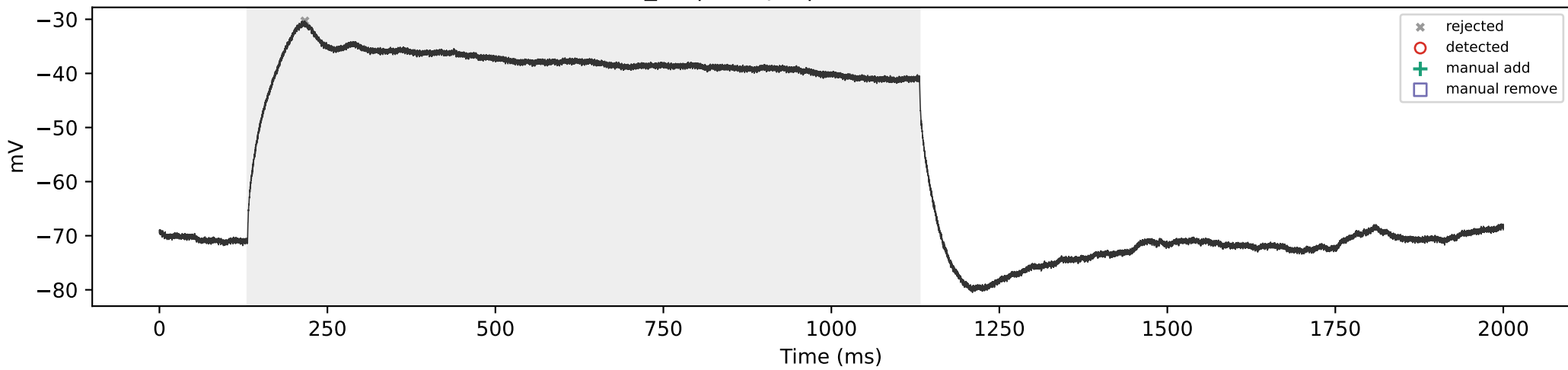
SCA3_07 | 450 pA | total=0, sustained=0
