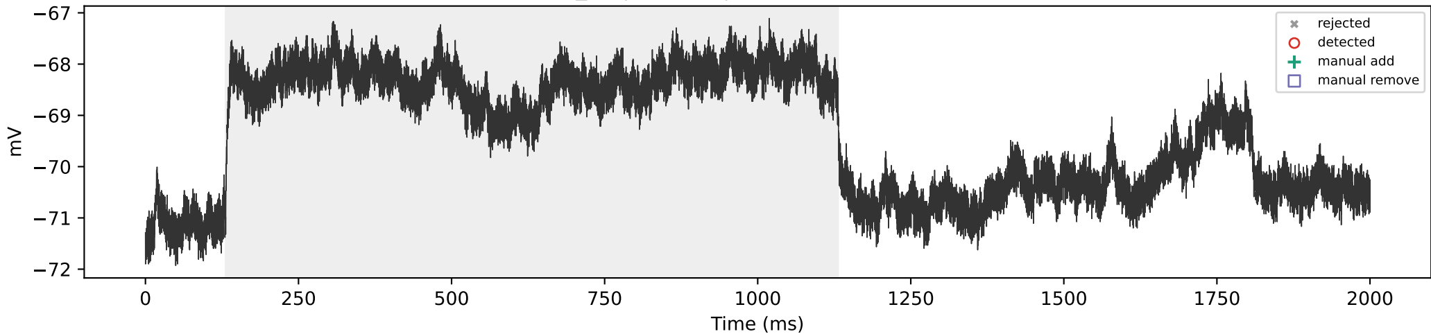
WT_05 | 100 pA | total=0, sustained=0
