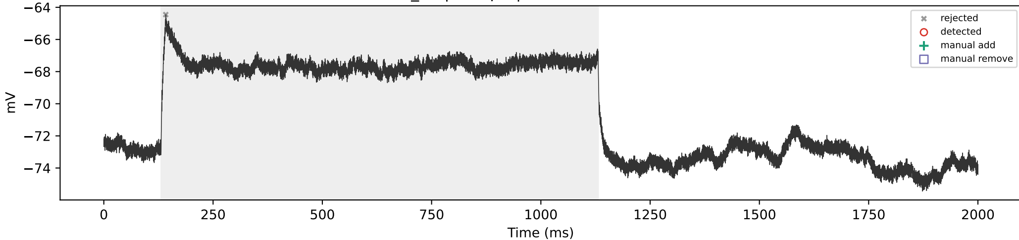
WT_05 | 200 pA | total=0, sustained=0
