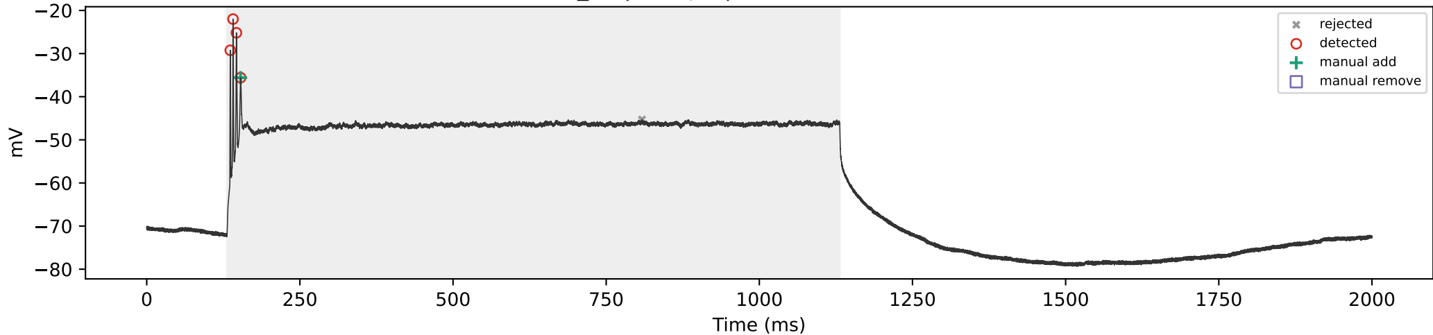
WT_05 | 600 pA | total=4, sustained=4
