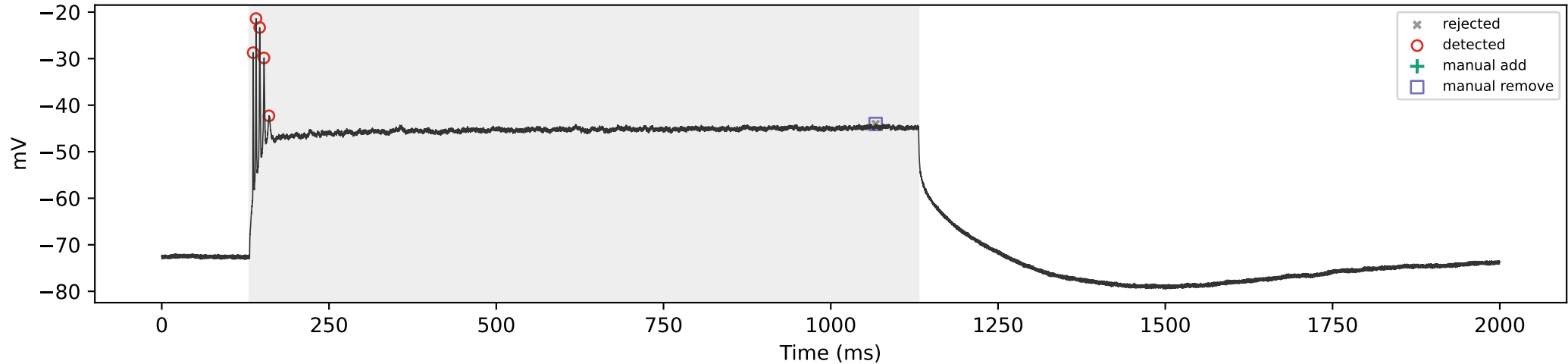
WT_05 | 650 pA | total=5, sustained=5
