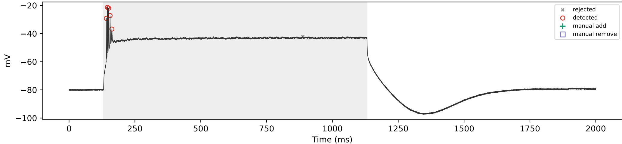
WT_05 | 850 pA | total=5, sustained=5
