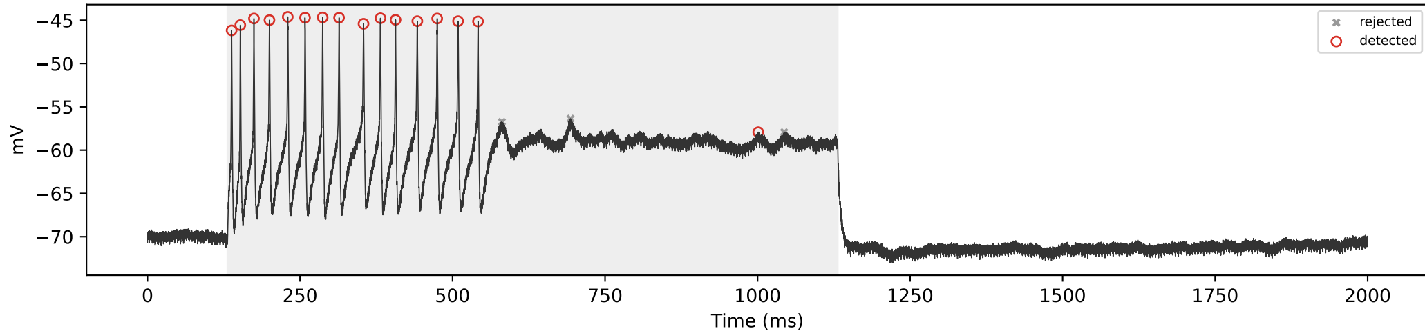
SCA3_02 | 250 pA | total=16, sustained=15
