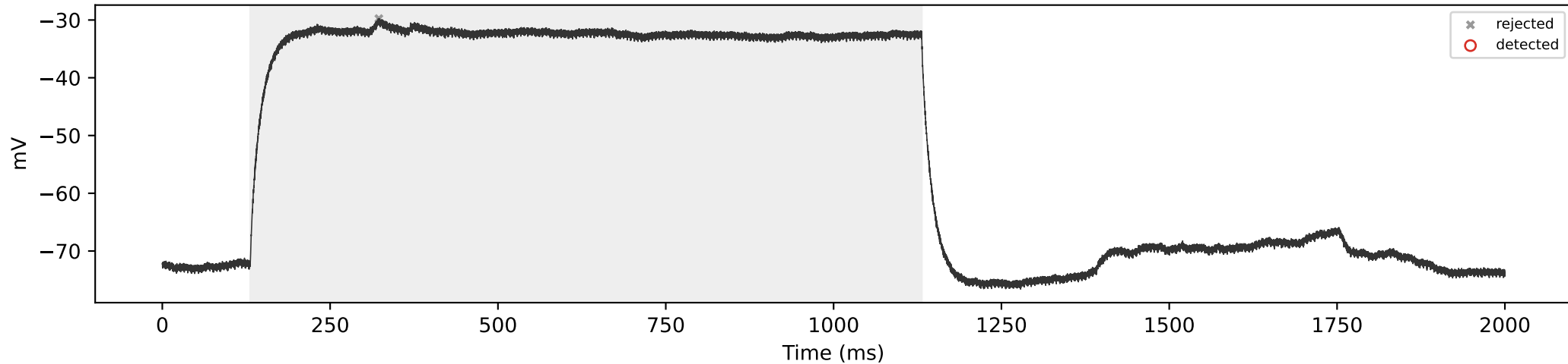
SCA3_03 | 300 pA | total=0, sustained=0
