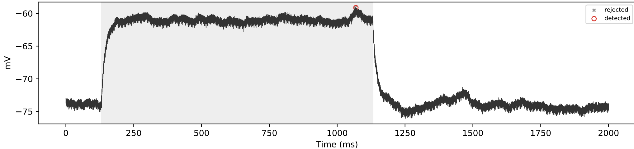
SCA3_03 | 100 pA | total=1, sustained=0
