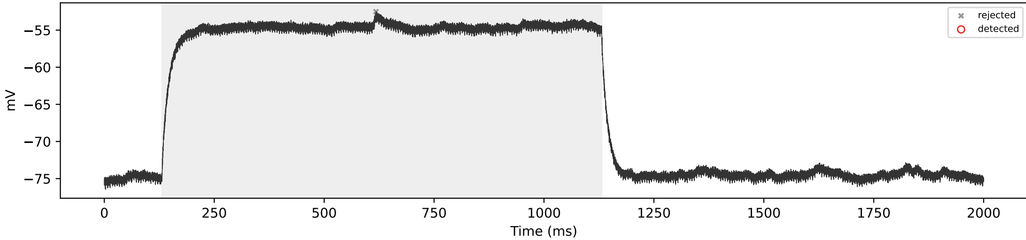
SCA3_03 | 150 pA | total=0, sustained=0
