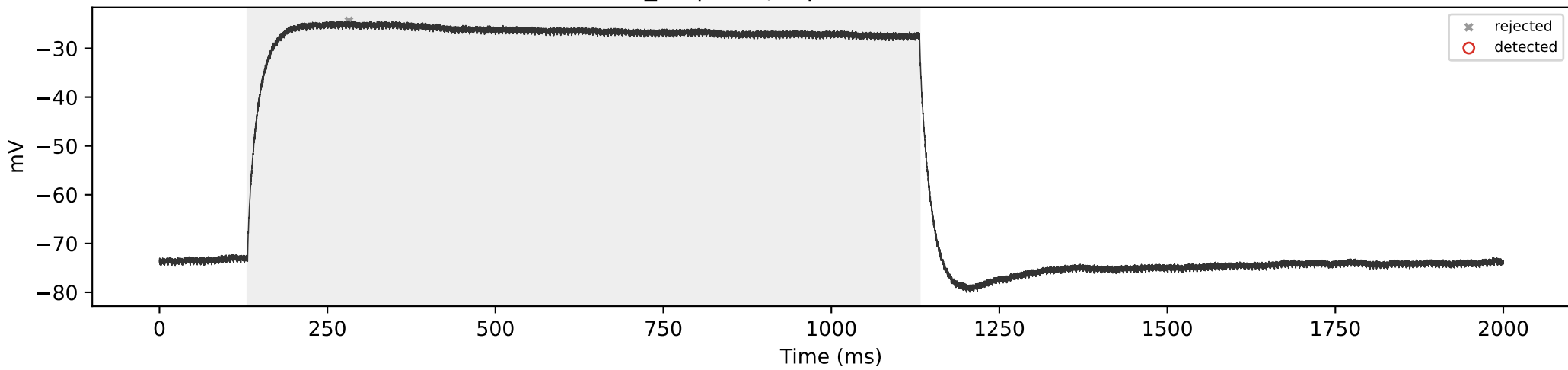
SCA3_03 | 350 pA | total=0, sustained=0
