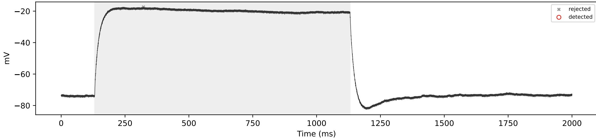
SCA3_03 | 400 pA | total=0, sustained=0
