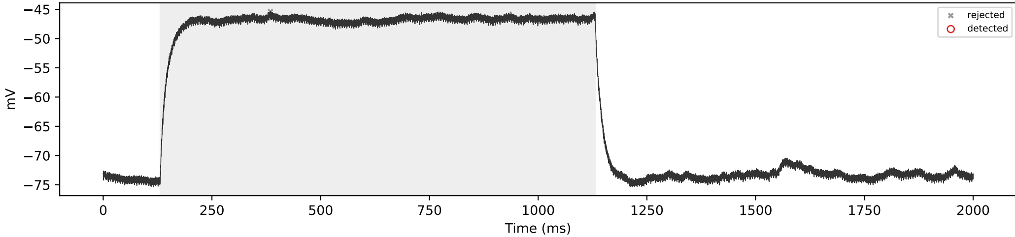
SCA3_03 | 200 pA | total=0, sustained=0
