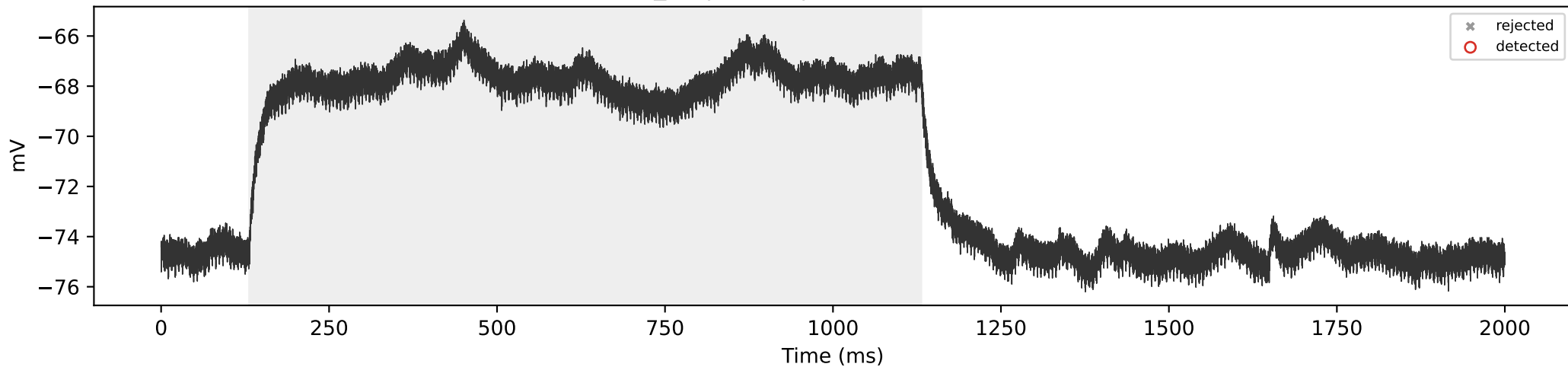
SCA3_03 | 50 pA | total=0, sustained=0
