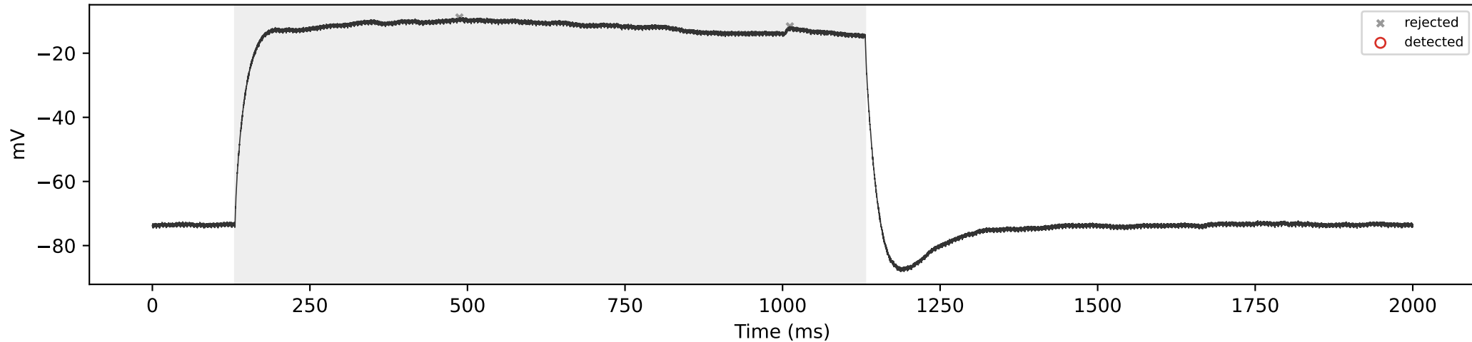
SCA3_03 | 450 pA | total=0, sustained=0
