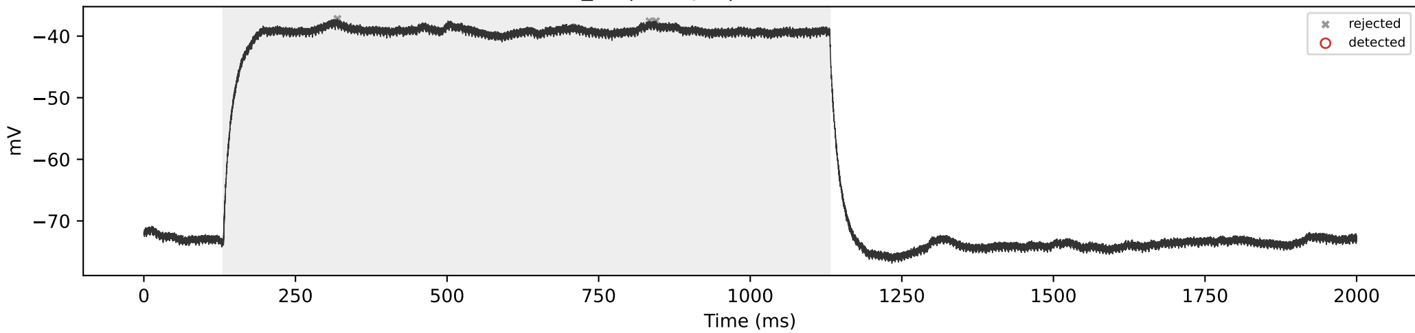
SCA3_03 | 250 pA | total=0, sustained=0
