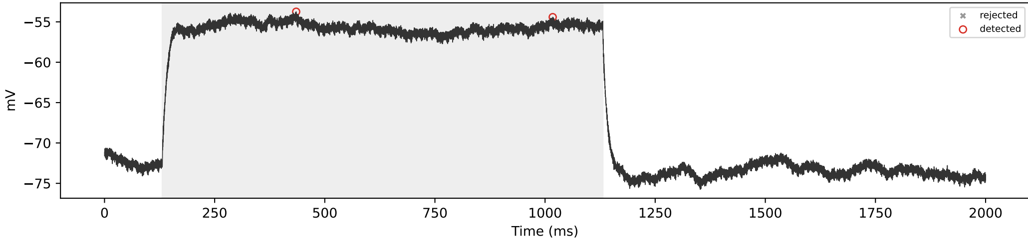
SCA3_05 | 250 pA | total=2, sustained=0
