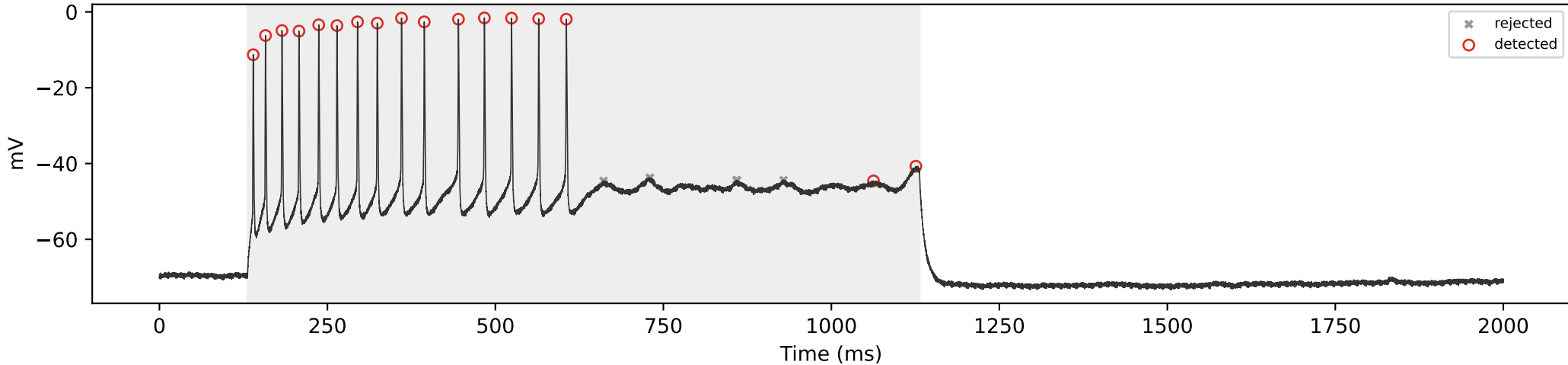
SCA3_05 | 400 pA | total=17, sustained=17
