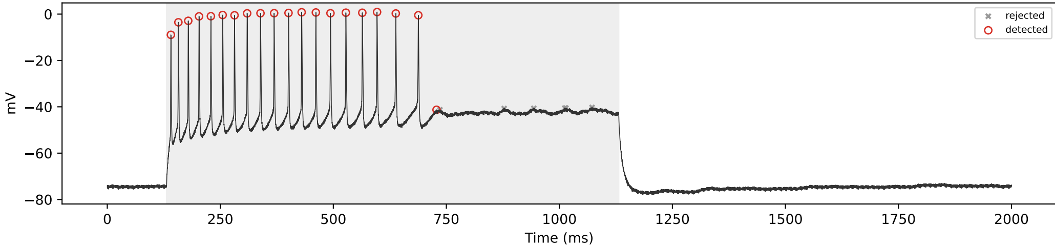
SCA3_05 | 550 pA | total=20, sustained=20
