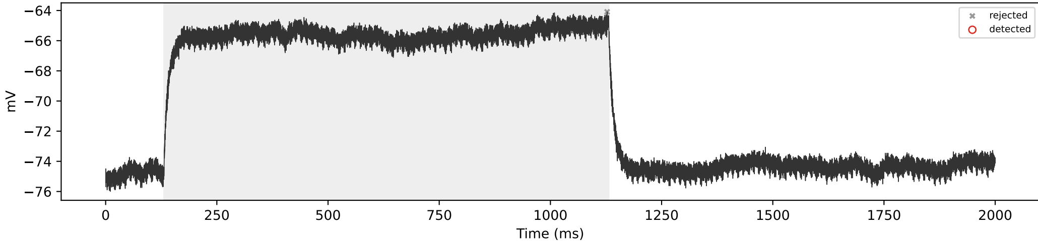
SCA3_05 | 150 pA | total=0, sustained=0
