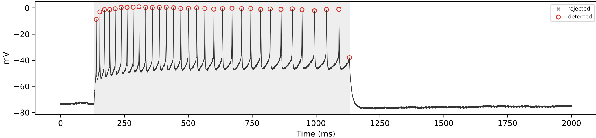
SCA3_05 | 600 pA | total=31, sustained=31
