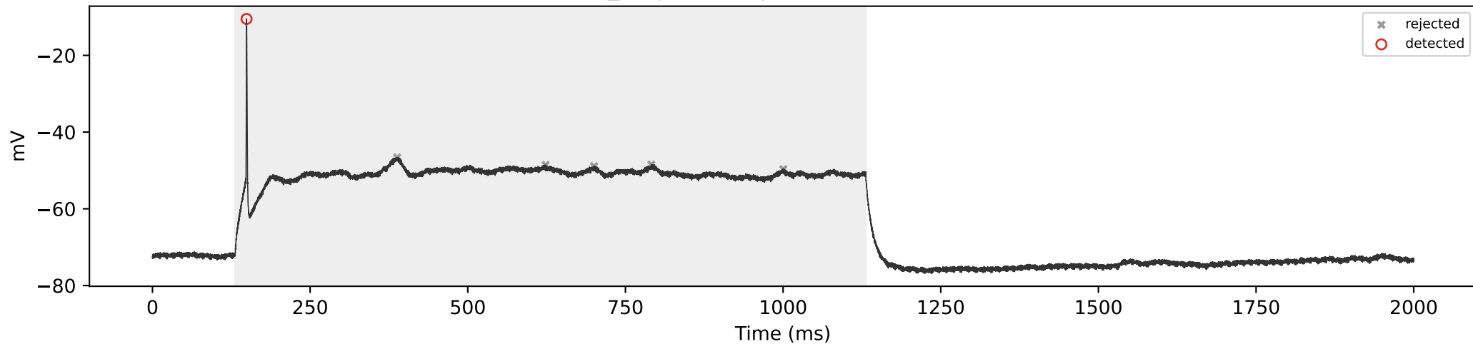
SCA3_05 | 300 pA | total=1, sustained=0
