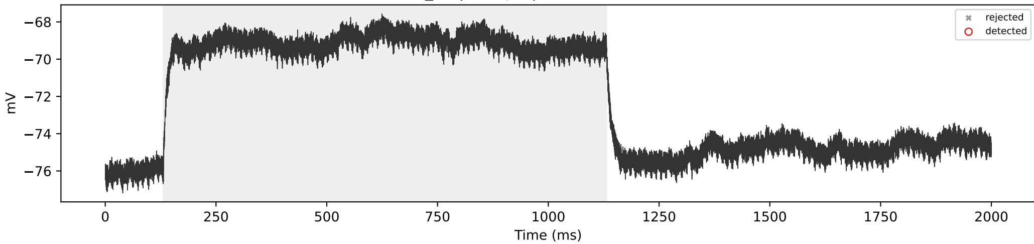
SCA3_05 | 100 pA | total=0, sustained=0
