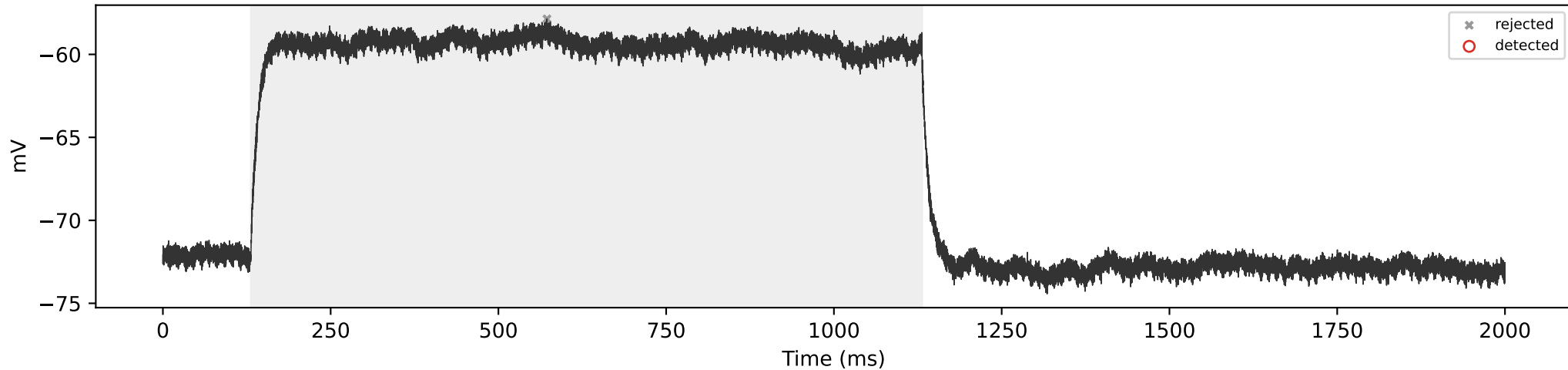
SCA3_05 | 200 pA | total=0, sustained=0
