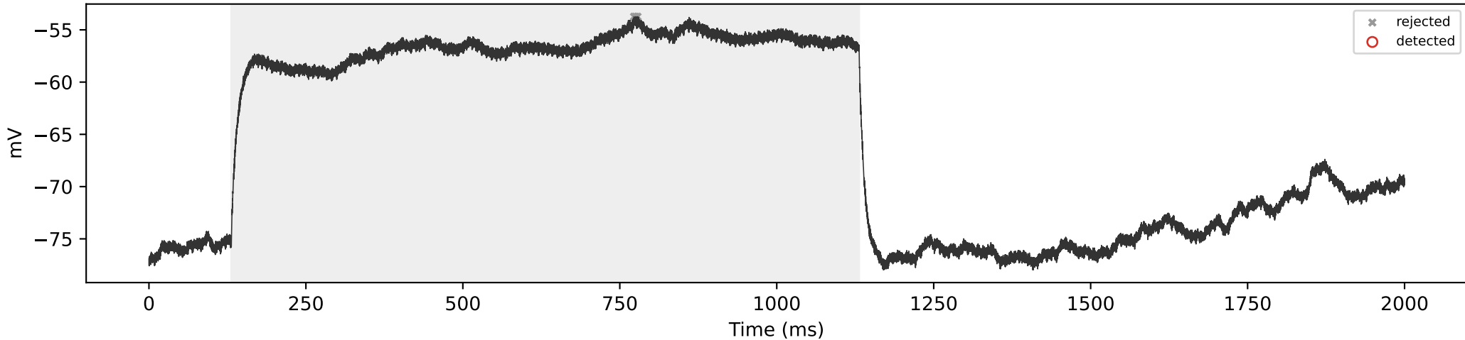
SCA3_06 | 250 pA | total=0, sustained=0
