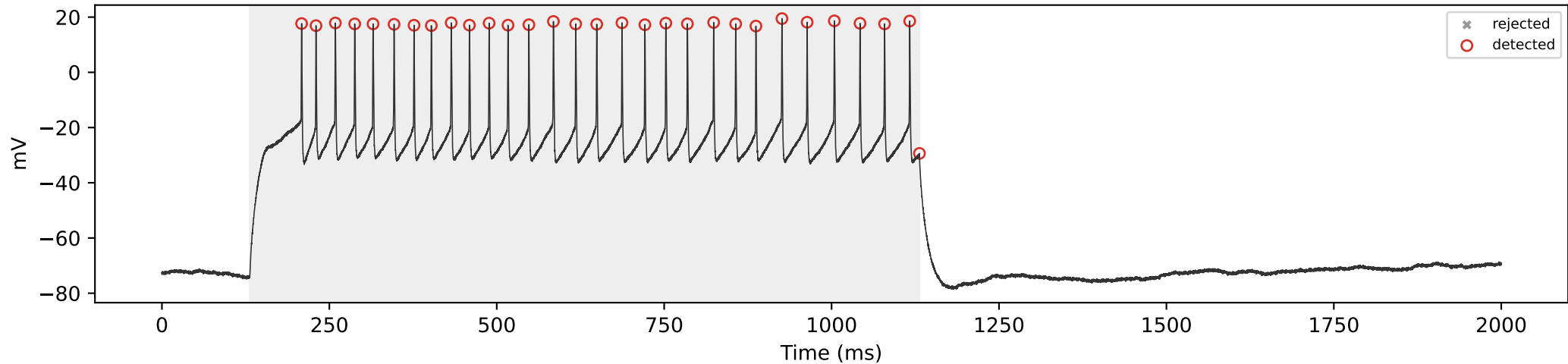
SCA3_06 | 550 pA | total=29, sustained=29
