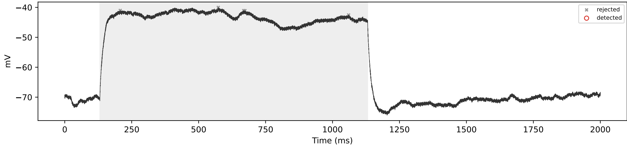
SCA3_06 | 300 pA | total=0, sustained=0
