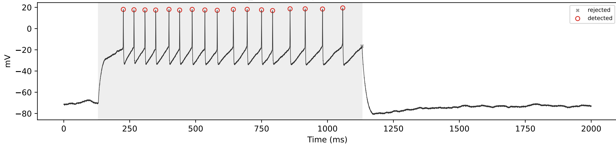
SCA3_06 | 500 pA | total=17, sustained=17
