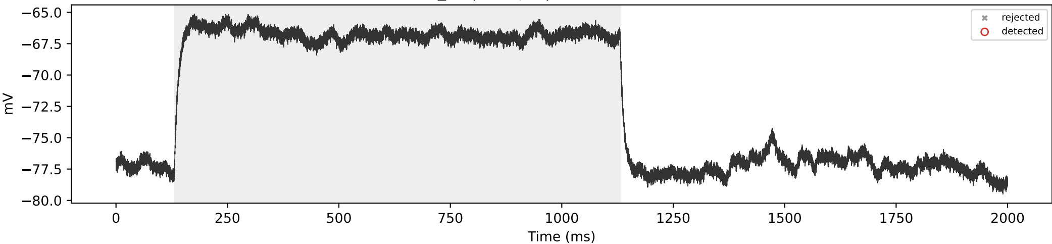
SCA3_06 | 150 pA | total=0, sustained=0
