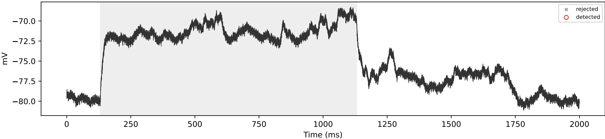
SCA3_06 | 100 pA | total=0, sustained=0
