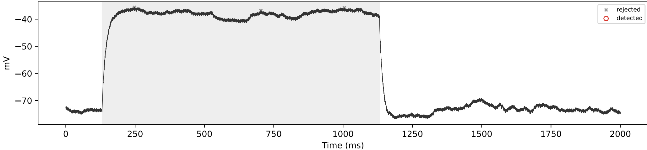
SCA3_06 | 350 pA | total=0, sustained=0
