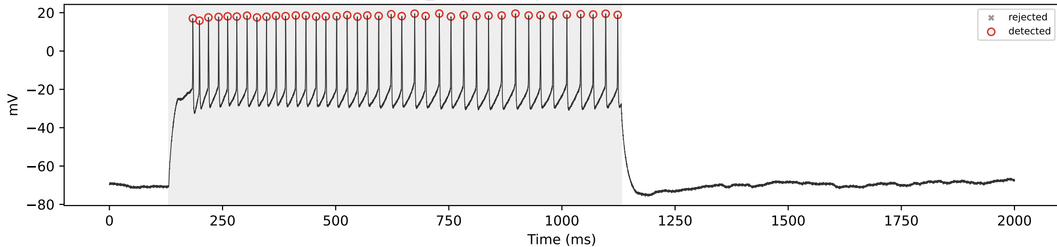
SCA3_06 | 600 pA | total=39, sustained=39
