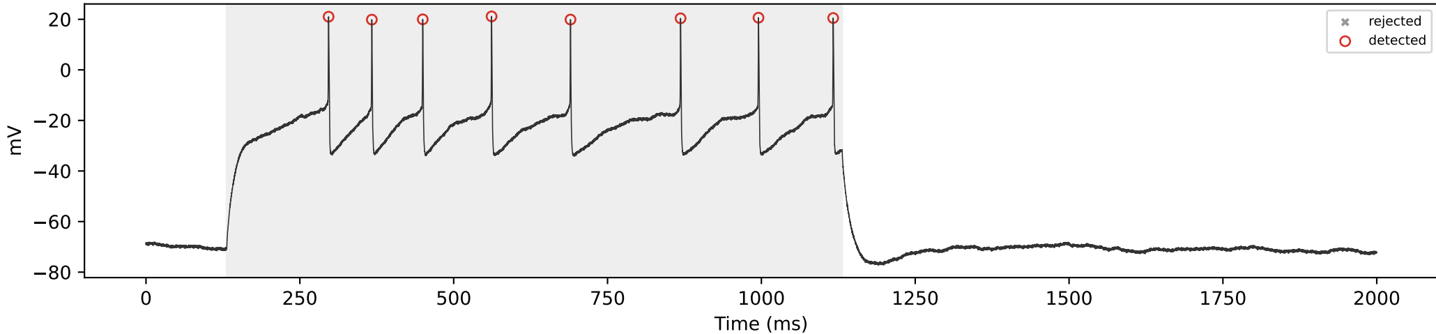
SCA3_06 | 450 pA | total=8, sustained=8
