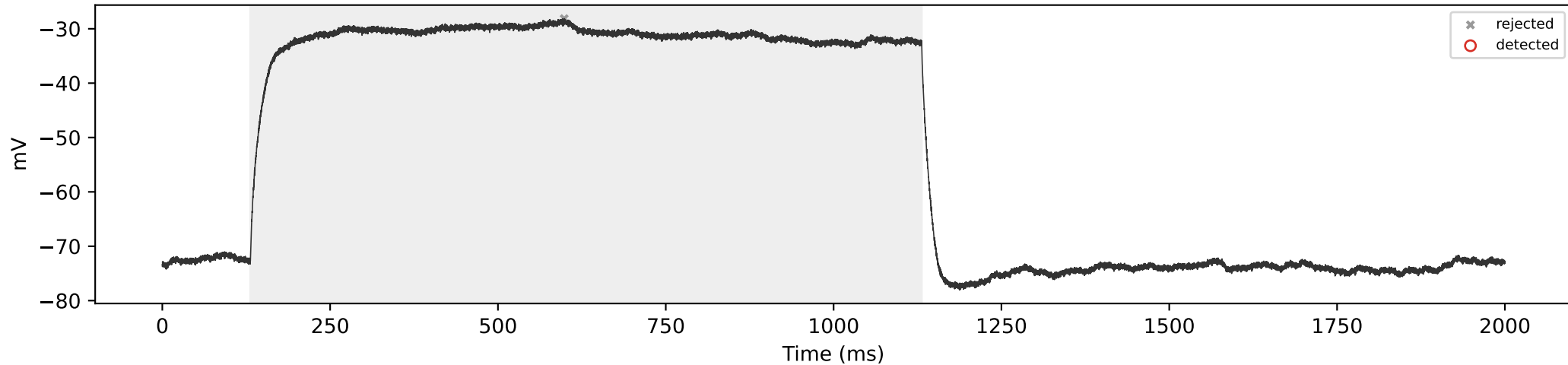
SCA3_06 | 400 pA | total=0, sustained=0
