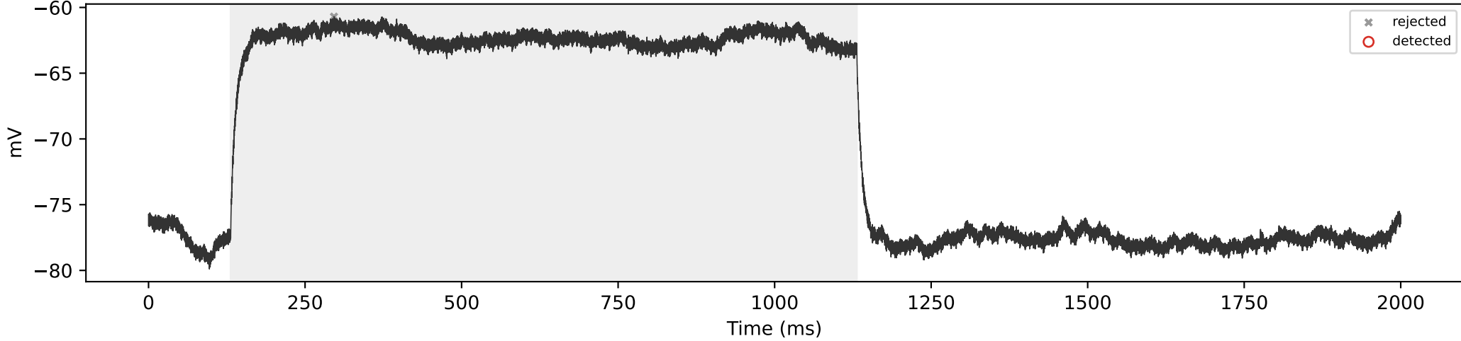
SCA3_06 | 200 pA | total=0, sustained=0
