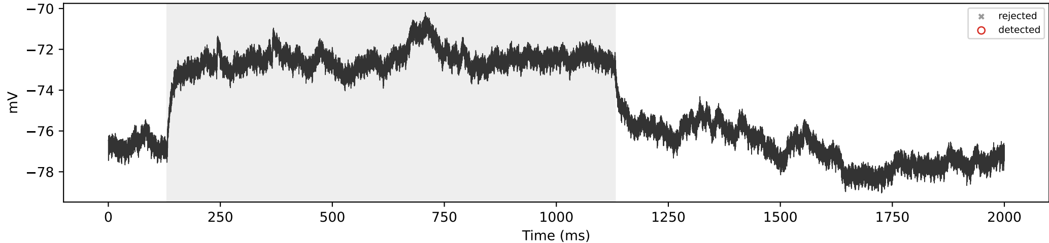
SCA3_06 | 50 pA | total=0, sustained=0
