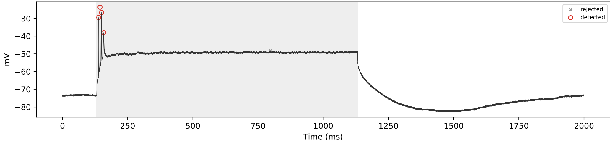
WT_05 | 500 pA | total=4, sustained=4
