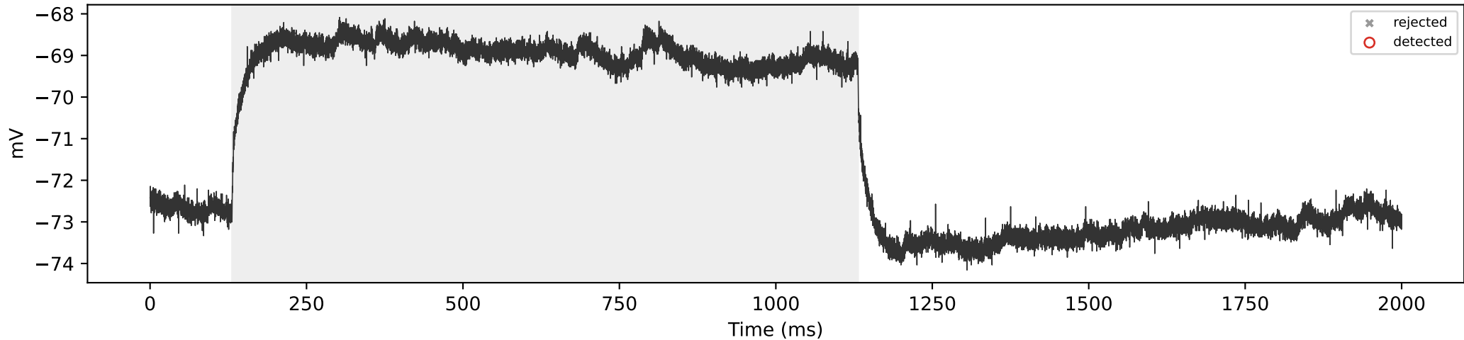
WT_12 | 100 pA | total=0, sustained=0
