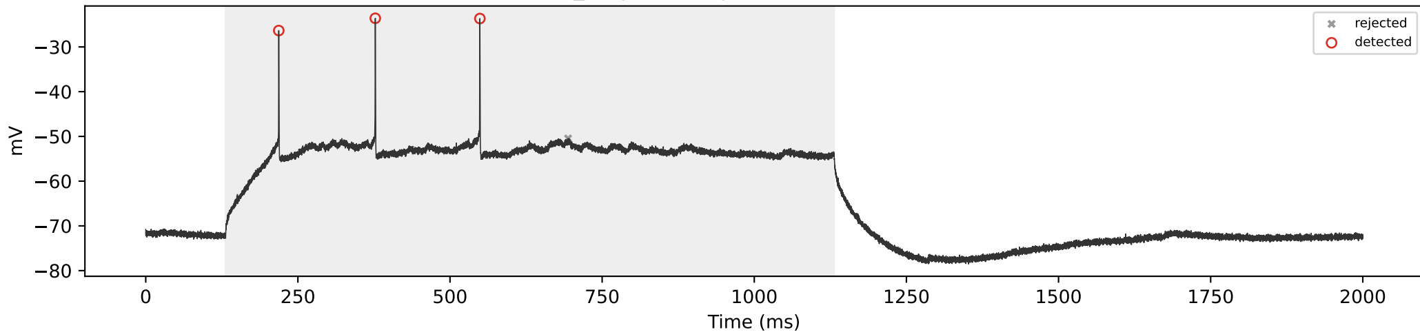
WT_15 | 200 pA | total=3, sustained=3
