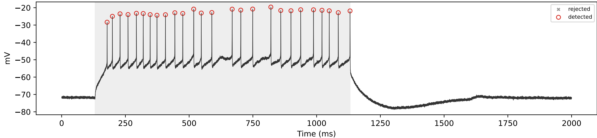
WT_15 | 250 pA | total=25, sustained=25
