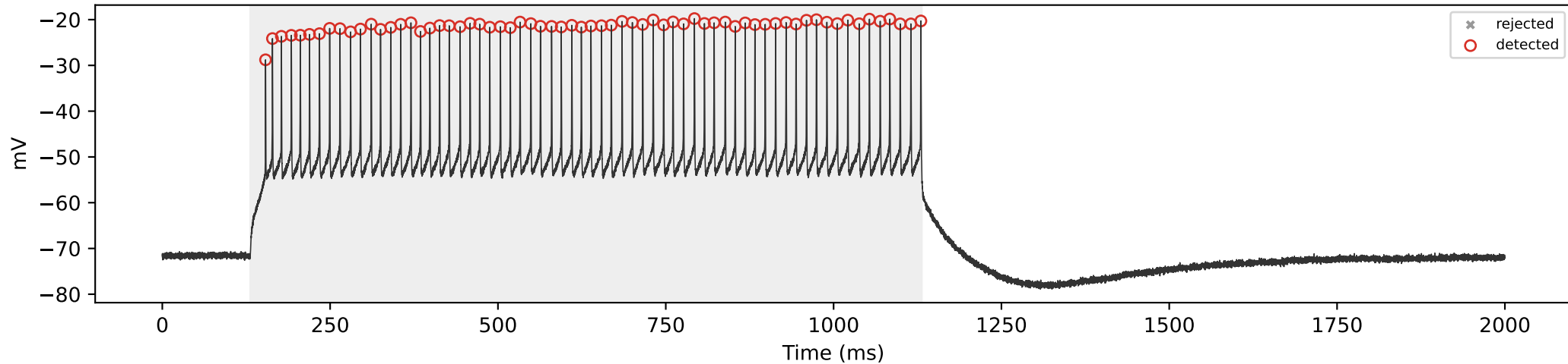
WT_15 | 350 pA | total=65, sustained=65
