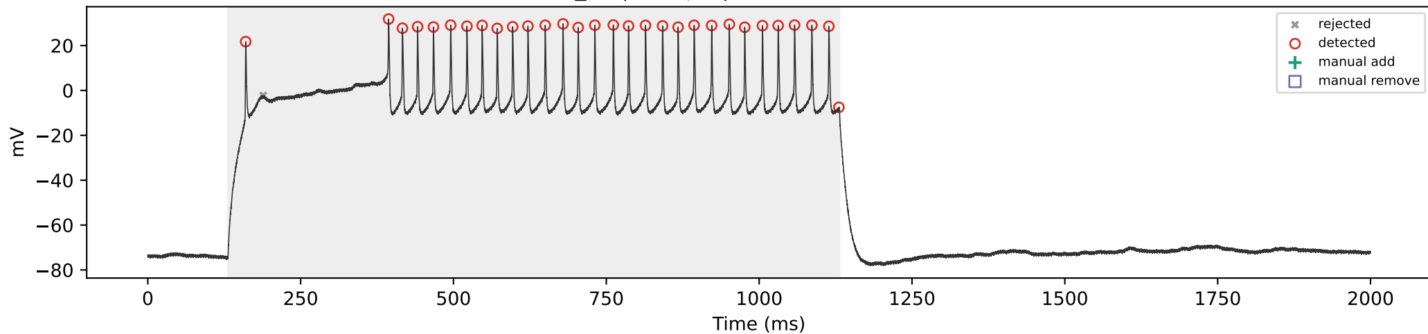
SCA3_01 | 550 pA | total=29, sustained=28
