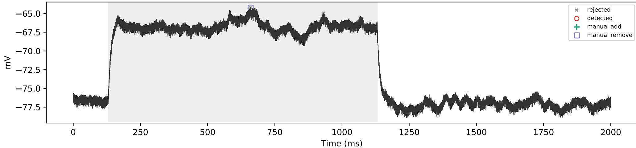
SCA3_01 | 100 pA | total=0, sustained=0
