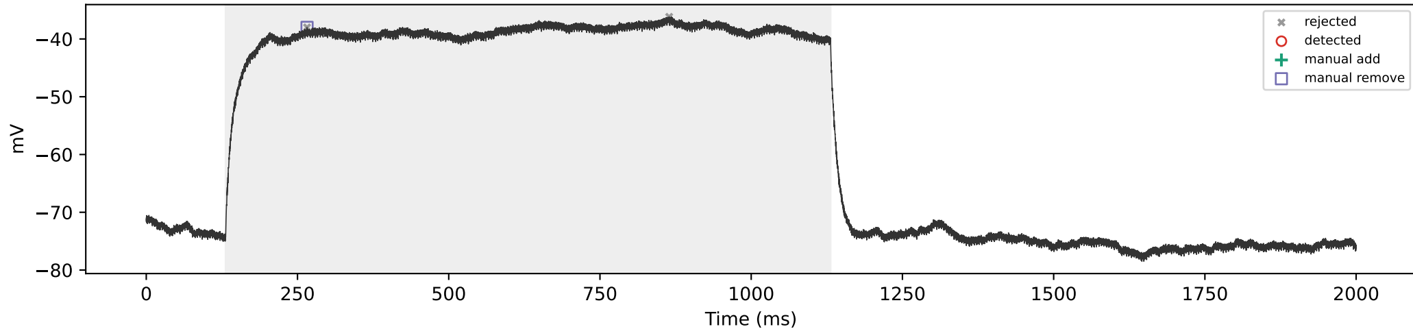
SCA3_01 | 300 pA | total=0, sustained=0
