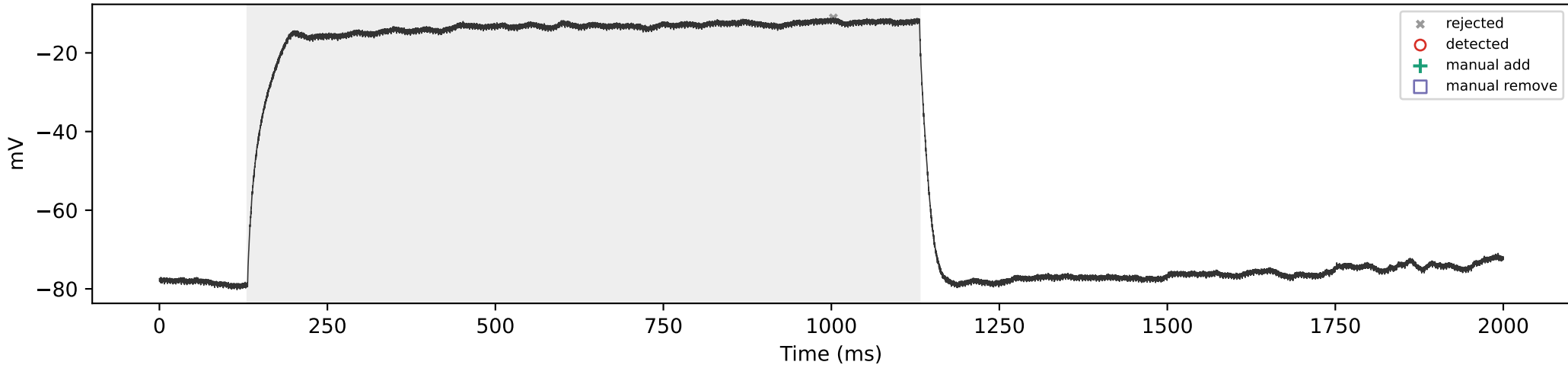
SCA3_01 | 450 pA | total=0, sustained=0
