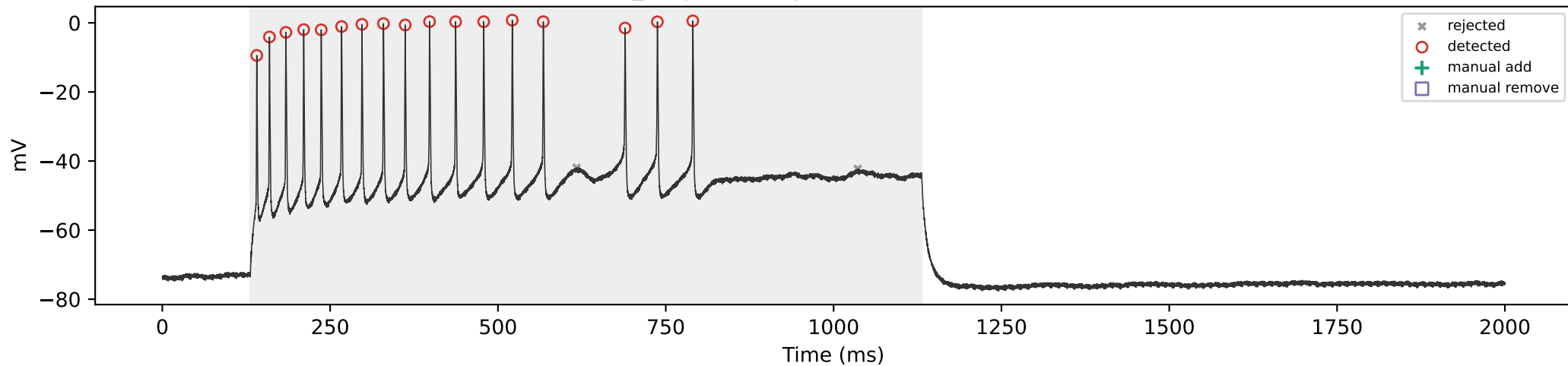
SCA3_05 | 500 pA | total=17, sustained=17
