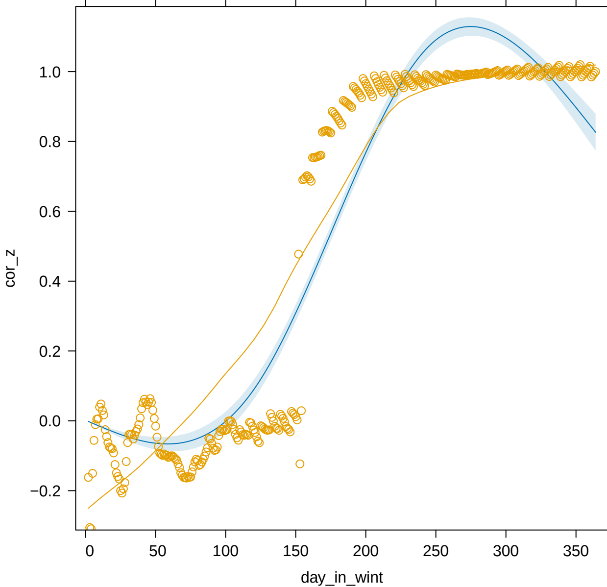
day_in_wint predictor effect plot
